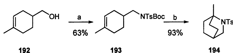
Scheme 2.50. a) \text{PPh}_3 , DIAD, \text{TsNHBoc} , THF, 0 °C, overnight b) 0.5 eq. \text{TfOH} , DCM, 20 °C, 48 hrs
