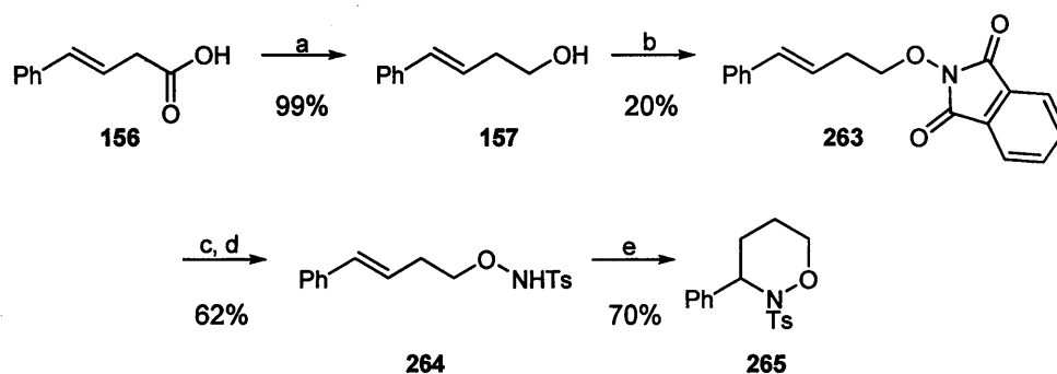
Scheme 2.71. a) \text{LiAlH}_4 , \text{Et}_2\text{O} , 20 °C, 1 hr b) \text{PPh}_3 , DIAD, N -hydroxyphthalimide, THF, 0 °C, overnight c) \text{H}_2\text{NNH}_2 , EtOH, 60 °C, 2 hrs d) p -TsCl, \text{NEt}_3 , DMAP, DCM, -78 °C, overnight e) 0.5 eq. TfOH, DCM, 20 °C, 24 hrs
