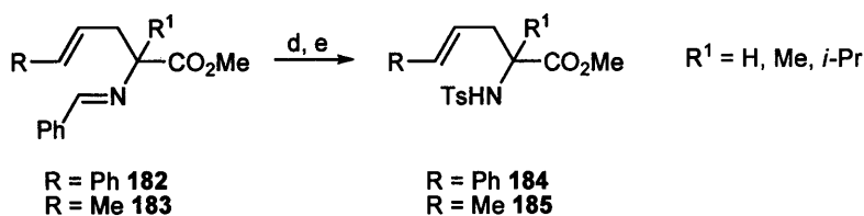
Scheme 2.44. d) 1 M HCl, Et 2 O, 2 hrs e) p -TsCl, NEt 3 , DCM, -78\text{ }^{\circ}\text{C} , overnight
