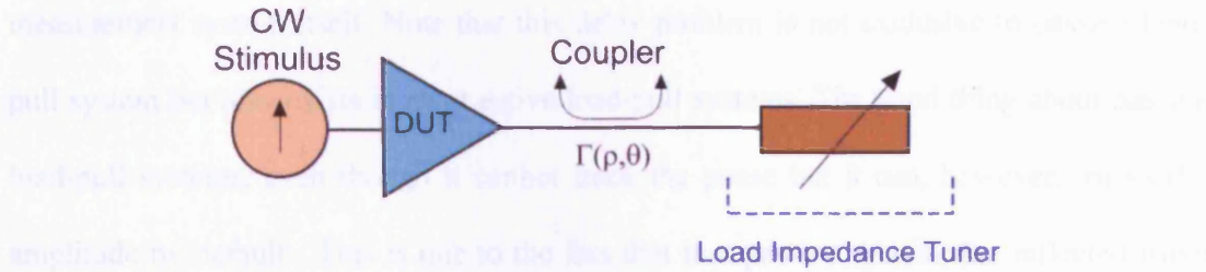
Figure 2.7: Passive load-pull
