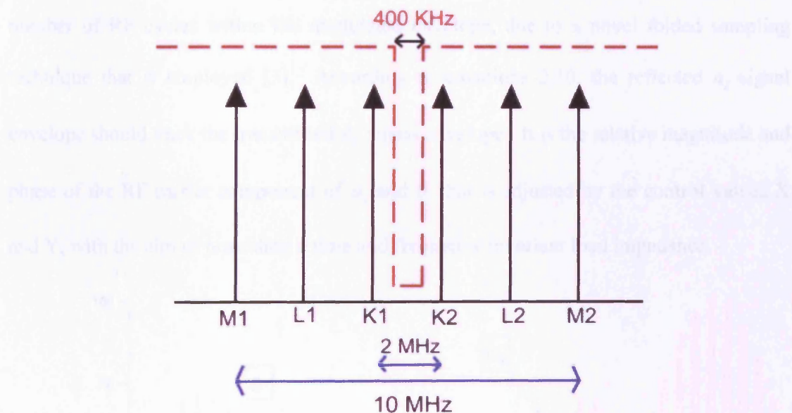
Figure 4.5: Six-tone stimulus signal, showing the spectral mask of digital controller
