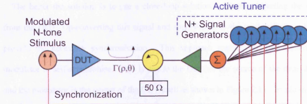
Figure 2.9: Active load-pull multi-tone stimulus with open loop architecture
