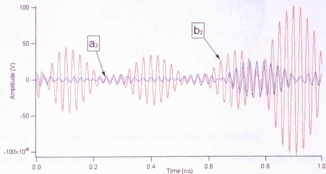
Figure 4.6: Measured waves for transmitted and reflected waves before delay compensation
