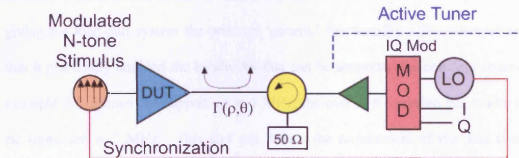
Figure 2.10: Active load-pull multi-tone stimulus with open loop architecture and modulator
