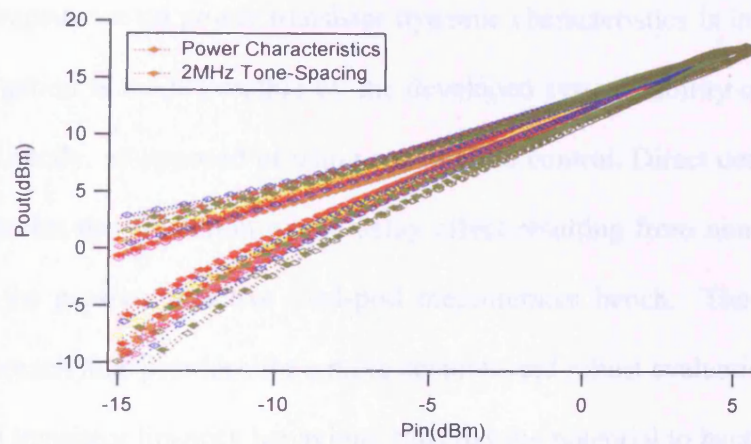
Figure 5.12: Envelope domain representation of dynamic power characteristics at different power levels
