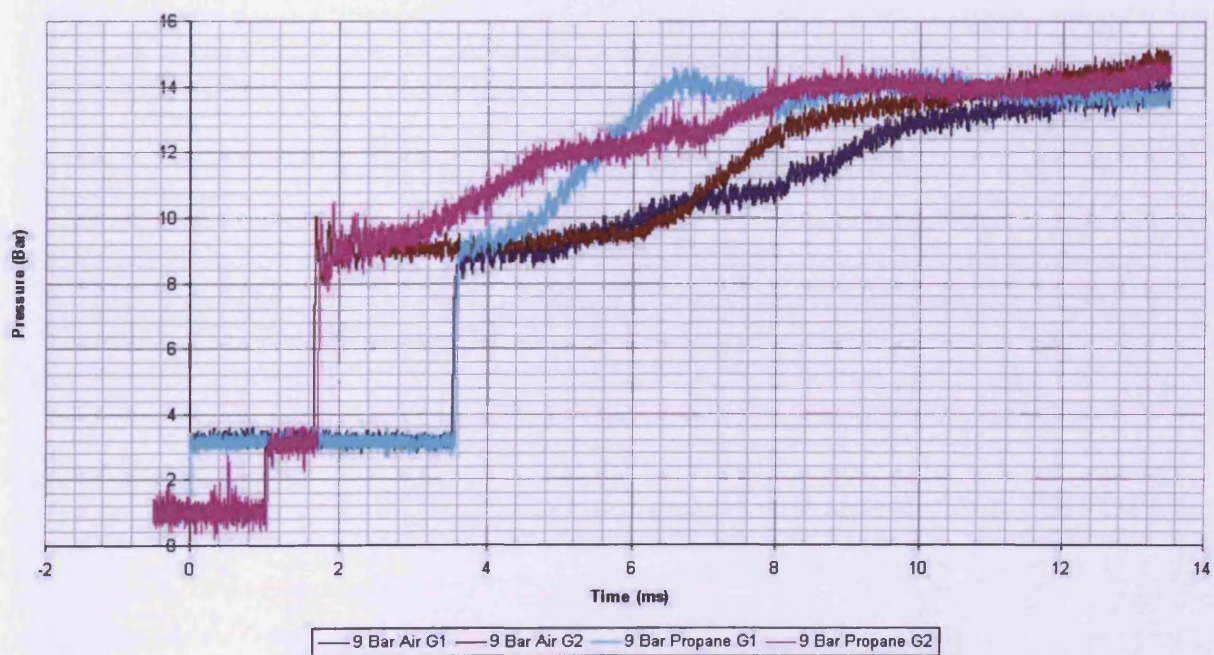
Figure 5.6: Propane Conical Face Results, M=1.70
