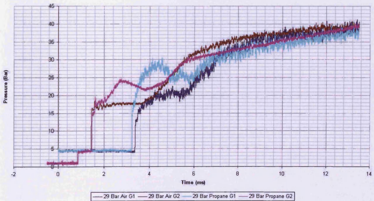
Figure 5.8: Propane Conical Face Results, M=2.00
