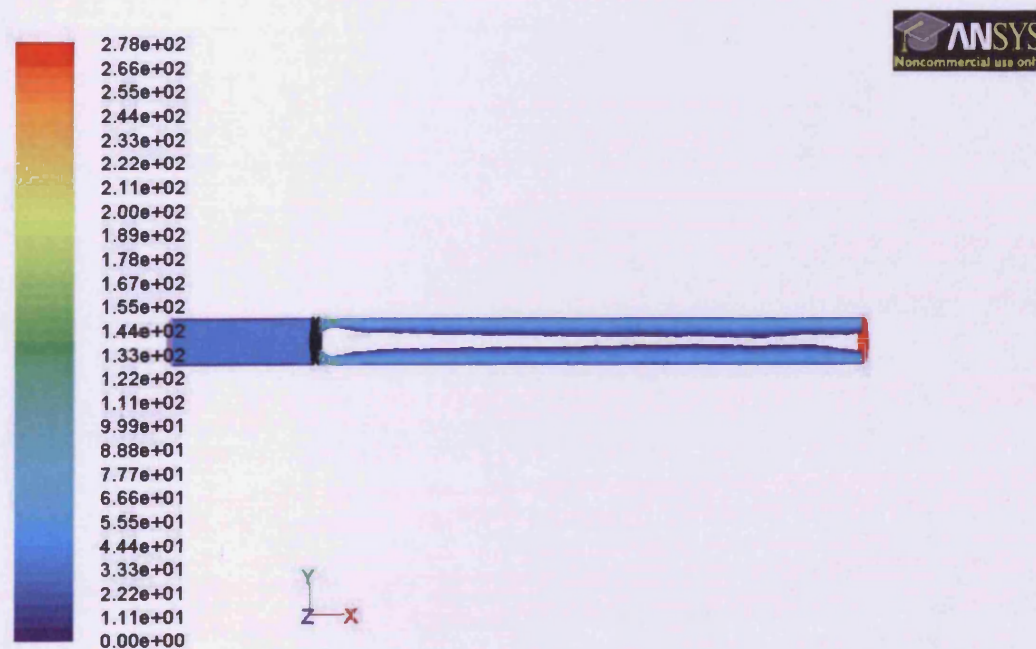
Figure 8.6b: Co-Swirl Mixing at Half Mass Flow Rate to 5% of target
