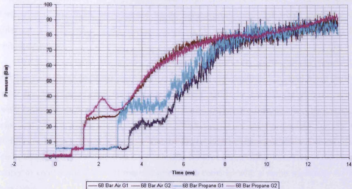
Figure 5.17: Propane Hemispherical Face Results, M=2.23
