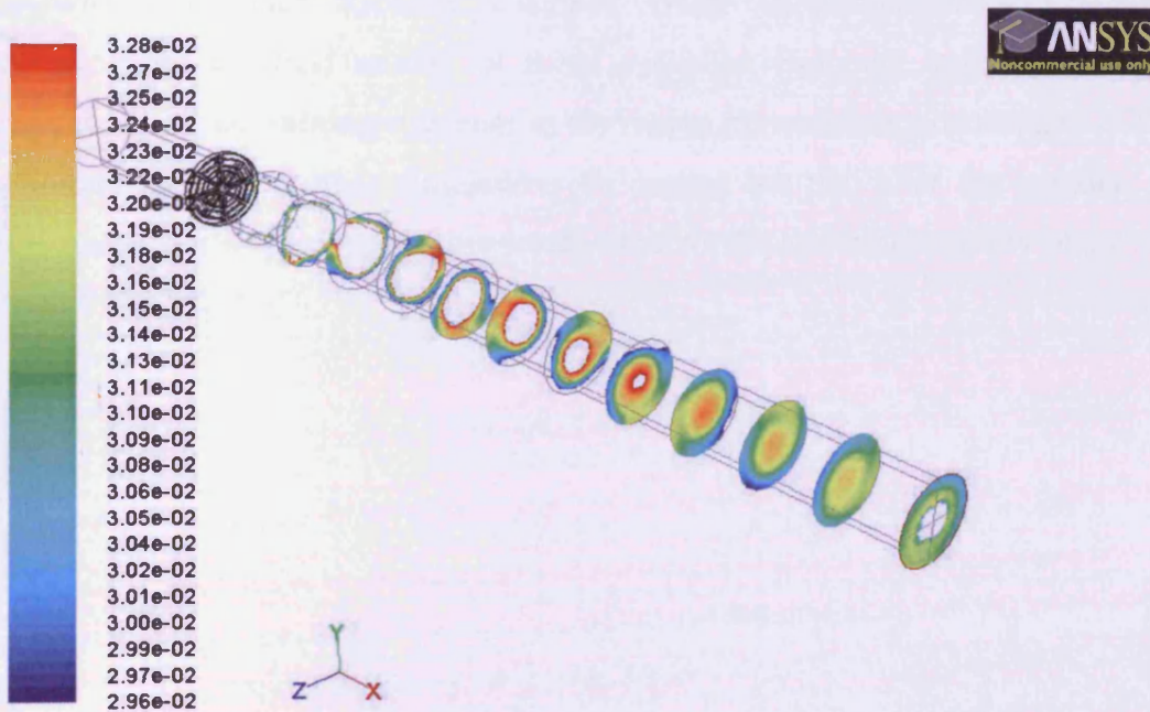
Figure 8.28a: Inner Circumferentially Clamped Bottom Outer Radially Clamped Mixing at Half Mass Flow Rate to 5% of target (front view)
