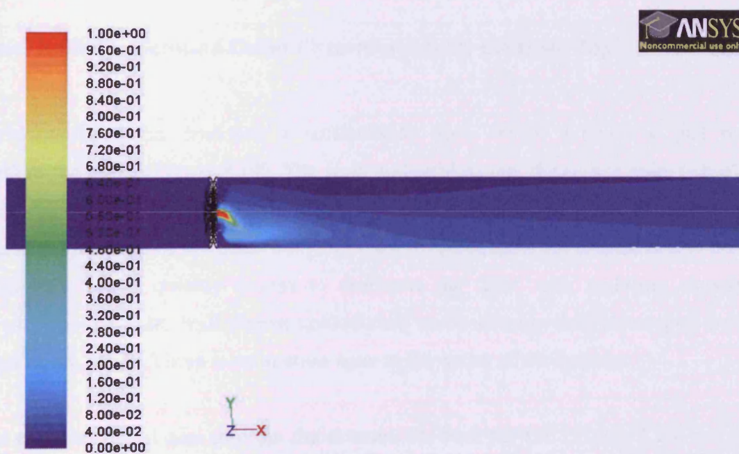
Figure 8.17: Circumferentially Clamped Bottom No Fuel Positive X velocity RSM Model
