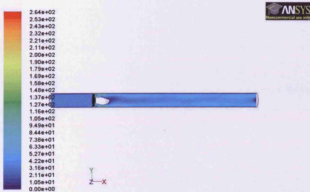
Figure 8.11b: Counter Swirl Mixing at Half Mass Flow Rate to 10% of target (cross sectional views)
