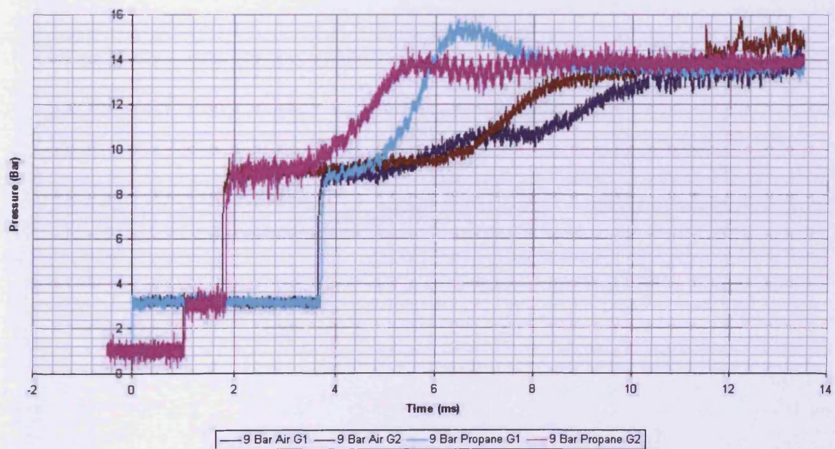
Figure 5.13: Propane Hemispherical Face Results, M=1.70
