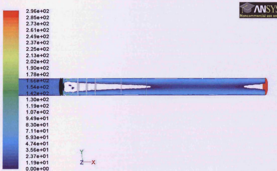
Figure 8.3: Co-Swirl Pathlines
