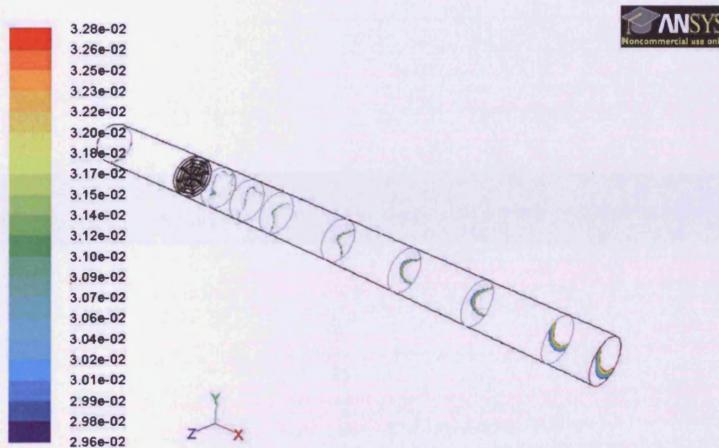
Figure 8.16a: Circumferentially Clamped Bottom Mixing at Half Mass Flow Rate to 10% of target
