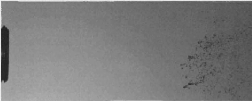
Figure 6.22m: Pulsed Flow Breakup, z=40\text{mm} , Frame 13
