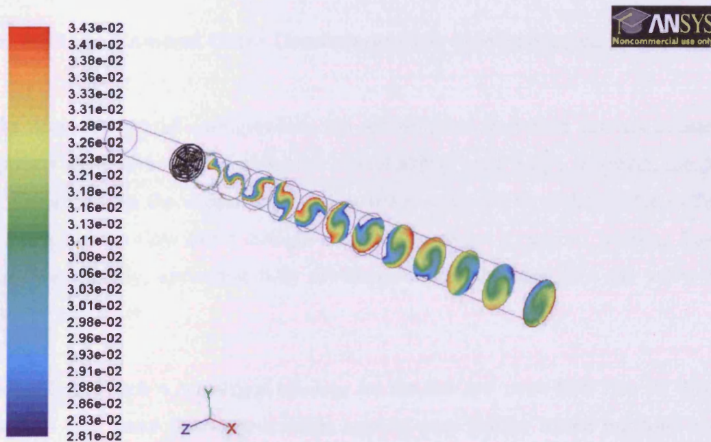
Figure 8.20b: Inner Radially Clamped Outer Circumferentially Clamped Top Mixing at Full Mass Flow Rate to 5% of target
