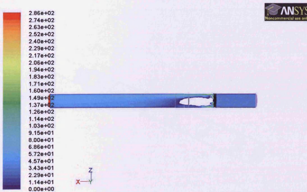
Figure 8.14a: Circumferentially Clamped Bottom No Fuel Positive X velocity (front view)
