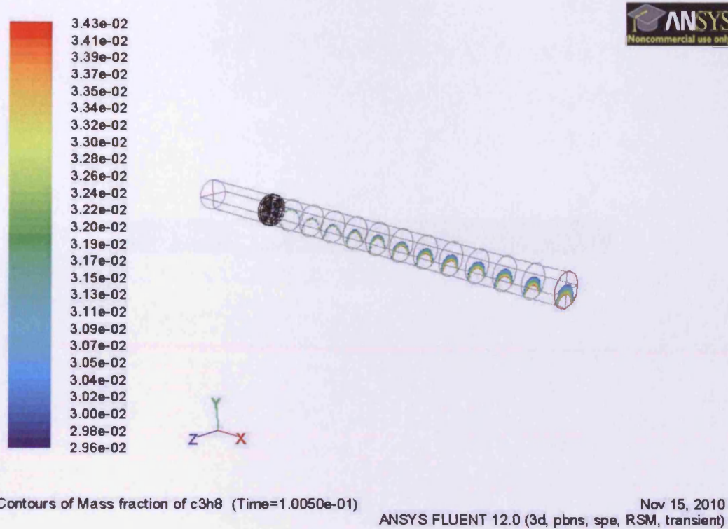
Figure 8.18b: Circumferentially Clamped Bottom Mixing at Half Mass Flow Rate RSM Model to 10% of target
