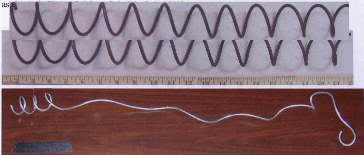
Figure 2.6: Damage Caused to a Schelkin Spiral [11]
