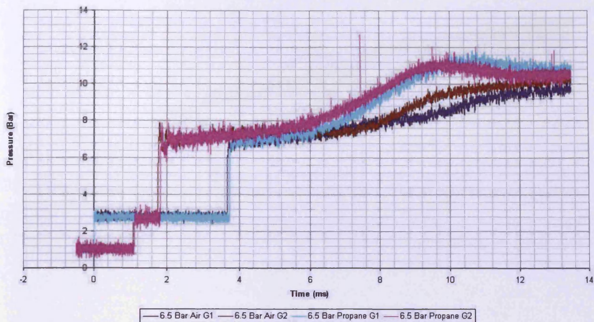
Figure 5.5: Propane Conical Face Results, M=1.60
