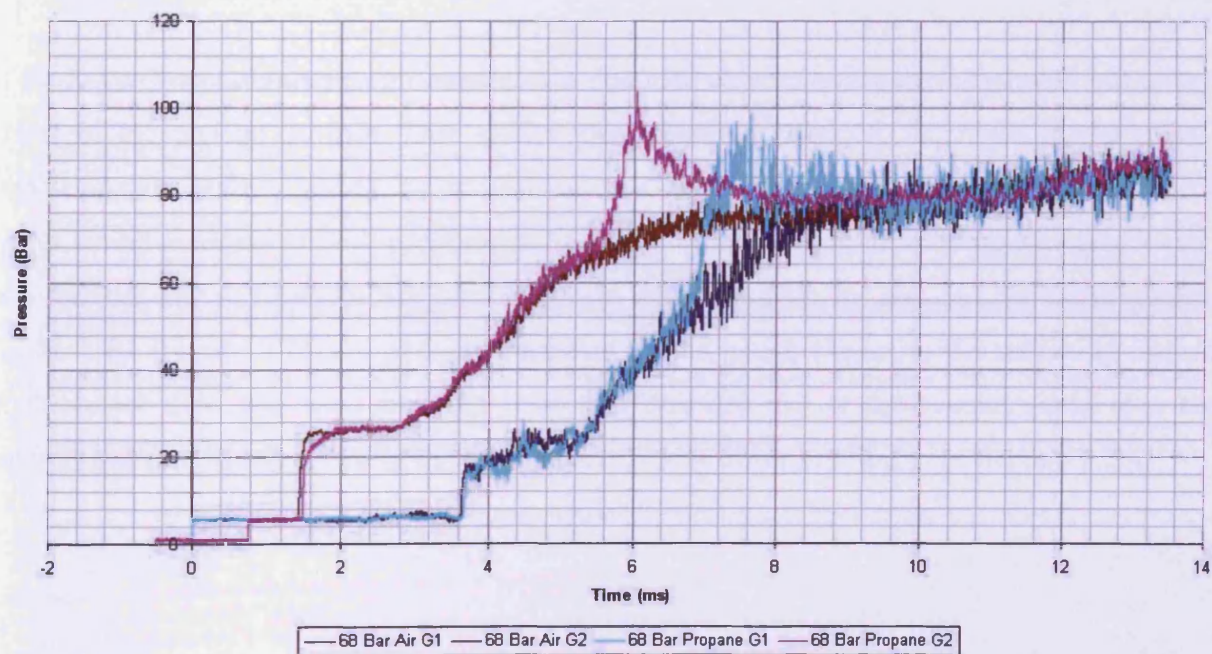
Figure 5.4: Propane Flat Face Results, M=2.23
