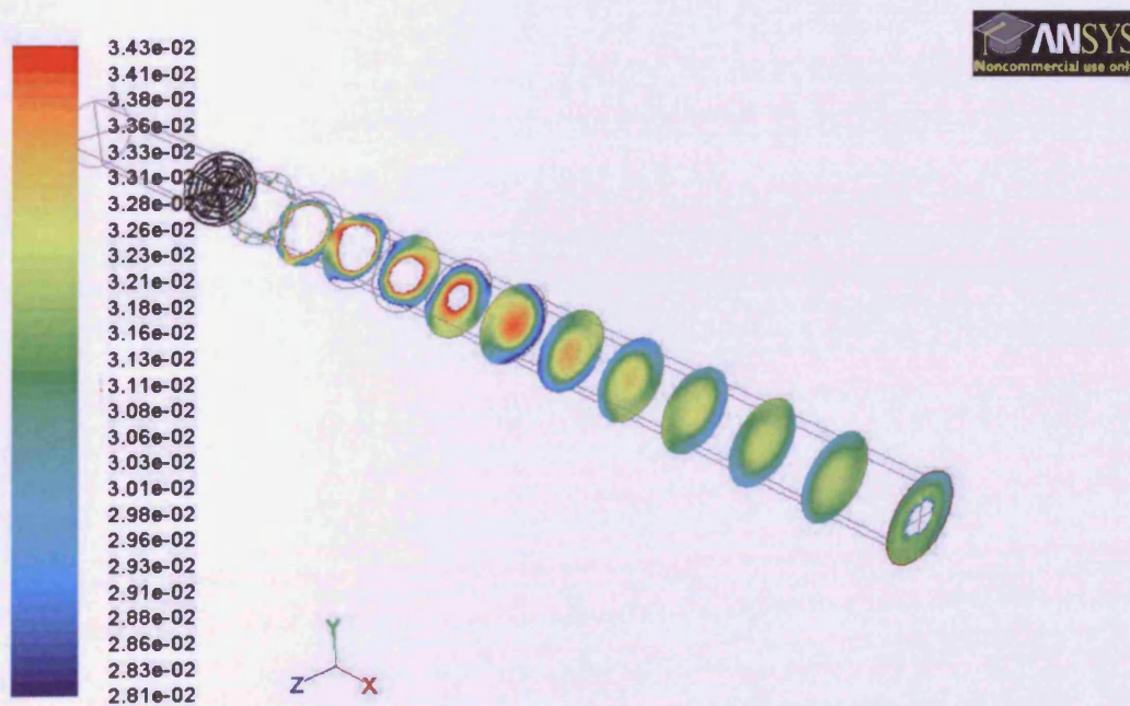
Figure 8.27a: Inner Circumferentially Clamped Bottom Outer Radially Clamped Mixing at Half Mass Flow Rate to 10% of target (front view)
