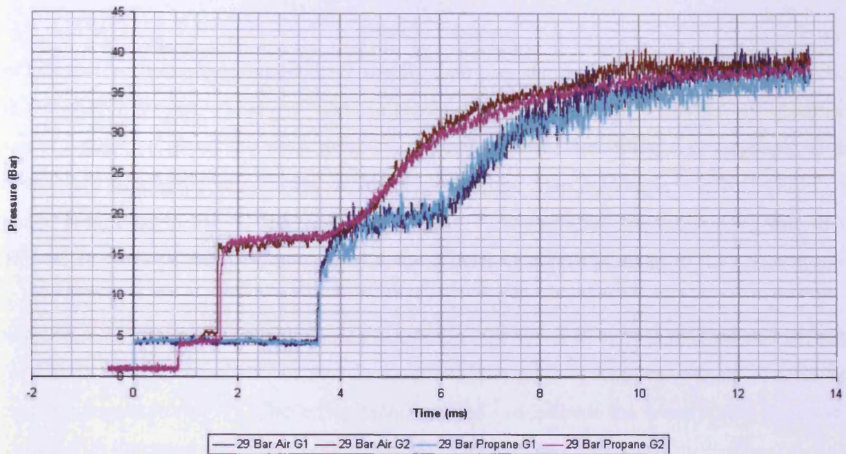
Figure 7.2: Propane Combustion, M=2.00
