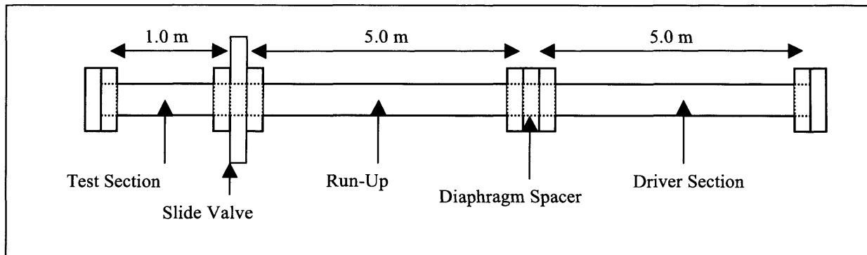
Figure 3.7: Shock Tube Schematic
