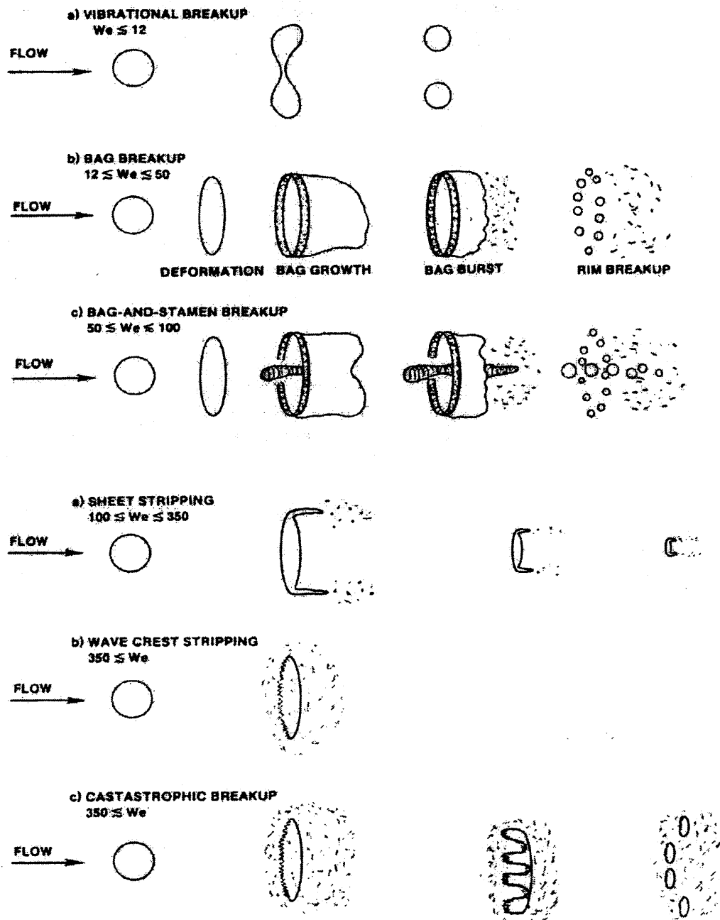
Figure 6.1: Droplet Breakup Processes [66]
