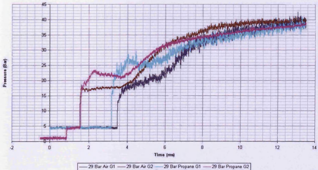
Figure 5.14: Propane Hemispherical Face Results, M=2.00
