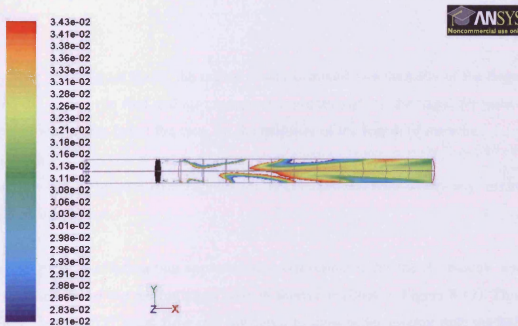
Figure 8.13a: Counter Swirl Mixing at Half Mass Flow Rate RSM Model to 10% of target (cross sectional views)
