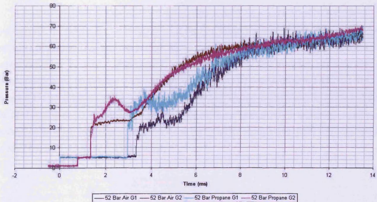
Figure 5.10: Propane Conical Face Results, M=2.16
