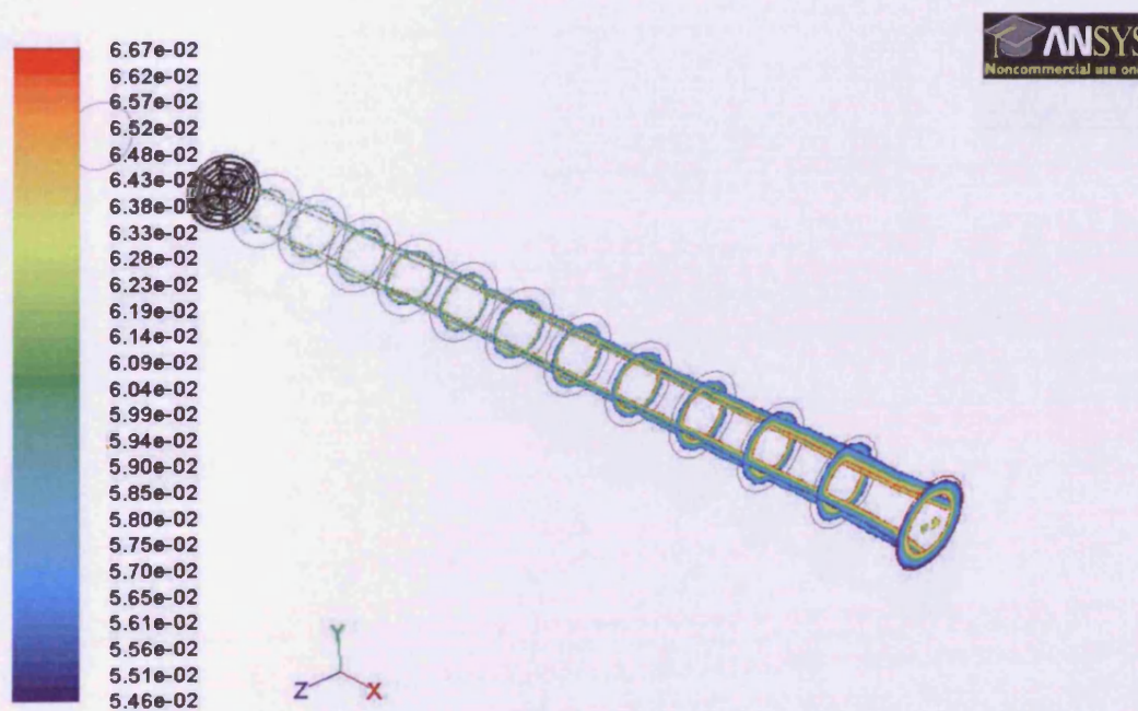
Figure 8.25b: Inner Circumferentially Clamped Bottom Outer Radially Clamped No Fuel Positive X velocity (top view)
