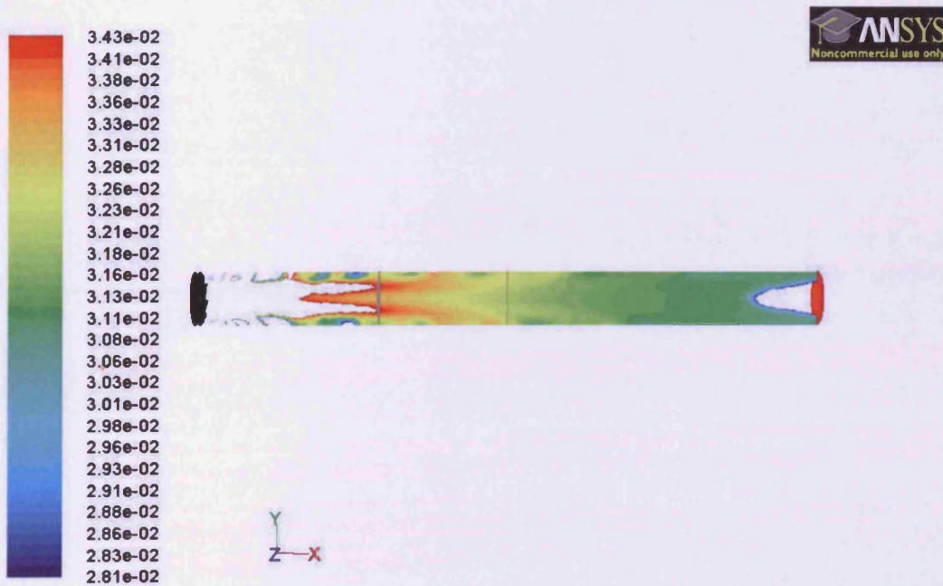
Figure 8.5: Co-Swirl Mixing at Full Mass Flow Rate
