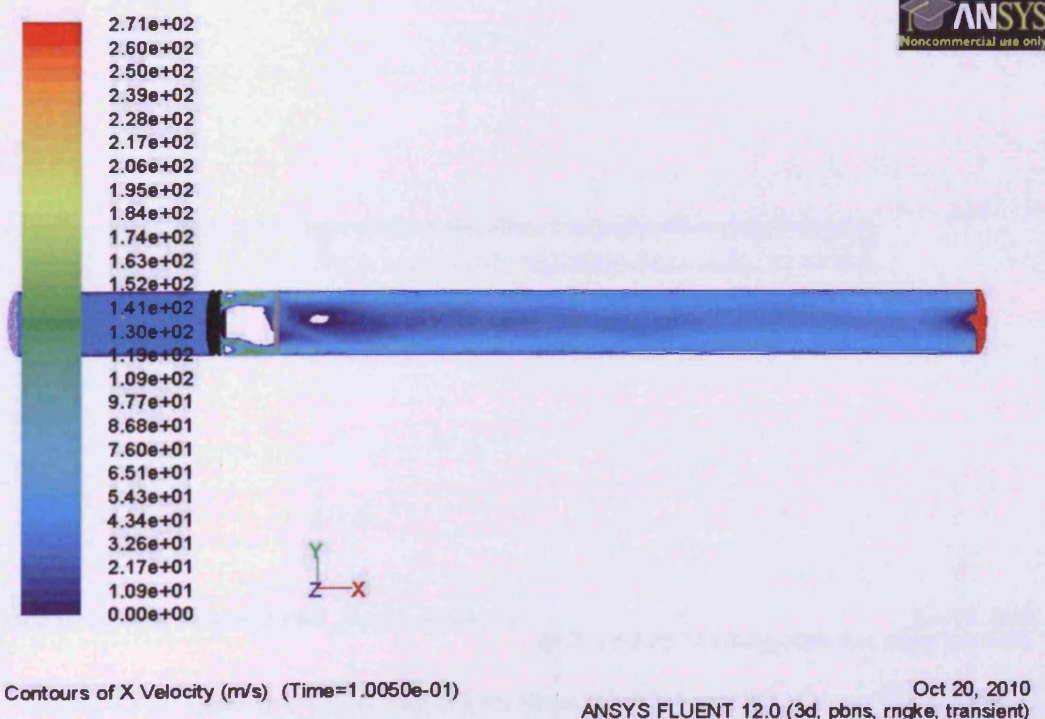
Figure 8.9: Counter-Swirl Positive X Velocity Plot
