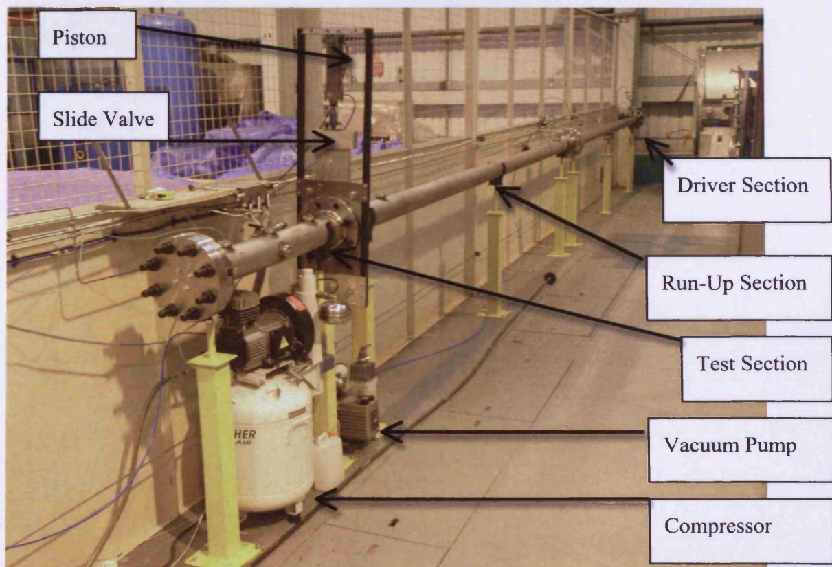
Figure 3.13: 4" Shock Tube
