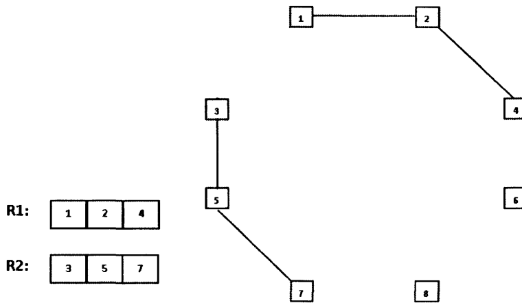
Figure 3.6. 2 Routes and Maximum 3 Nodes Example
