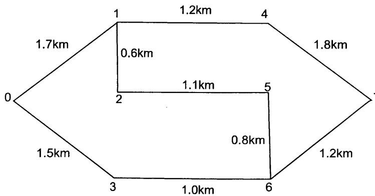
Figure 3.4. 8 Nodes and 9 Links Network
