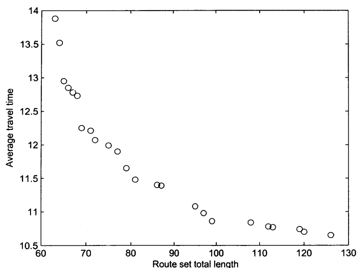
Figure 5.11. Non-dominated Solutions from 10 Runs for 4-route Scenario for Mandl's Network (route length and travel time both measured in minutes)
