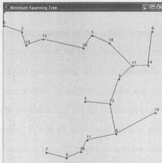
Figure 3.2. Minimum Spanning Tree
