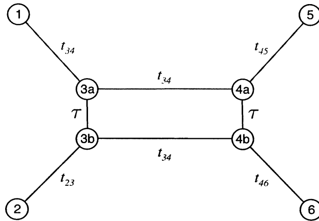
Figure 6.2. New Transit Network
