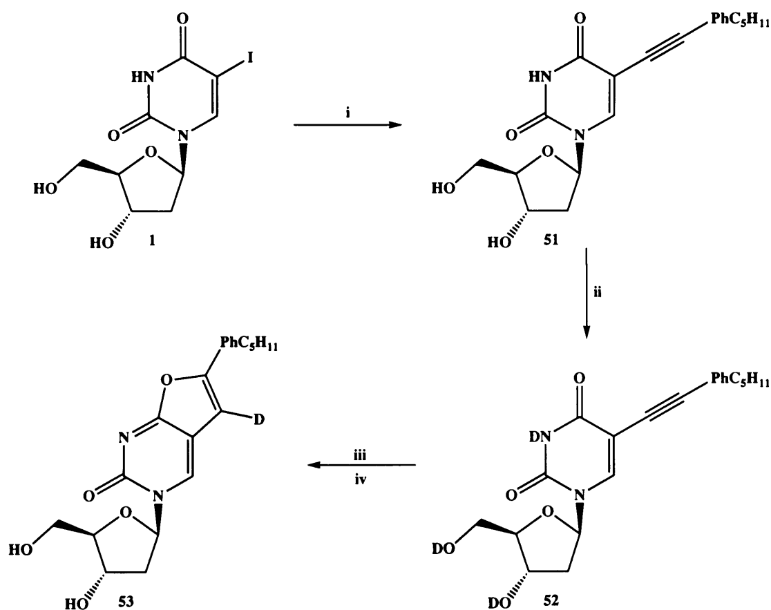
Scheme 3.4: i) DMF, 4-pentylphenylacetylene, Tetrakis \text{Pd}(\text{PPh}_3)_4 , \text{CuI} , DIPEA. ii) \text{CH}_3\text{OD} . iii) \text{CH}_3\text{OD} , TEA, \text{CuI} , \Delta . iv) \text{MeOH} .
