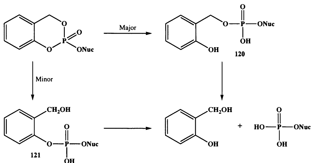
Scheme 5.3: Activation of CycloSal pronucleotide
