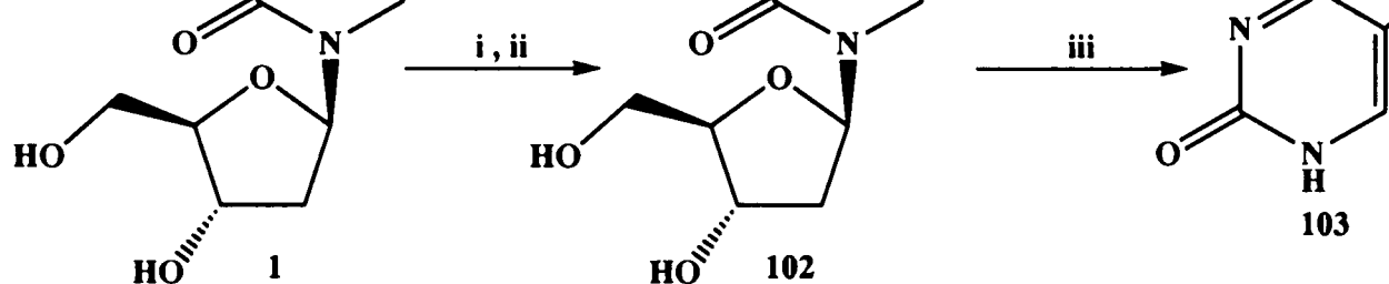
Scheme 4.6: i) DMF, 4-ethynyl-BOC-aniline, Tetrakis Pd(PPh 3 ) 4 , CuI, DIPEA. ii) CuI, TEA. iii) TFA, 100 °C, 1 h.
