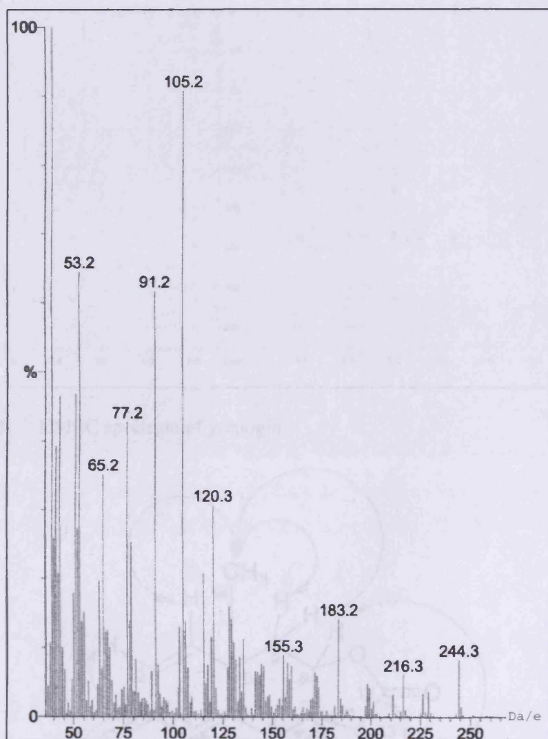
Figure 5.12. Mass spectrum of yomogin.
