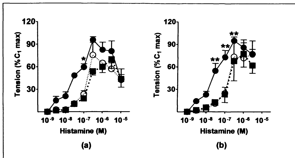
Figure 5.25. Effects of (a) yomogin (n=4) and (b) mixture of yomogin and 1,2,3,4-diepoxyl-11(13) eudesmen-12,8-olide (n=4) on contractile responses of the guinea pig ileum to histamine. Responses are the mean ( \pm S.E.M.) contractions expressed as a percentage of the maximum contraction of CRC 1 . Mean responses ( \pm S.E.M.) on individual concentrations of CRC 1 and CRC 2 were compared by repeated measures ANOVA followed by Bonferroni pos-hoc test. Significant (*, P < 0.05 or **, P < 0.01 ) differences were seen between CRC 1 and CRC 2 . ●—● CRC 1 after 30 min tissue equilibration, ■—■ CRC 2 after 30 min tissue equilibration after the wash out of first curve, and ○--○ CRC 3 after 30 min tissue equilibration from the washout of second curve. 1 mg of the plant extracts dissolved in 0.1 mL DMSO was added prior to the construction of CRC 2 .
