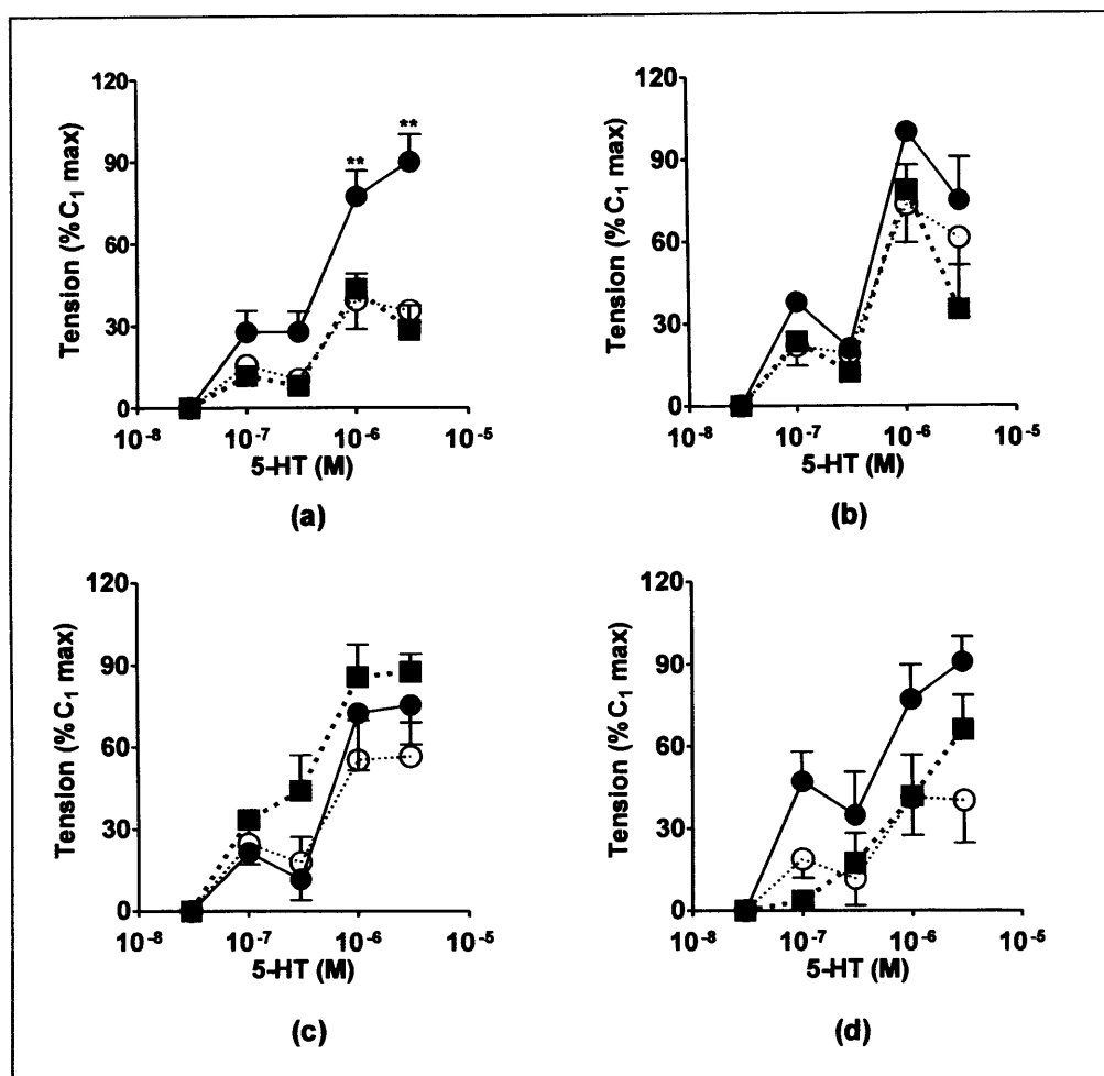
Figure 3.2. Effects of chloroform and methanol extracts of S. grandiflora on mean cumulative CRCs of guinea pig ileum for contractions to 5-HT, (a) SGF-CHCl 3 , n=4, (b) SGF-MeOH, n=4, (c) SGL-CHCl 3 , n=4, and (d) SGL-MeOH, n=4. Responses are the mean ( \pm S.E.M.) contractions expressed as a percentage of the maximum contraction of CRC 1 . Mean responses ( \pm S.E.M.) on individual concentrations of CRC 1 and CRC 2 were compared by repeated measures ANOVA followed by Bonferroni pos-hoc test. Significant (P<0.01, **) differences between CRC 1 and CRC 2 . ●—● CRC 1 after 30 min tissue equilibration, ■—■ CRC 2 after 30 min tissue equilibration after the wash out of first curve, and ○--○ CRC 3 after 30 min tissue equilibration from the washout of second curve. 1 mg of S. grandiflora crude extract dissolve in 0.1 mL DMSO was added prior to the construction of CRC 2 .
