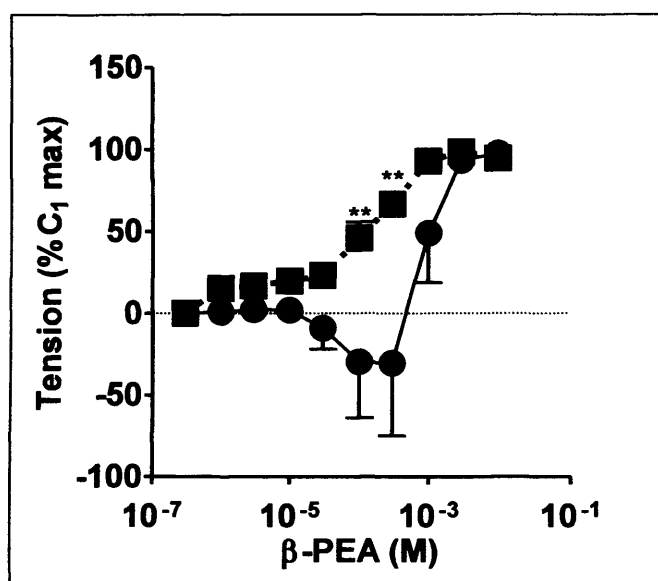
Figure 2.18. Mean cumulative CRCs for contractile responses of the guinea pig trachea to \beta -PEA. Responses are the mean ( \pm S.E.M.) contractions expressed as a percentage of the maximum contraction of CRC 1 . Mean responses ( \pm S.E.M.) on individual concentrations of the \beta -PEA CRC with ( n=4 ) and without propranolol ( n=4 ) were compared by repeated measures ANOVA followed by Bonferroni pos-hoc test. Significant ( P<0.01 , **) differences. ●—● CRC after 60 min tissue equilibration and ■—■ CRC after 60 min tissue equilibration with 1\times 10^{-6} M propranolol.
