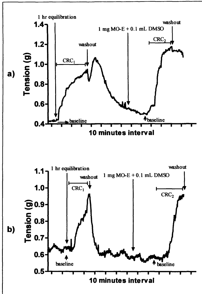
Figure 4.11. Representative chart recording showing the effects of M. oleifera acid-base extracts in repeated contractile response CRCs of the guinea pig aorta to (a) phenylephrine (refer to section 2.4.15 for phenylephrine concentrations used for each CRC) and (b) \beta -PEA (refer to section 2.4.17 for \beta -PEA concentrations used for each CRC).
