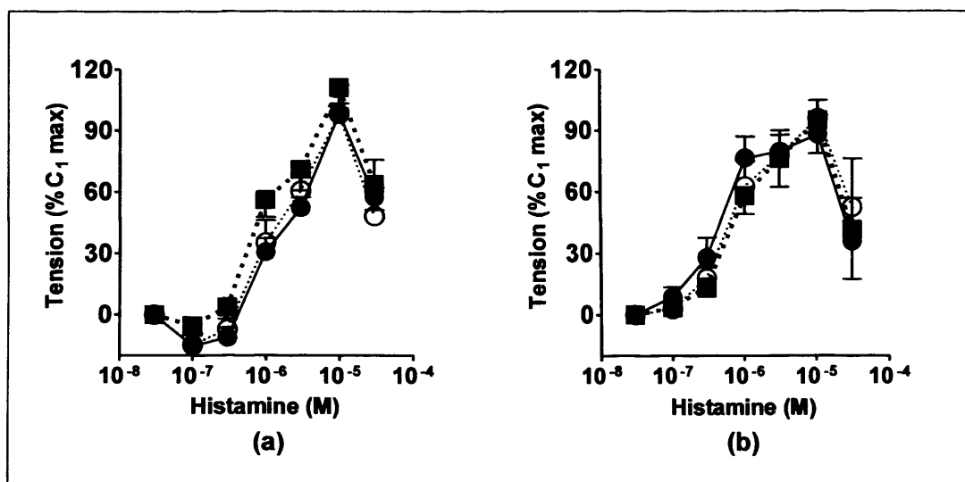
Figure 2.9. Mean cumulative CRCs for the contractile responses of the guinea pig ileum to histamine. (a) Repeated CRCs for histamine (n=4), (b) effect of DMSO added during CRC 2 on histamine (n=4). Responses are the mean ( \pm S.E.M.) contractions expressed as a percentage of the maximum contraction of CRC 1 . Mean responses ( \pm S.E.M.) on individual concentrations of CRC 1 vs. CRC 2 , and CRC 2 vs. CRC 3 were compared by repeated measures ANOVA followed by Bonferroni pos-hoc test. No significant ( P>0.05 ) differences were seen at each dose between CRC 1 , CRC 2 and CRC 3 of 5-HT. ●—● CRC 1 , ■—■ CRC 2 after 30 min tissue equilibration after the wash out of first curve with or without DMSO, and ○--○ CRC 3 after 30 min tissue equilibration from the washout of second curve
