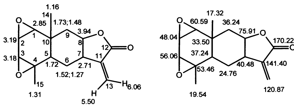
Figure 5.24. 1 H-NMR and 13 C-NMR chemical shift of 1,2,3,4-diepoxy-11(13)-eudesmen-12,8-olide
