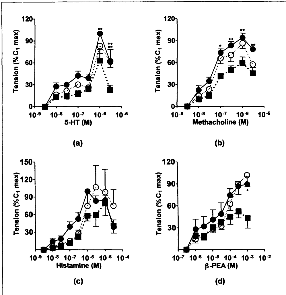
Figure 4.7. Effects of acid-base extracts of M. Oleifera (MO-E) on mean cumulative CRCs of guinea pig ileum for constriction to (a) 5-HT, n=4 , (b) methacholine, n=4 , (c) histamine, n=5 , and (d) \beta -PEA, n=4 . Responses are the mean ( \pm S.E.M.) contractions expressed as a percentage of the maximum contraction of CRC 1 . Mean responses ( \pm S.E.M.) on individual concentrations of CRC 1 and CRC 2 were compared by repeated measures ANOVA followed by Bonferroni pos-hoc test. Significant differences (*, P<0.05 or **, P<0.01 ) between CRC 1 and CRC 2 or (+, P<0.01 ) between CRC 2 and CRC 3 . ●—● CRC 1 after 30 min tissue equilibration, ■—■ CRC 2 after 30 min tissue equilibration after the wash out of first curve, and ○—○ CRC 3 after 30 min tissue equilibration from the washout of second curve. 1 mg of M. oleifera crude extract dissolved in 0.1 mL DMSO was added 20 min prior to the construction of CRC 2 .
