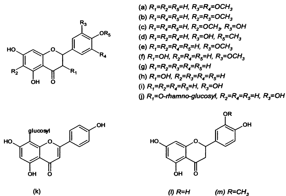
Figure 1.24. Estrogenic Flavonoids from A. vulgaris L. (a) Tricin, (b) Jaceosidine, (c) Eupalofin, (d) Diosmetin, (e) Chrysoeriol, (f) Isorhamnetin, (g) Apeginin, (h) Kaempferol, (i) Luteolin, (j) Rutin, (k) Vitexin, (l) Eriodictyol, and (m) Homoeriodictyol (Lee et al. , 1998).
