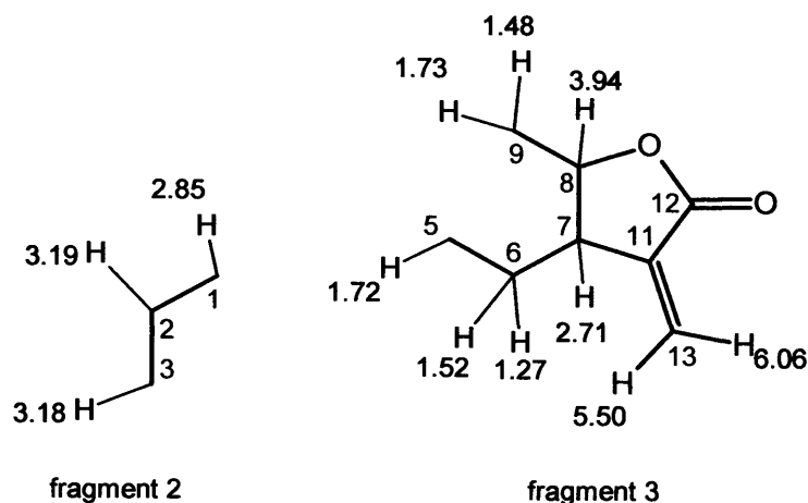
Figure 5.21. COSY and HSQC correlations of 1,2,3,4-diepoxy-11(13)-eudesmen-12,8-olide.
