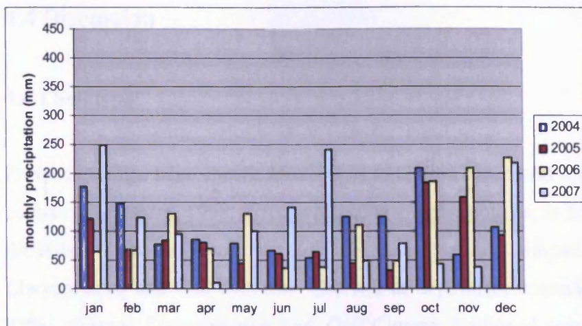
Figure 4.31: Monthly total precipitation during all years at Llysindnam.
