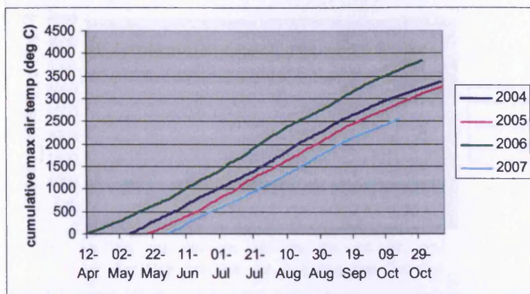
Figure 4.22: Annual cumulative maximum air temperatures obtained during the Miscanthus growing seasons, defined as the frost-free periods, at Llysdim.
