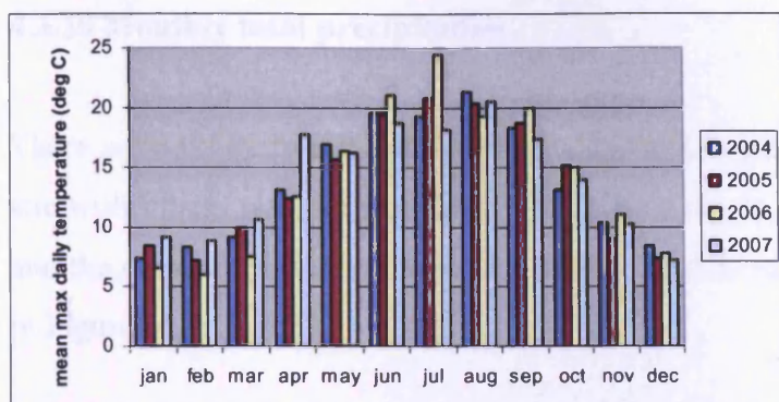
Figure 4.26: Monthly mean maximum daily temperatures for all years at Llysdimam.
