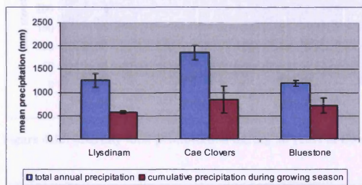
Figure 4.30: Mean \pm 1 standard deviation annual precipitation and cumulative precipitation during the Miscanthus growing season.
