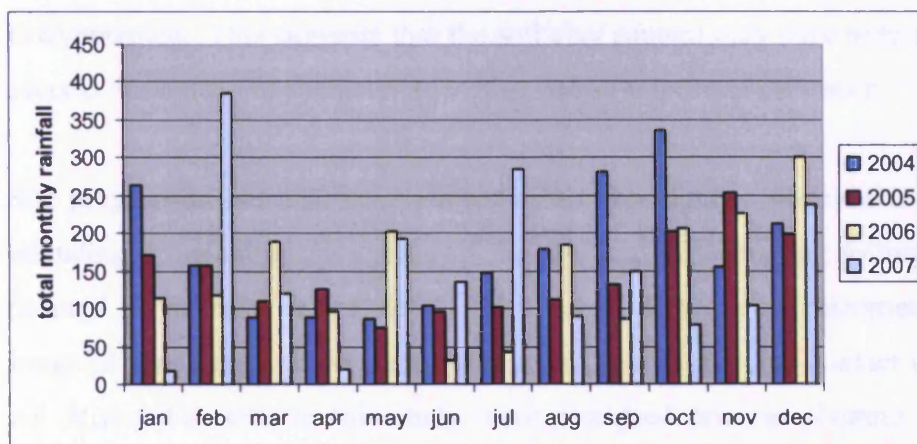
Figure 4.32: Monthly total precipitation during all years at Cae Clovers.
