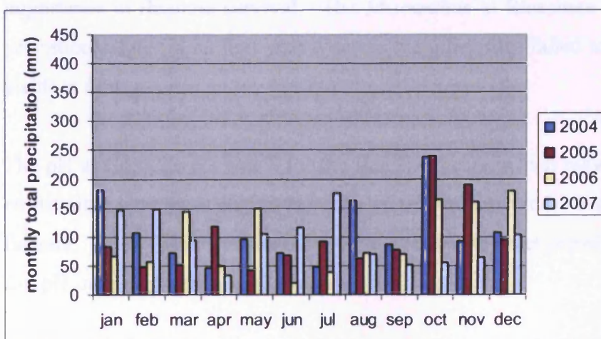
Figure 4.33: Monthly total precipitation during all years at Bluestone.
