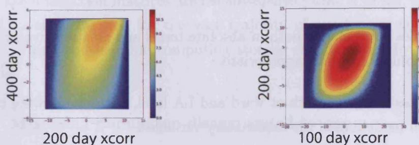
Figure 5.7: Scatter density plots of longer vs shorter term cross-correlation. Again, wmin = 0 and wmax = 1 , while time slice length varies. Frequency ( z ) axis shows natural logarithmic frequency count \ln(f + 1) .
