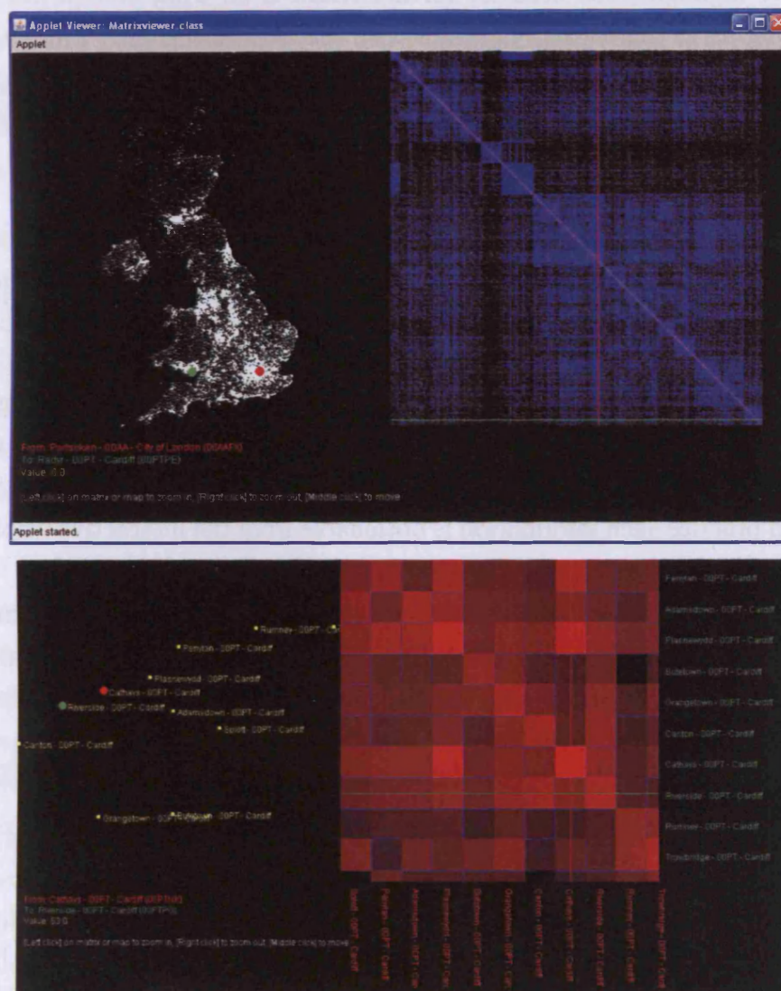
Figure 3.14: Screenshots of software showing Ward level visualisation of UK internal migration, at wide and close zoom levels. Text to the left of the display shows names of the currently selected origin and destination, together with the relevant value(s) from the interaction matrix. For close levels of zoom (shown in the lower figure), place names are added to both the map and matrix.
