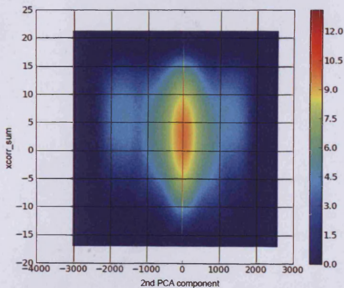
Figure 5.10: Plot of cross-correlation against most correlated component for cross-correlation regression. Frequency ( z ) axis shows natural logarithmic frequency count \ln(f + 1) .
