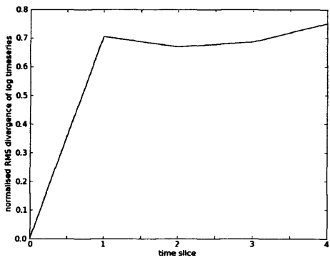
Figure 5.6: Reconstruction of time series based on long-term cross-correlation. In each case, wmin = 0 and wmax = 1 while the time slice length is varied. First time-slice errors are approx. 0.5 for 100 days, 0.6 for 200 days, 0.7 for 400 days and 1.0 for 800 days (not shown).
