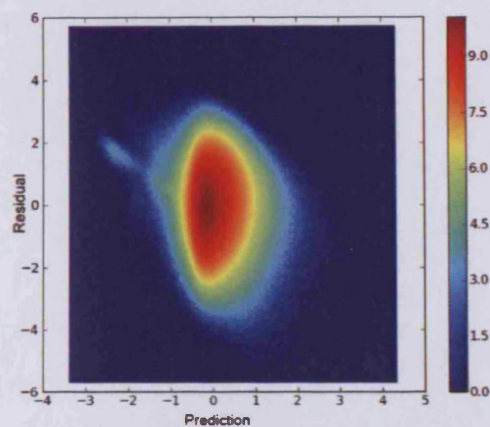
Figure 5.9: Plot of residuals against \text{corr\_sum} values predicted by regression. Frequency ( z ) axis shows natural logarithmic frequency count \ln(f + 1) .
