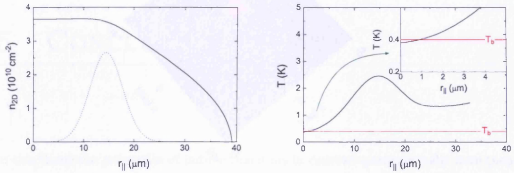
(a) The concentration plotted against radius. The excitation profile is also shown with a dotted line.
