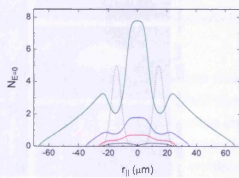
(f) Theoretical results: occupation number of the ground state.
