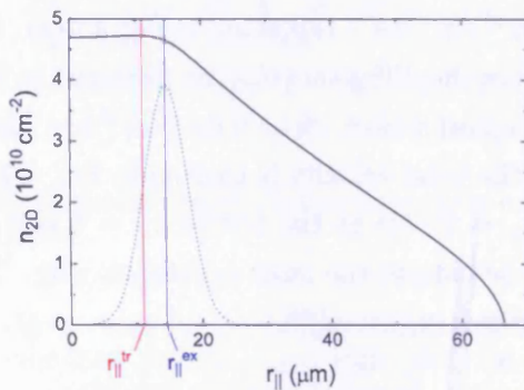
Figure 4.5: The radius of the trap, r_{\parallel}^{\text{tr}} , compared with the radius of the laser ring, r_{\parallel}^{\text{ex}} . The solid curve shows the concentration profile for the highest excitation power, \Lambda_0 = 0.64 \times 10^{10} \text{cm}^{-2}\text{ns}^{-1} and the dotted line shows the excitation laser intensity profile.
