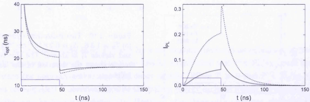
(c) The effective radiative lifetime of excitons plotted against time.
