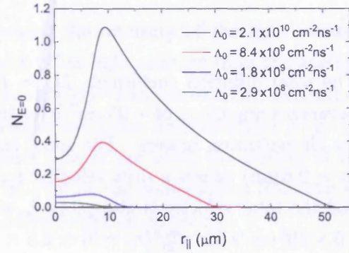
(b) A plot of the occupation number of the ground state against radius for excitation powers.
