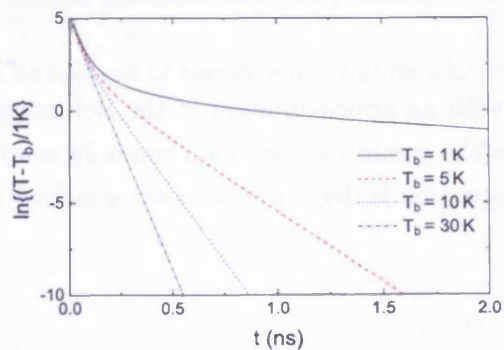
Figure 2.4: A plot of \ln\{(T - T_b)/1\text{K}\} against time for n_{2D} = 10^9 \text{ cm}^{-2} , T_i = 200 K and various lattice temperatures as shown.
