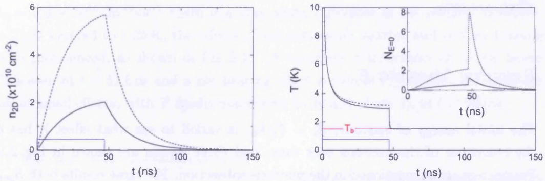
(a) The concentration plotted against time for two excitation powers.
