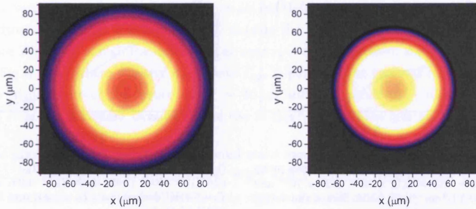
(a) Constant diffusion coefficient, D_x = D_x^c = 100 \text{ cm}^2/\text{s} .
