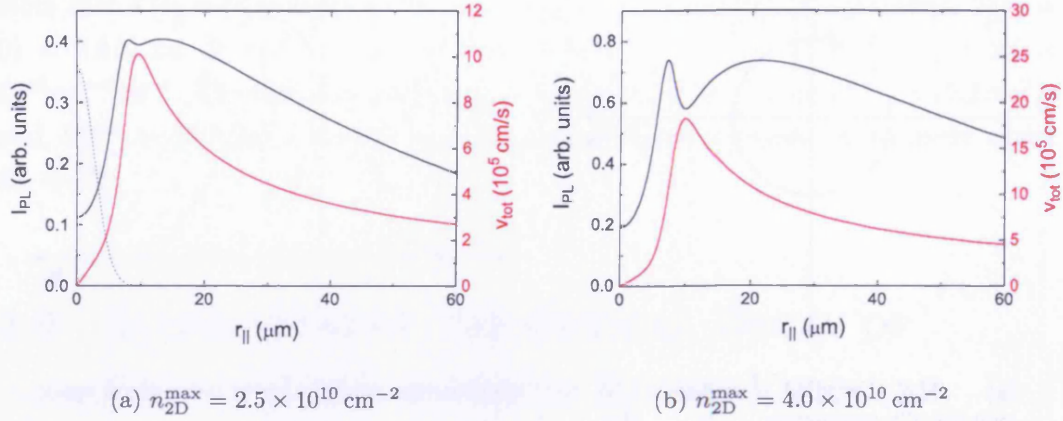
Figure 3.18: PL signal and total velocity plotted against radius for D_x = D_x^c = 100 \text{ cm}^2/\text{s} , T_b = 1.5 \text{ K} , T_i = 200 \text{ K} and two different concentrations.
