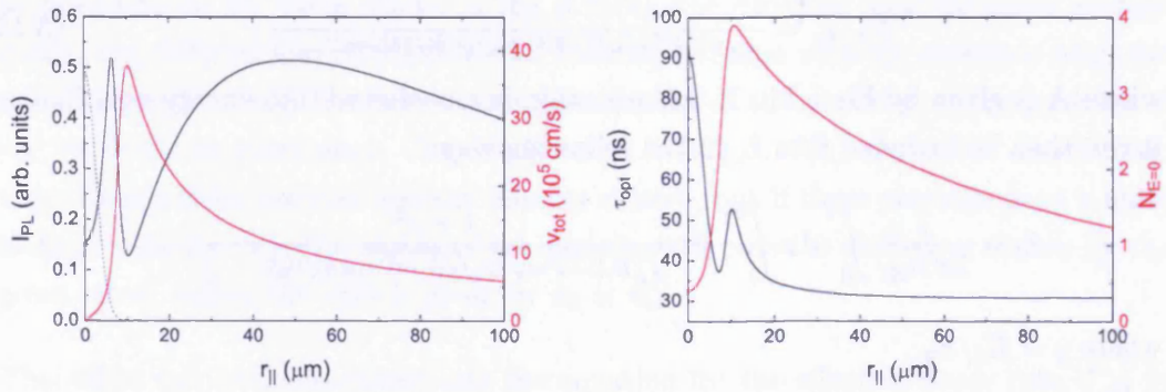
(a) PL signal and total velocity plotted against radius.
