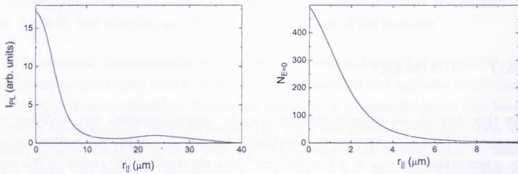
(c) PL signal plotted against radius.
