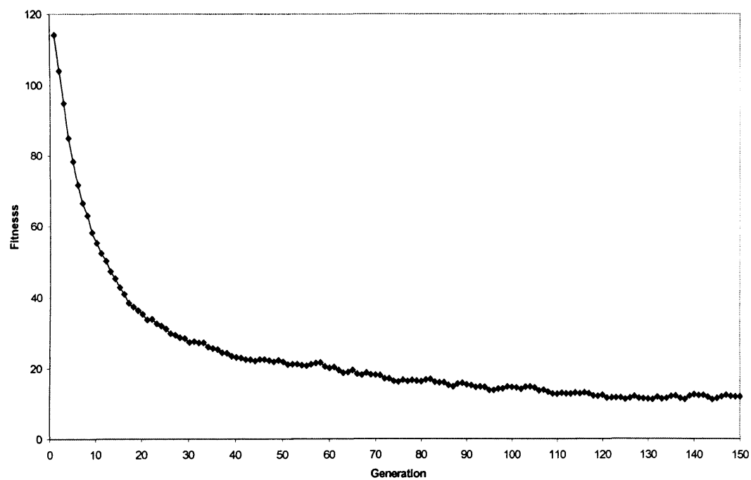
Figure 4-27 150 Generations
