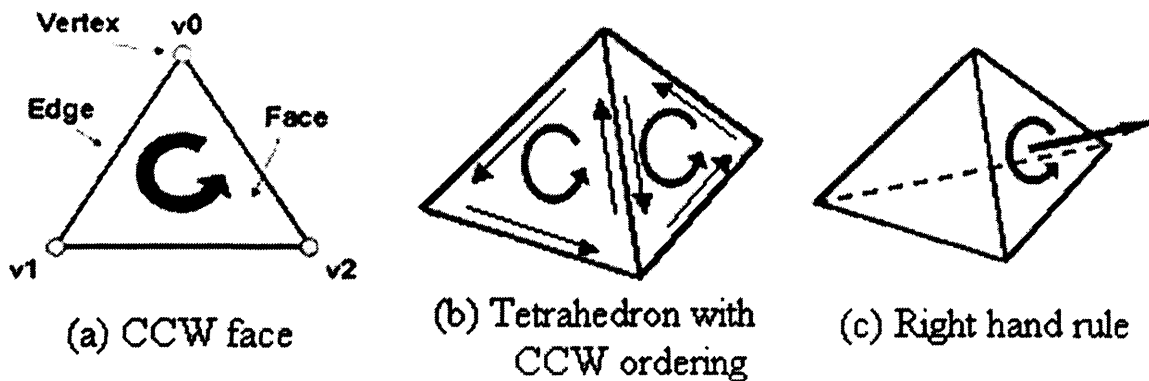
Figure 5-5 Polyhedral properties
