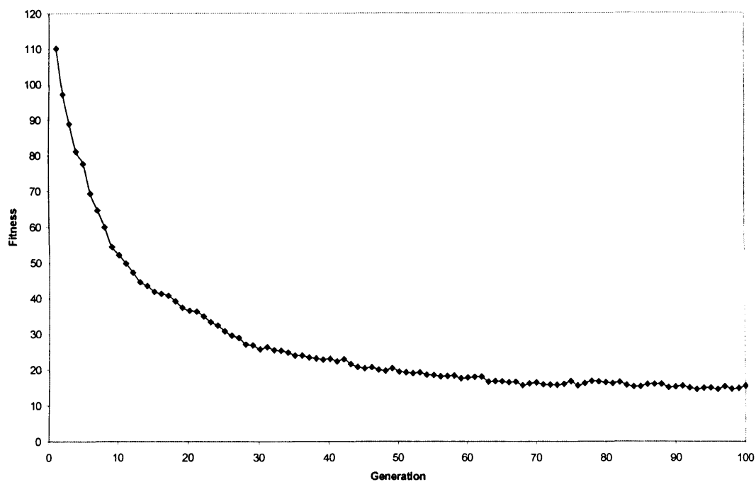
Figure 4-26 100 Generations
