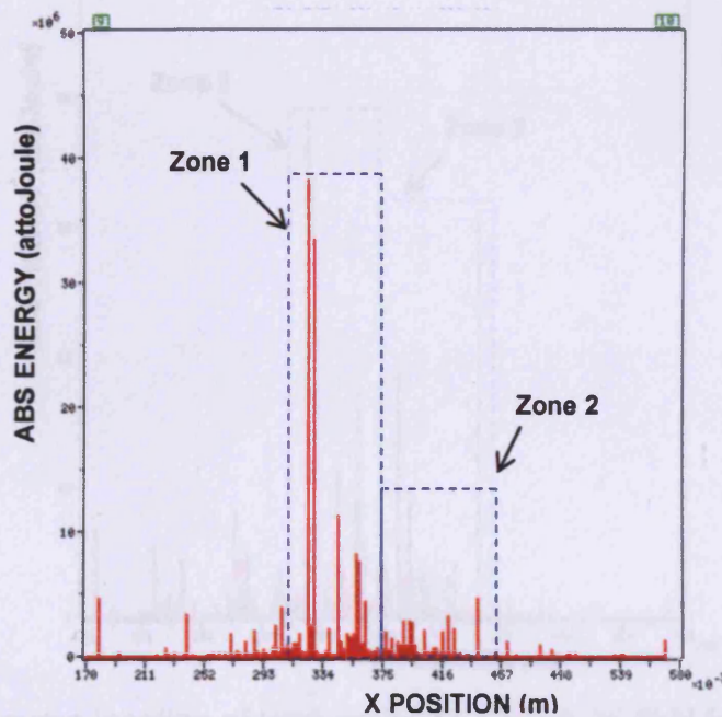
Figure 4.33: Source location of total emission from 0-17.5kN for B22PS
