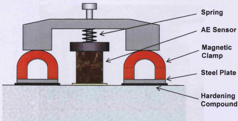
Figure 3.12: Magnetic clamp
