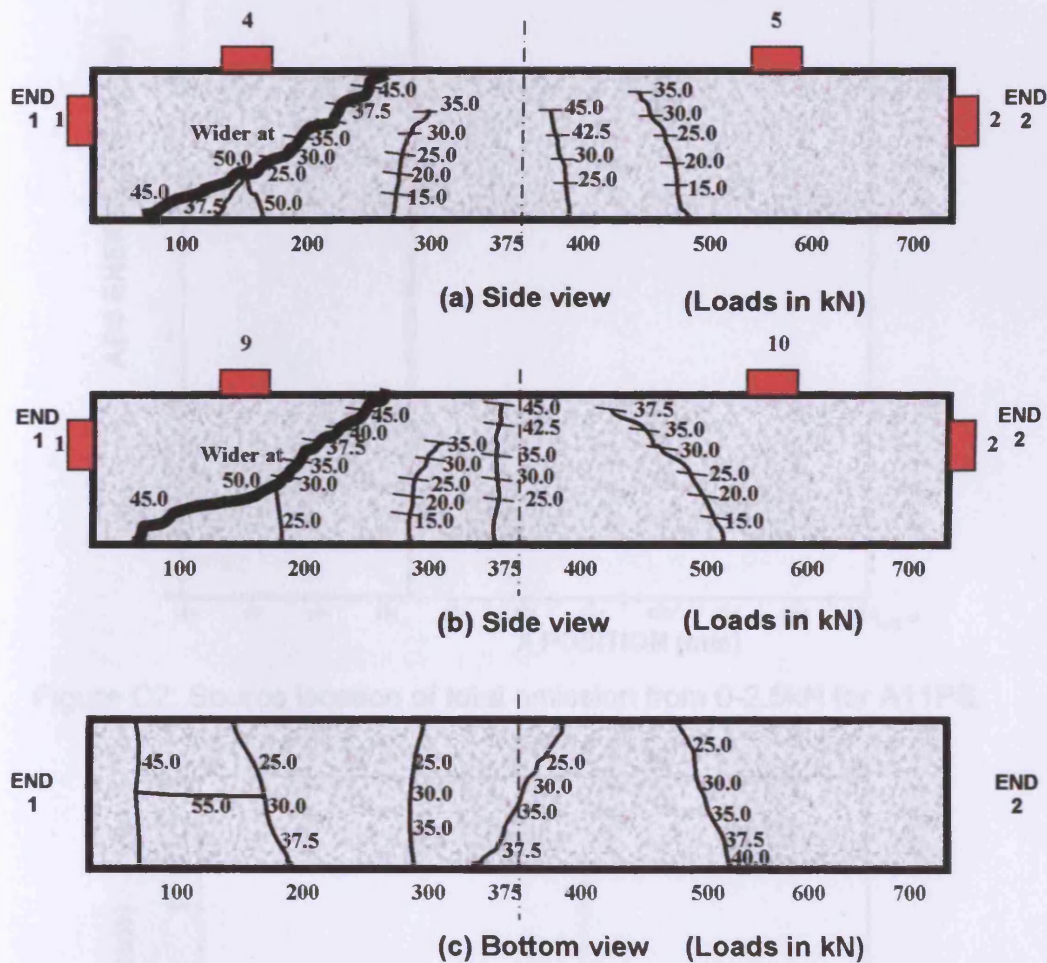
Figure C1: Crack pattern from visual observation for A11PS
