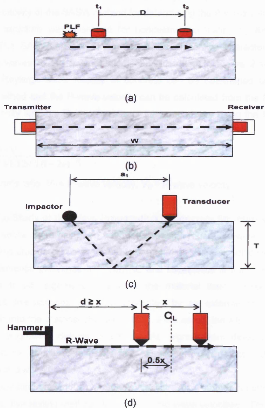
Figure 2.4: Four kinds of stress wave velocity measurements
