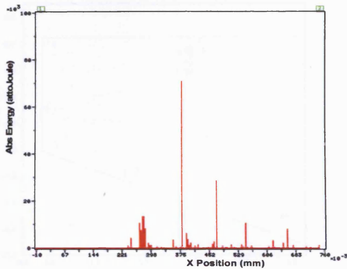
Figure 3.6: 2D linear location plot from DiSP-LOC.
