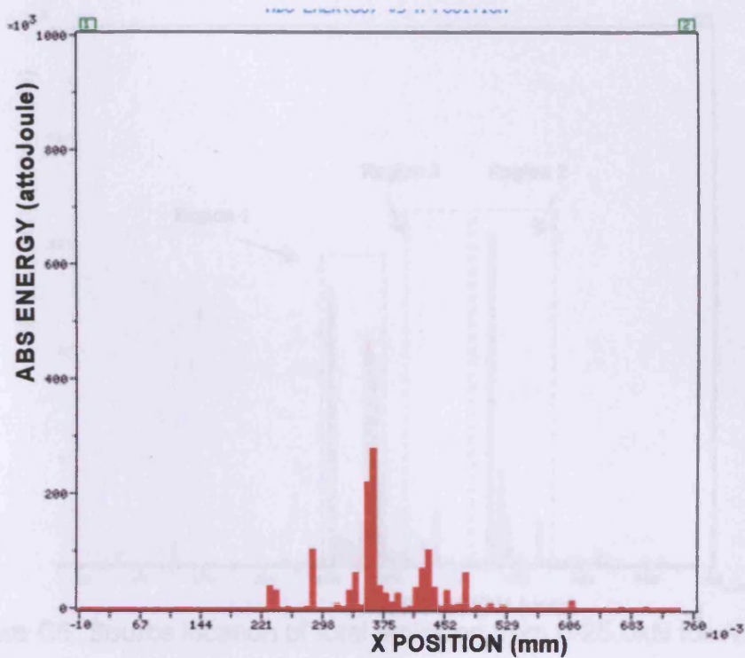
Figure C4: Source location of total emission from 0-10.0kN for A11PS.
