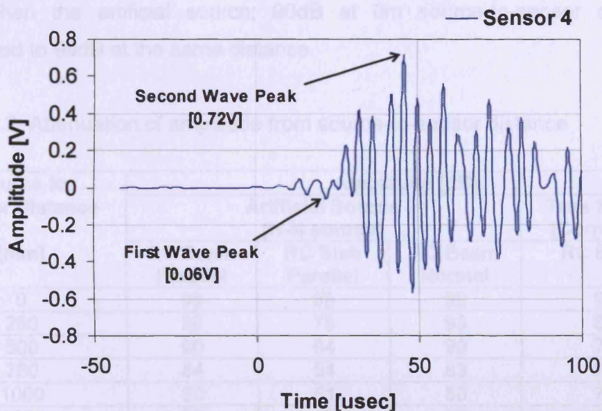
Figure 5.18: Signal recorded at sensor 4 during corrosion test.
