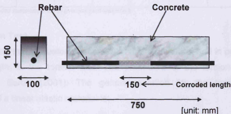
Figure 4.1: Dimension of concrete beam specimen.
