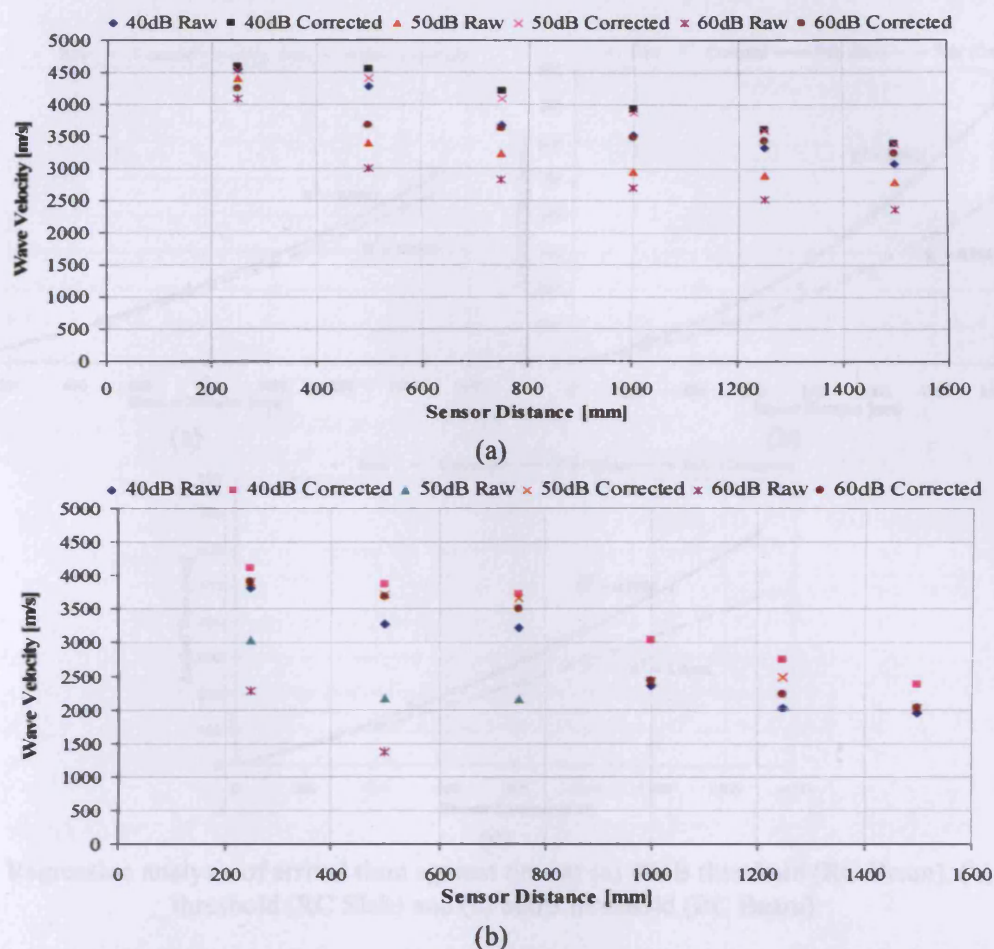
Fig. 5. Wave velocity for raw and corrected signal at 40dB, 50dB and 60dB for (a) RC beam (b) RC slab
