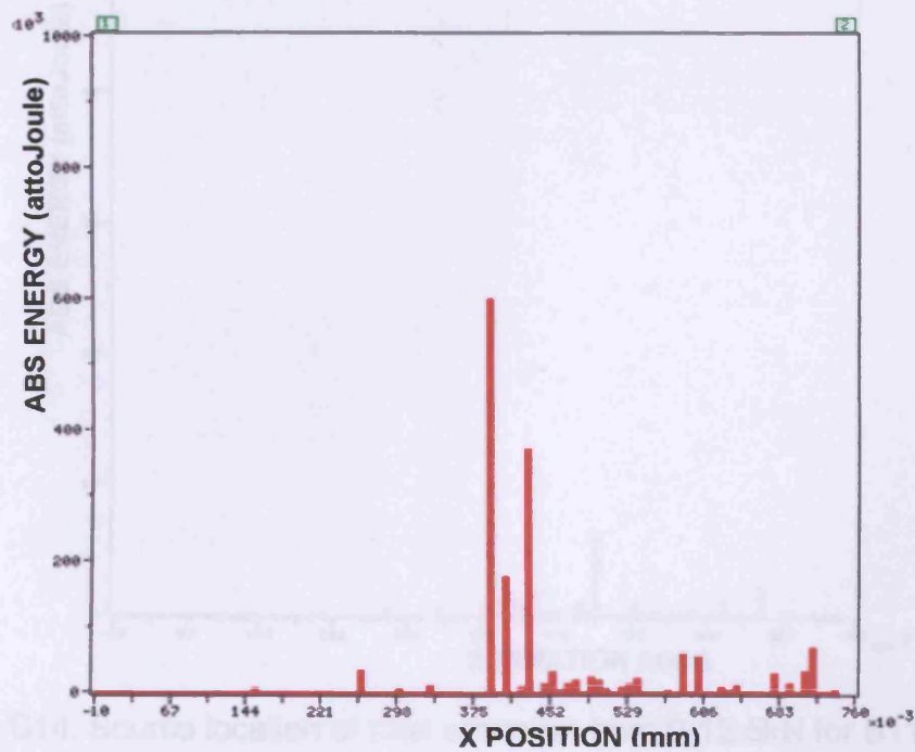
Figure C12: Source location of total emission from 0-5.0kN for B11PS.
