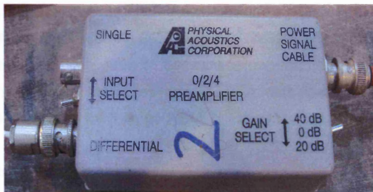
Figure 3.4: PAC's 0/2/4 preamplifier
