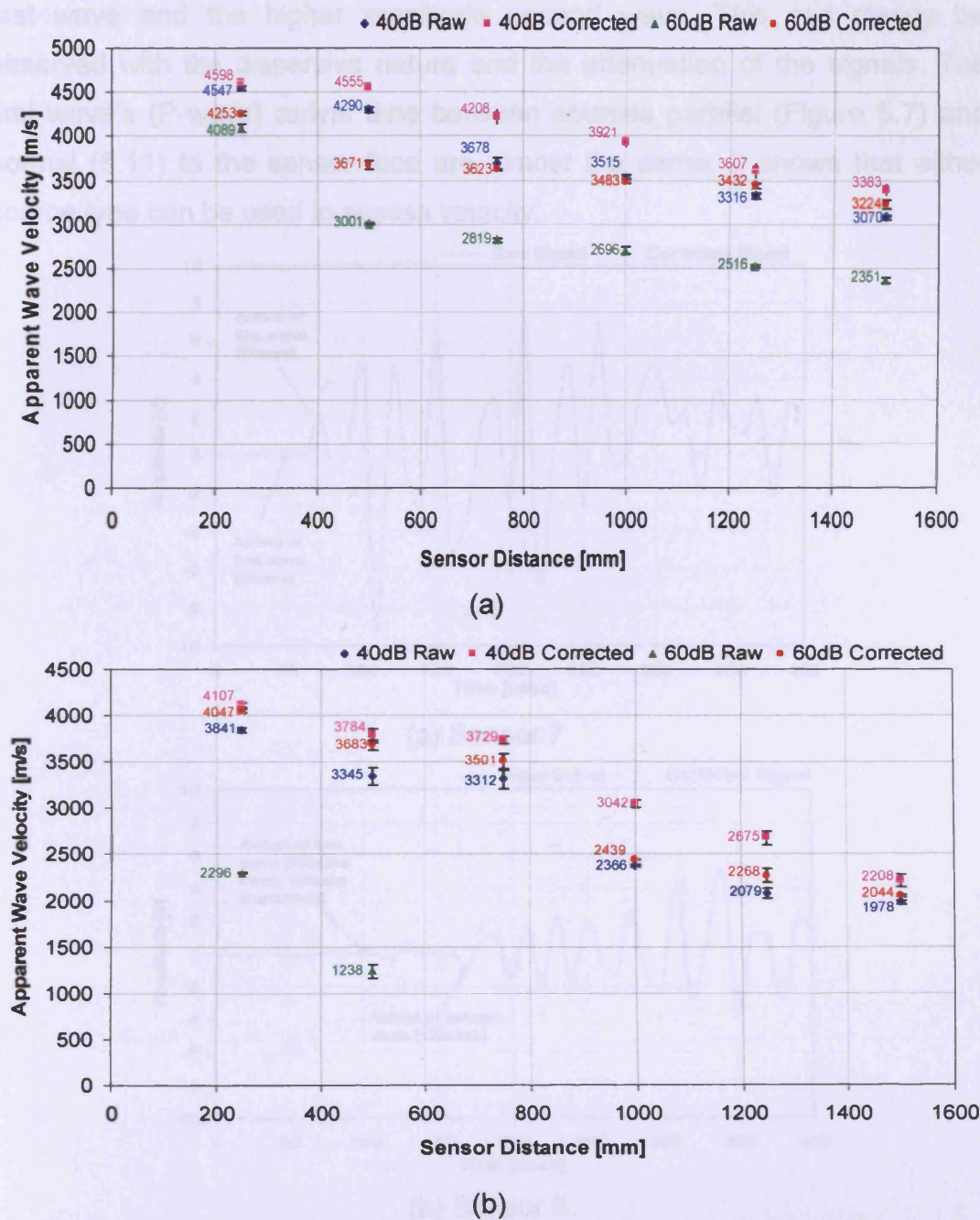
Figure 5.10: Apparent wave velocity for raw and corrected signal of source parallel to sensor face for (a) RC beam and (b) RC slab at 40dB and 60dB.
