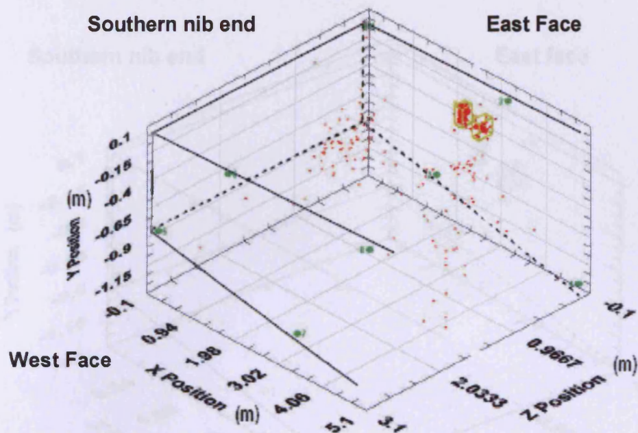
Figure 6.7: Crosshead 68 Southern Nib AE Source Location – 3D View.
