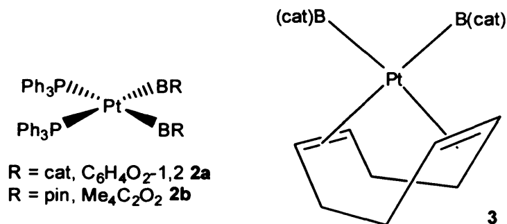
Figure 1 – The platinum diboryl complexes, 2a-b and 3
