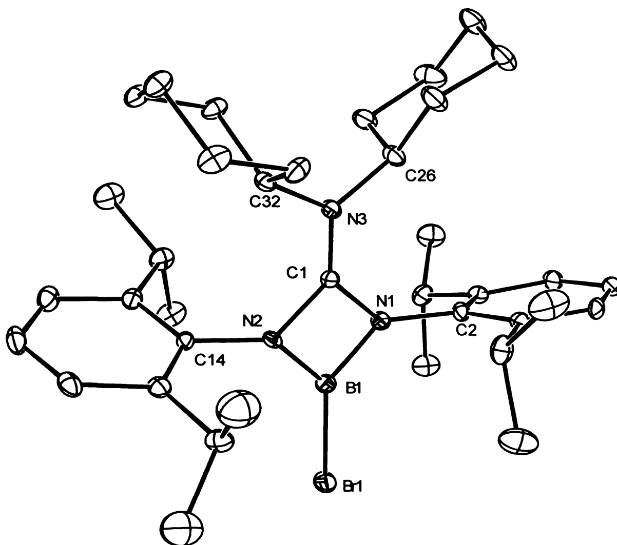
Figure 8 – Thermal ellipsoid plot (25 % probability surface) of the structure of the cationic component of [\text{BrB}(\text{Giso})][\text{GaBr}_4] 24 ; hydrogen atoms omitted for clarity. Selected bond lengths (Å) and angles (°): \text{Br}(1)\text{—B}(1) 1.881(8), \text{N}(1)\text{—C}(1) 1.400(9), \text{N}(1)\text{—B}(1) 1.451(11), \text{C}(1)\text{—N}(3) 1.288(9), \text{C}(1)\text{—N}(2) 1.409(9), \text{B}(1)\text{—N}(2) 1.425(11), \text{C}(1)\text{—N}(1)\text{—B}(1) 85.9(6), \text{N}(1)\text{—C}(1)\text{—N}(2) 95.2(5), \text{N}(2)\text{—B}(1)\text{—N}(1) 92.3(6), \text{C}(1)\text{—N}(2)\text{—B}(1) 86.6(6).
