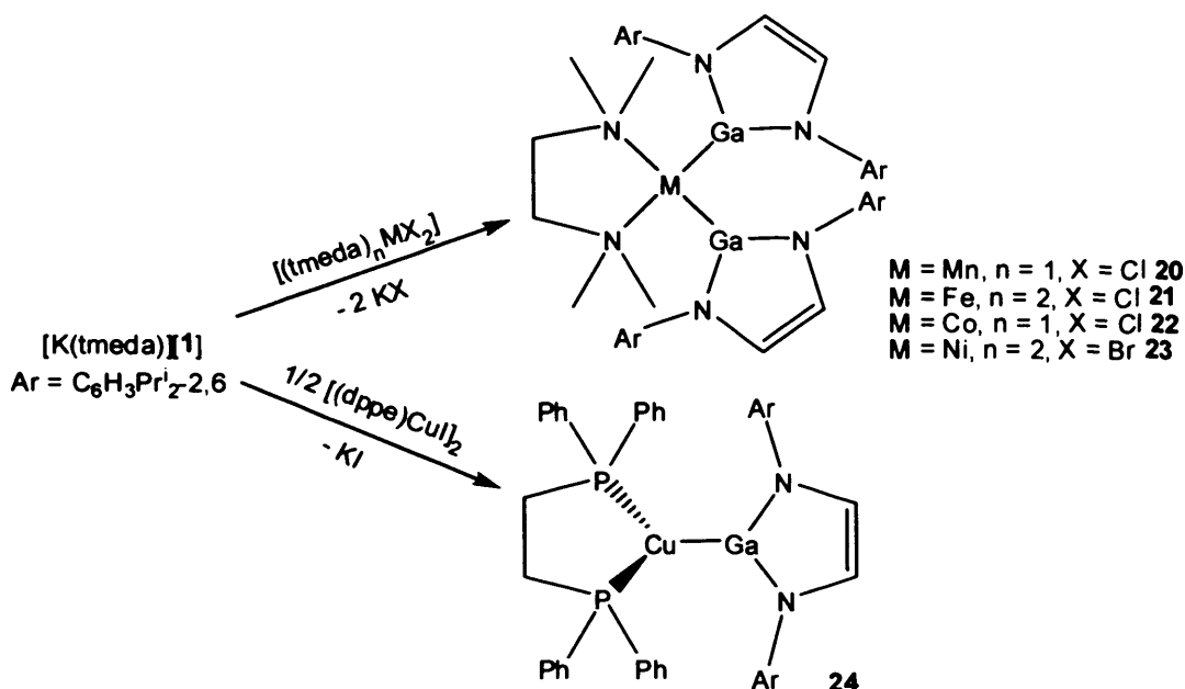
Scheme 7 – The synthesis of 20 – 24
