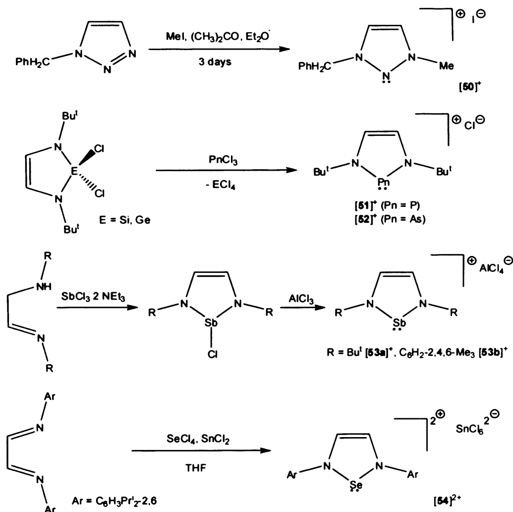
Scheme 11 – The synthesis of 50 – 54
