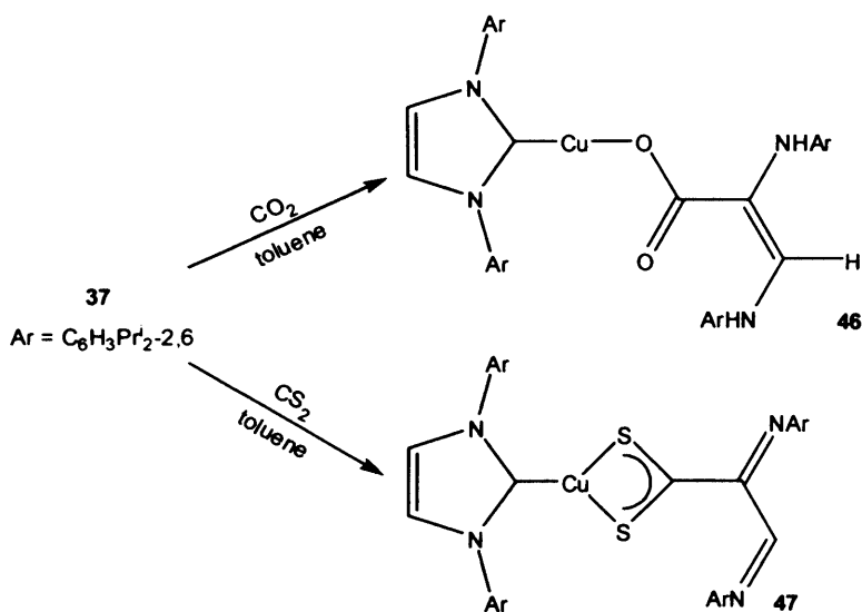
Scheme 14 – The synthesis of 46 and 47
