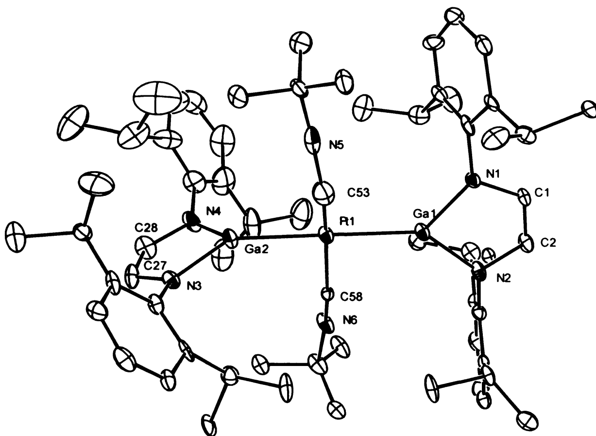
Figure 17 – Thermal ellipsoid plot (25 % probability surface) of the molecular structure of trans -[(Bu i NC) 2 Pt{Ga{[N(Ar)C(H) 2 ]} 2 }] 2 19 ; hydrogen atoms are omitted for clarity.
