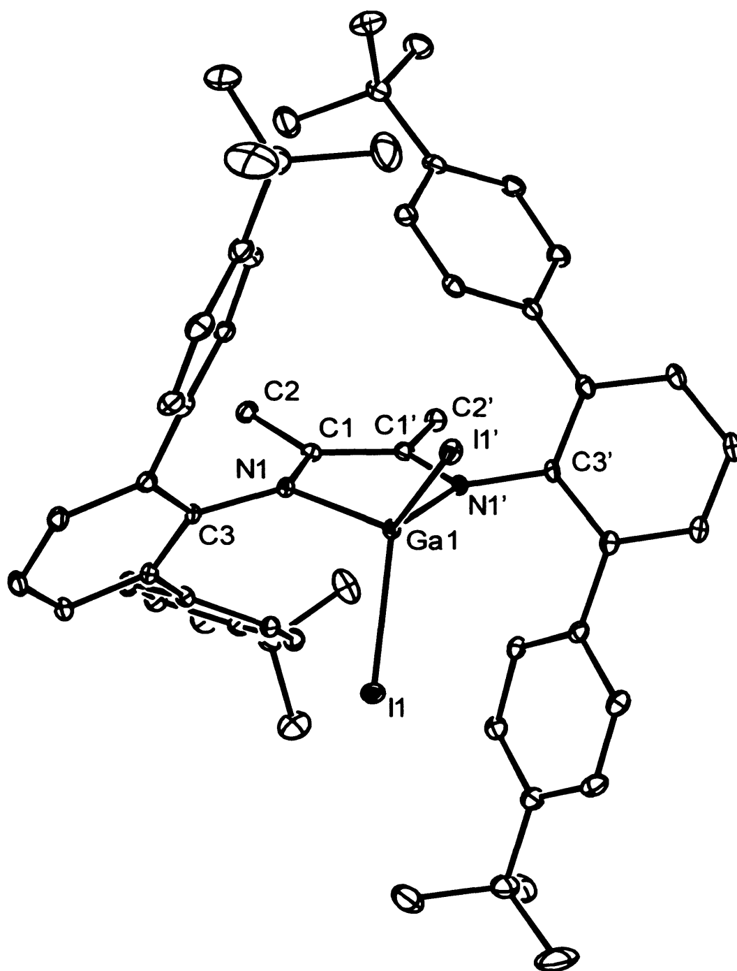
Figure 8 – Thermal ellipsoid plot (25 % probability surface) of the molecular structure of [I_2Ga\{[N(Ar'')C(Me)]_2\}] 12 ; hydrogen atoms omitted for clarity. Selected bond lengths (Å) and angles (°): I(1)—Ga(1) 2.5205(6), Ga(1)—N(1) 1.939(3), N(1)—C(1) 1.341(5), N(1)—C(3) 1.437(4), C(1)—C(1') 1.422(7), N(1')—Ga(1)—N(1) 84.79(18), N(1)—Ga(1)—I(1') 122.12(9), N(1)—Ga(1)—I(1) 108.61(9), I(1')—Ga(1)—I(1) 109.66(3) symmetry operation ' : -x + 1, y, -z + 3/2 .
