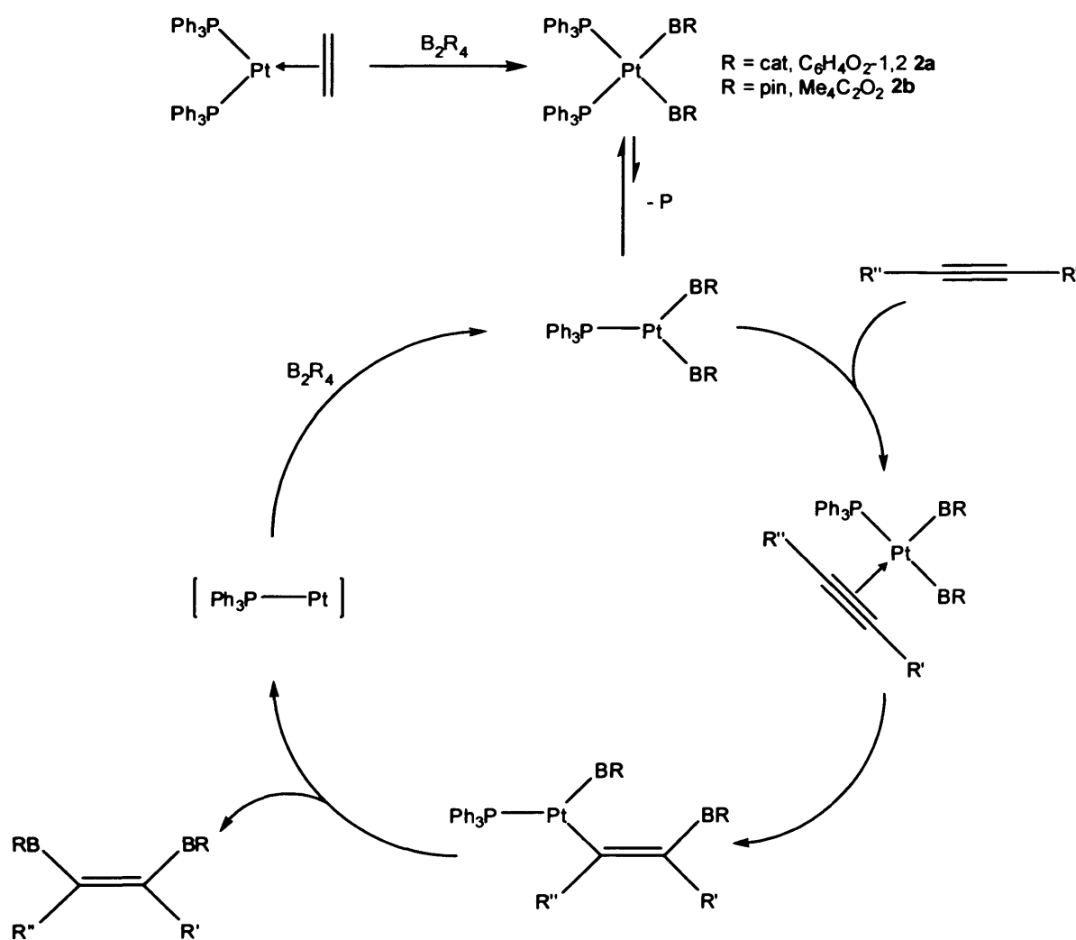
Scheme 1 – A proposed catalytic cycle for the diboration of alkynes mediated by 2a-b
