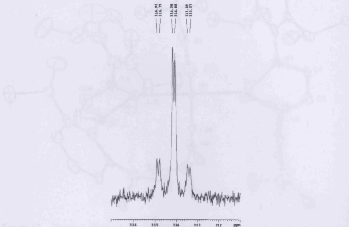
Figure 17 – Detailed chemical shift of the ^{31}\text{P} NMR spectrum of 20 .
