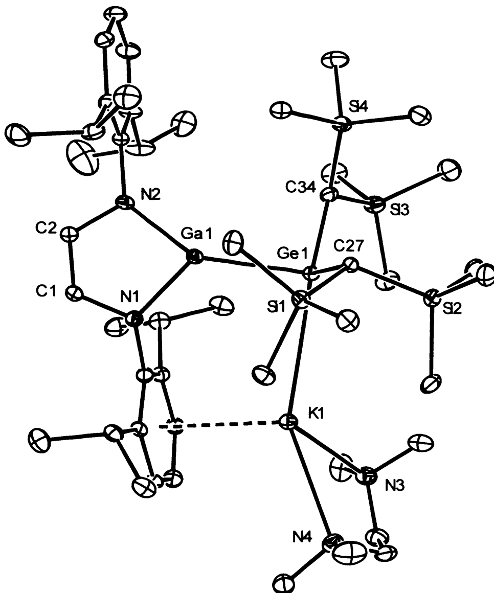
Figure 2 – Thermal ellipsoid plot (25 % probability surface) of the molecular structure of [K(tmeda)][Ge\{CH(SiMe_3)_2\}_2\{Ga\{[N(Ar)C(H)]_2\}] 17 ; hydrogen atoms omitted for clarity. Selected bond lengths (Å) and angles (°): Ge(1)—C(27) 2.085(4), Ge(1)—C(34) 2.091(4), Ge(1)—Ga(1) 2.5396(8), Ge(1)—K(1) 3.4418(12), Ga(1)—N(2) 1.911(4), Ga(1)—N(1) 1.925(4), K(1)—N(3) 2.783(4), K(1)—N(4) 2.959(4), N(1)—C(1) 1.398(6), N(2)—C(2) 1.404(6), C(1)—C(2) 1.324(6), K(1)—centroid (C(3)—C(8)) 2.931(3), C(27)—Ge(1)—C(34) 105.81(18), C(27)—Ge(1)—Ga(1) 106.13(12), C(34)—Ge(1)—Ga(1) 97.15(14), C(27)—Ge(1)—K(1) 106.21(12), C(34)—Ge(1)—K(1) 143.45(14), Ga(1)—Ge(1)—K(1) 90.47(2), N(2)—Ga(1)—N(1) 85.59(15), N(2)—Ga(1)—Ge(1) 148.55(11), N(1)—Ga(1)—Ge(1) 123.60(11).
