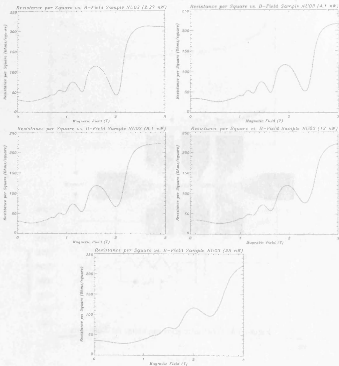
Figure 5.5: Shubnikov de Haas oscillations in Nottingham sample dissipating constant powers. Note the dampening of the oscillations at the higher power levels. This is due to the higher temperature of the 2DEG electrons.
