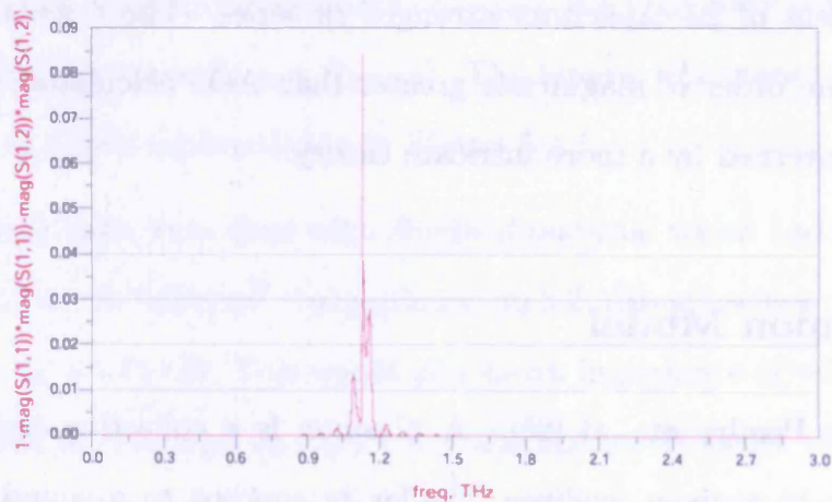
Figure 5.13: The FTS test of the meander structure on the Sheffield 2DEG showed an absorption peak at \approx 1.1\text{THz} (a.). We modeled the system with ADS including a value for the capacitance of the meander structure and made an absorption curve (b.), matching the absorption peak and thus determining the capacitance of the meander.
