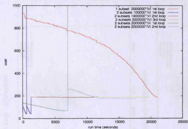
Figure 7.25: Cost-time plot for Bradford10 with balanced GPFAP decomposition into two subsets for 4,000,000 * |V| evaluations with preprocessing approach.
