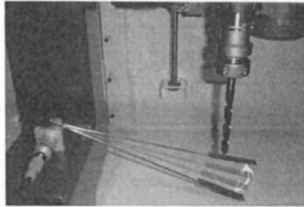
Figure 3.3: Contact-type tool breakage detection systems (adopted from [3.51])
