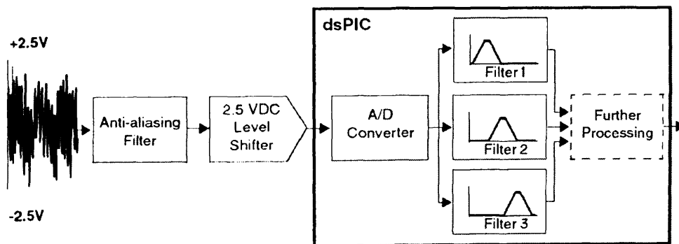
Figure 6.3: Signal processing system using multiple filters
