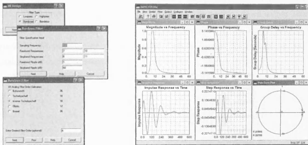
(b) Main Screen with generated graphs
