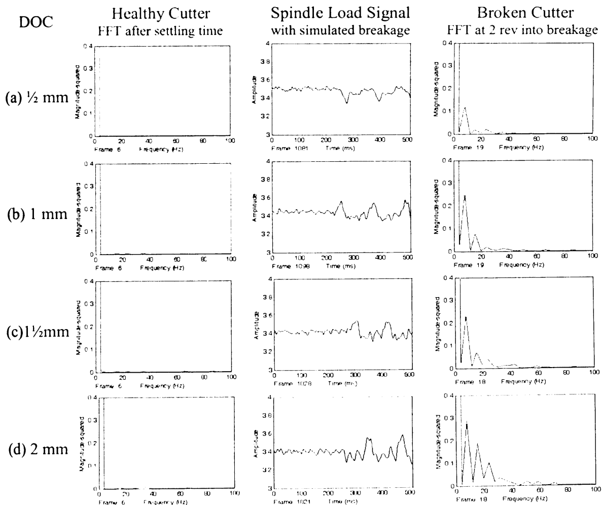
Figure 5.14: 256 pt FFT Analysis for cutting tests at different DOC
