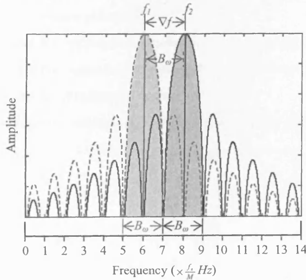
Figure 5.8: Two rectangular window transforms displaced by \Delta f = \frac{2f_s}{M} Hz
