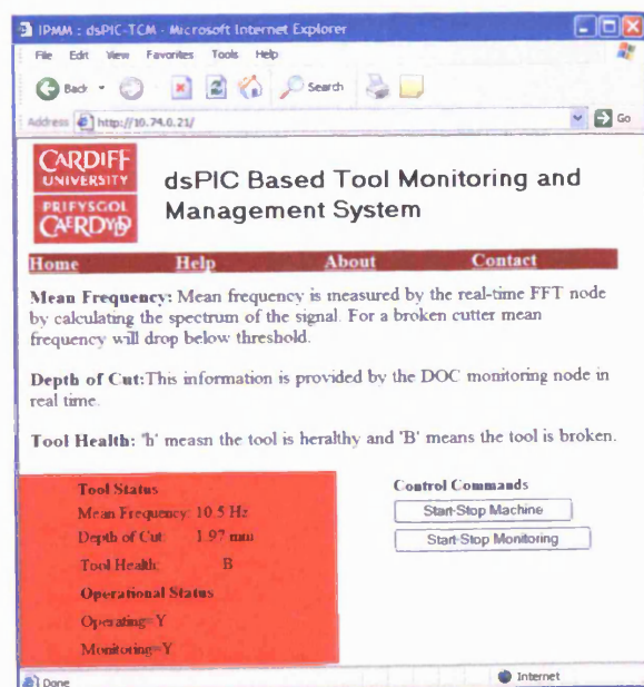
Figure 8.3(b): Webpage information for a healthy cutter
