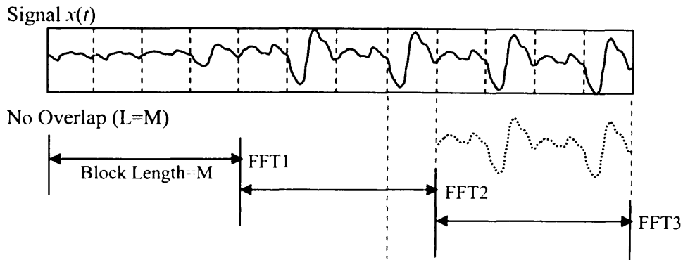
Figure 5.3 (a): STFT with no overlap
