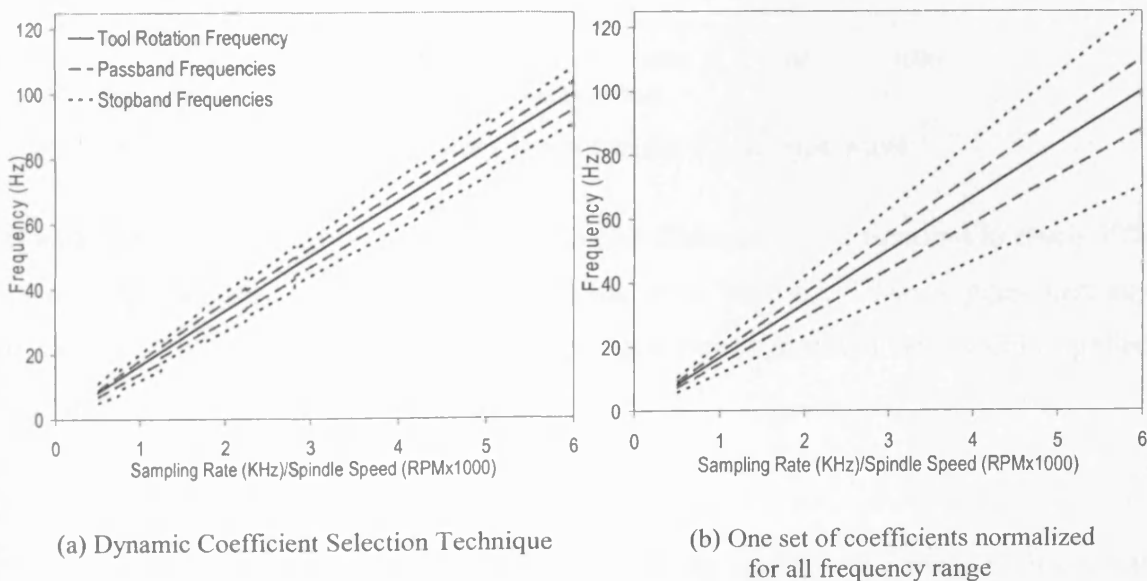
Figure 6.8: Filter Frequencies (Bandwidth) of the IIR Filter
