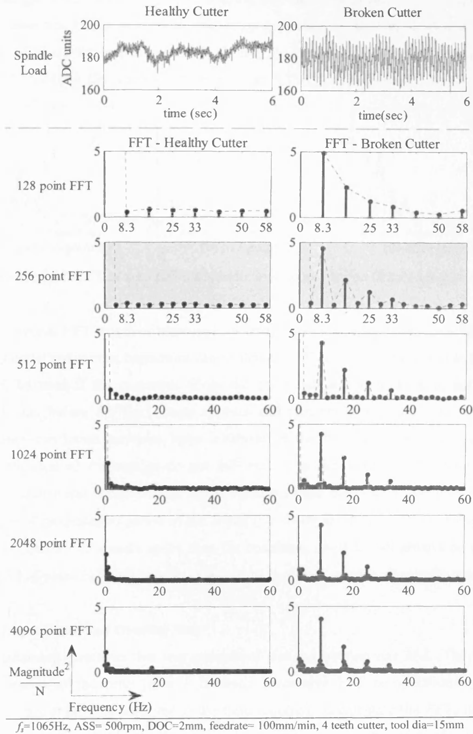
(Left: Healthy Cutter, Right: Broken Cutter, Row 1: Spindle Load, Row 2 to7: FFT) Figure 5.10: Comparison of Spindle Load Signal for different FFT Lengths (N)
