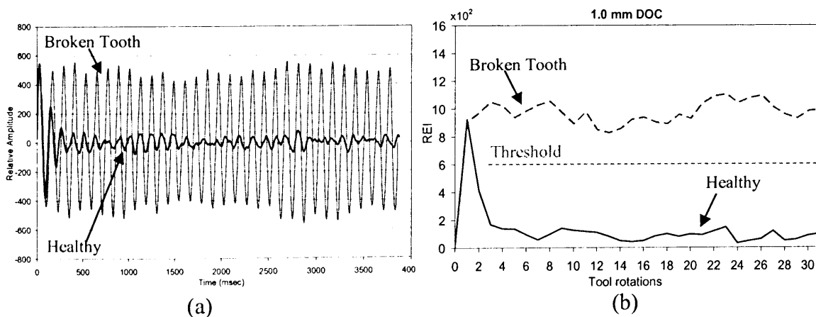
Figure 6.14: (a) The filter output for a healthy and broken cutter at 1 mm depth of cut. (b) REI at 1 mm depth of cut.
