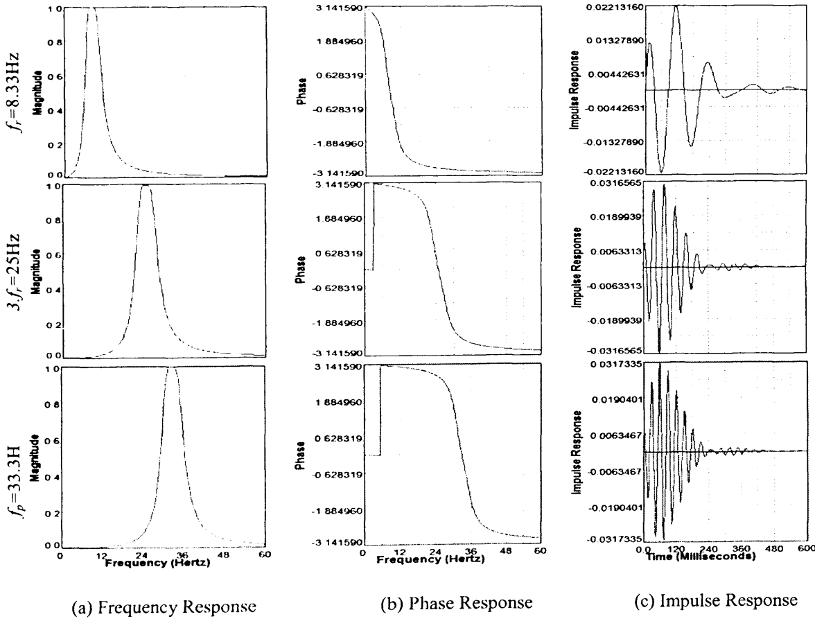
Figure 6.6: IIR Filter/System Response at 500sps (for Spindle Speed = 500rpm)
