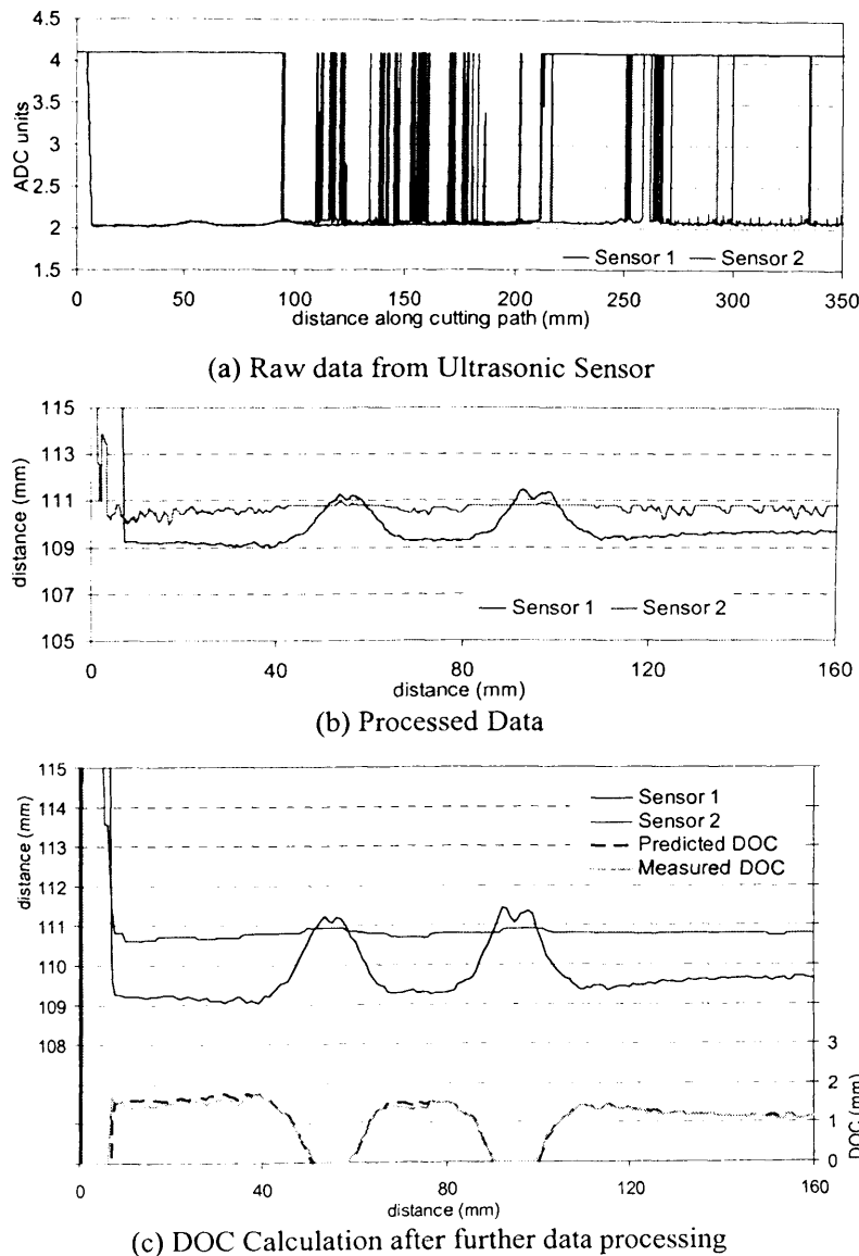
Figure 7.25: Depth of Cut Measurement for Cutting Test with 1.5 mm DOC
