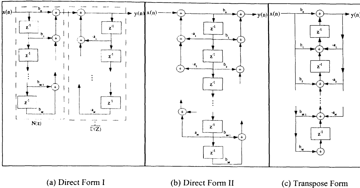
Figure 6.2: IIR Filter Structures (adopted from [6.4])
