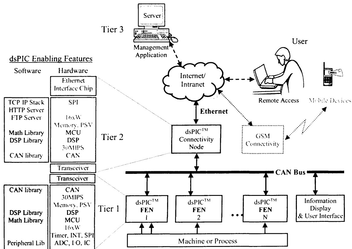
Figure 4.1: Hardware architecture of proposed monitoring system.
