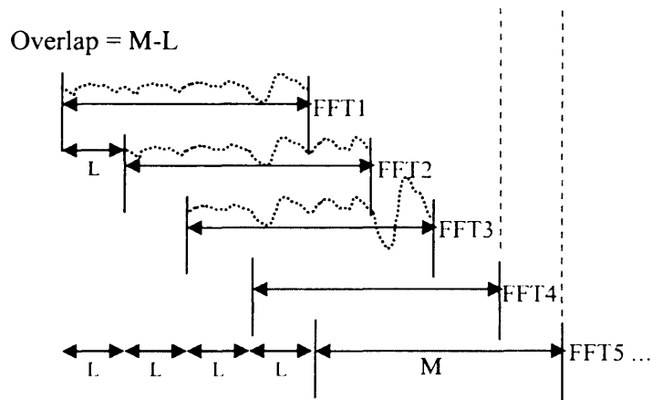
Figure: 5.3 (b) Overlap FFT
