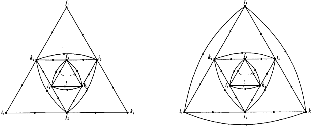
Figure 4.9: Labels for the vertices of \mathcal{D}^{(2n+1)*} and \mathcal{D}^{(2n)*}
