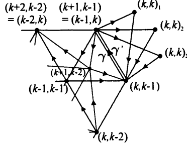
Figure 4.6: Labels for the graph \mathcal{D}^{(3k+3)}
