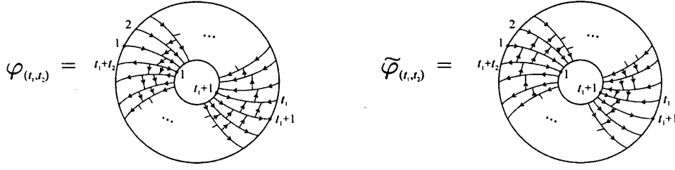
Figure 6.51: \varphi_{(t_1, t_2)} and \tilde{\varphi}_{(t_1, t_2)}
