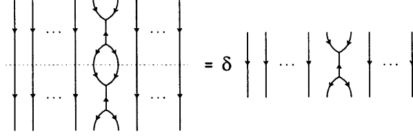
Figure 6.5: w_i^2 = \delta w_i
