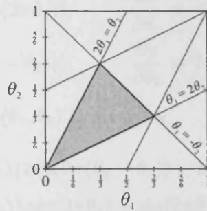
Figure 7.10: A fundamental domain C of \mathbb{T}^2/G .
