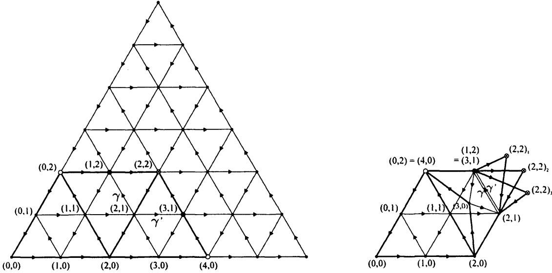
Figure 4.5: \mathcal{A}^{(9)} and its \mathbb{Z}_3 orbifold \mathcal{D}^{(9)}
