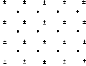
Figure 2.2: Ising Configuration Space
