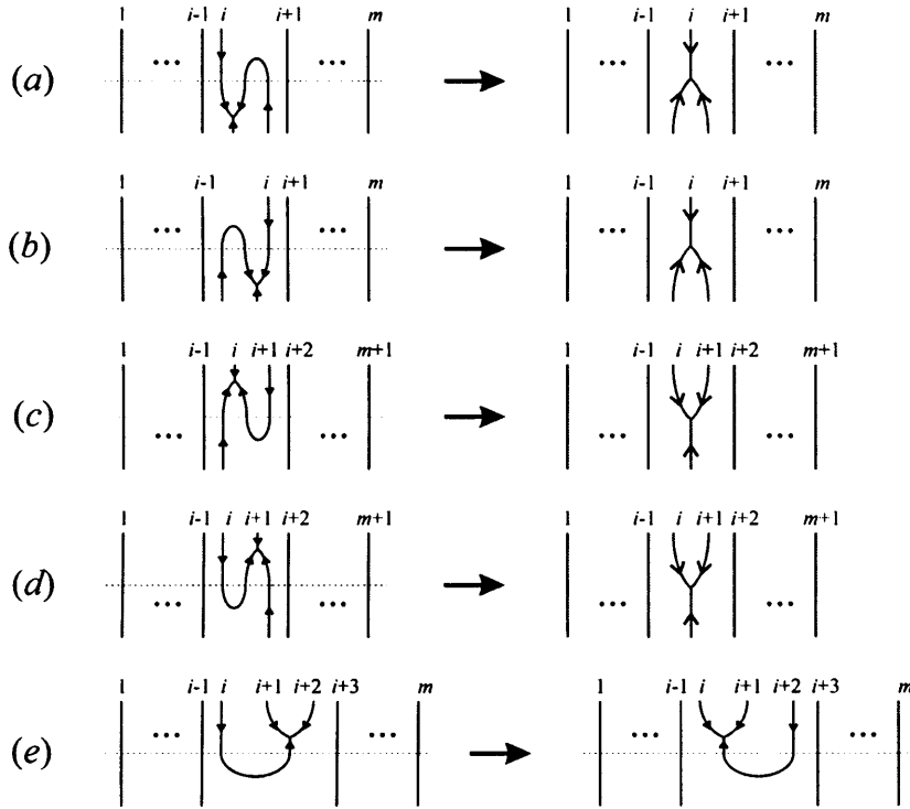
Figure 6.39: Isotopies involving an incoming trivalent vertex
