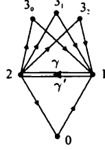
Figure 4.8: Labelling the graph \mathcal{D}^{(6)}
