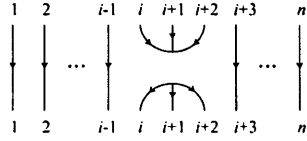
Figure 6.8: The m -tangle F_i , i = 1, \dots, m-2 .
