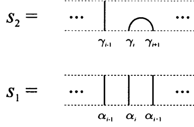
Figure 6.45: Horizontal strips s_1, s_2
