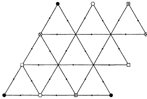
Figure 7.15: \mathbb{Z}_{n-2} \times \mathbb{Z}_{n-2} for n = 6 ; vertices which have the same symbol are identified.
