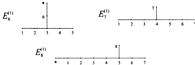
Figure 7.6: Affine Dynkin diagrams E_6^{(1)} , E_7^{(1)} and E_8^{(1)}
