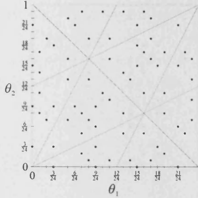
Figure 7.13: The points (\theta_1, \theta_2) \in \{g(\lambda) \mid \lambda \in \text{Exp}, g \in G\} for \mathcal{E}^{(8)} .
