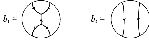
Figure 6.22: Discs b_1 and b_2
