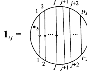
Figure 6.26: Identity Tangle 1_{i,j}
