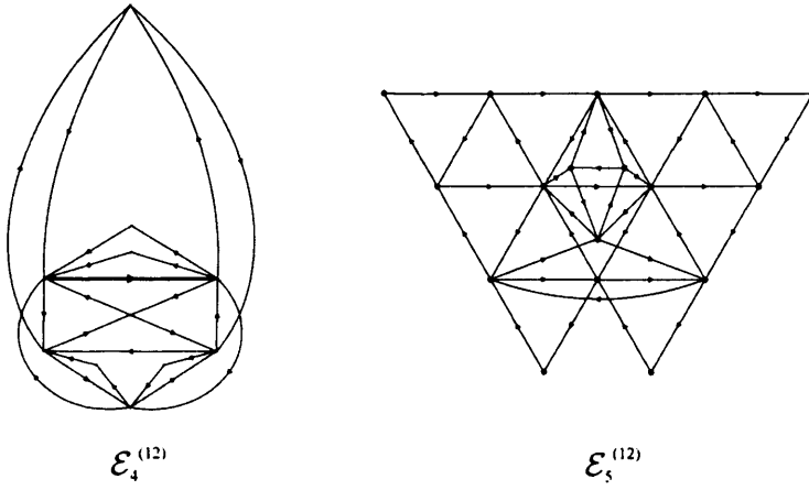
Figure 1.14: Moore-Seiberg graph \mathcal{E}_5^{(12)} and conjugate Moore-Seiberg graph \mathcal{E}_4^{(12)}
