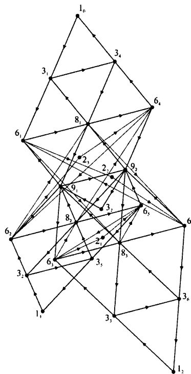
Figure 7.19: (G) = \sum(216 \times 3)
