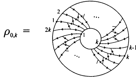
Figure 6.52: “Rotation” tangle \rho_{0,k}
