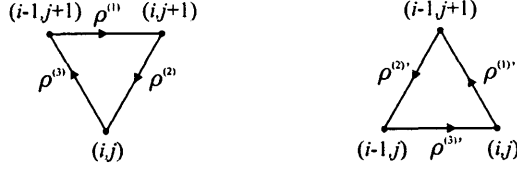
Figure 4.7: Triangles \Delta_{(i,j),(i-1,j+1),(i,j+1)}^{(\rho^{(1)},\rho^{(2)},\rho^{(3)})} and \Delta_{(i-1,j),(i,j),(i-1,j+1)}^{(\rho^{(1)'},\rho^{(2)'},\rho^{(3)'})}
