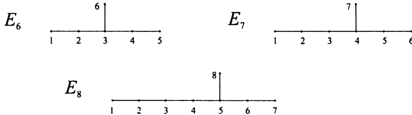
Figure 1.3: Dynkin diagrams E_6 , E_7 and E_8
