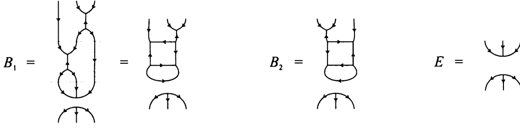
Figure 6.3: 3-tangles B_1 , B_2 , E
