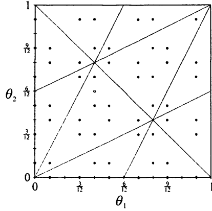
Figure 7.14: The points (\theta_1, \theta_2) \in \{g(\lambda) \mid \lambda \in \text{Exp}, g \in G\} for \mathcal{E}_1^{(12)} . The white circle indicates is the point (5/12, 6/12) .
