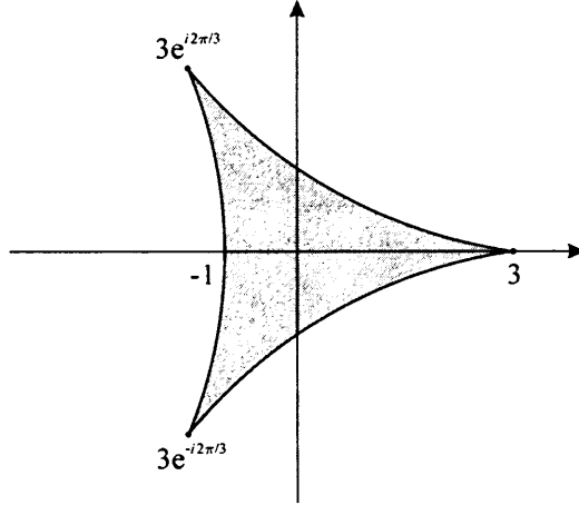
Figure 7.8: The set \mathfrak{D} , the closure of the interior of a deltoid.
