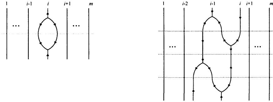
Figure 6.41: Tangles for checking K2 and K3
