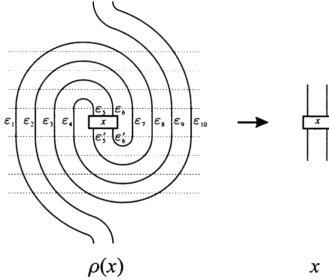
Figure 6.44: Rotation of internal rectangles by 2\pi
