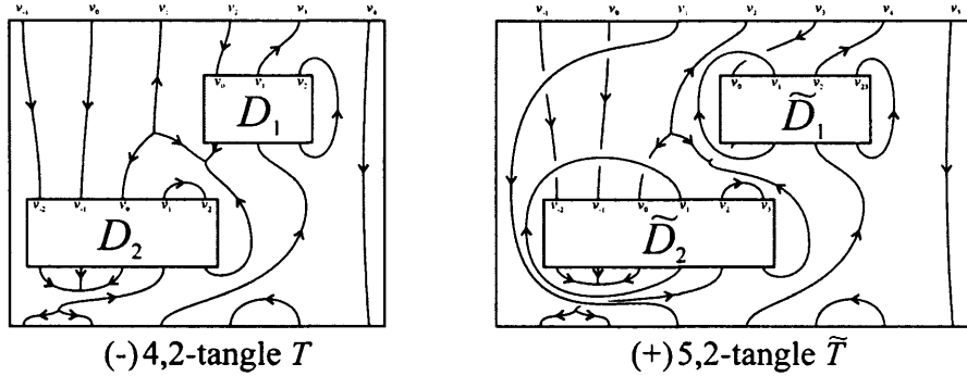
Figure 6.31: T \rightarrow \tilde{T} for duality
