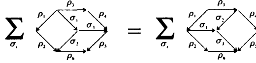
Figure 1.5: The Yang-Baxter equation
