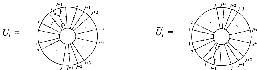
Figure 6.53: Annular i, j -tangles U_l, \tilde{U}_l, l = 1, \dots, j
