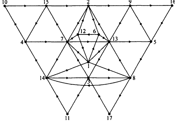
Figure 4.11: Labelled graph \mathcal{E}_5^{(12)}
