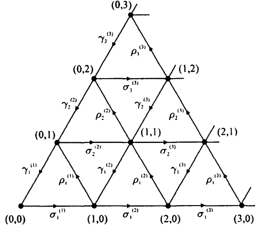
Figure 4.4: Labels for the vertices and edges of \mathcal{A}^{(n)}
