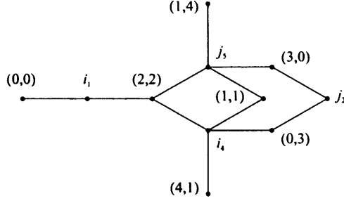
Figure 5.2: Principal graph for the A_2 Goodman-de la Harpe-Jones subfactor for \mathcal{E}^{(8)}
