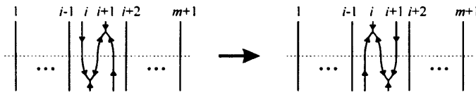
Figure 6.40: An isotopy involving an incoming and outgoing trivalent vertex
