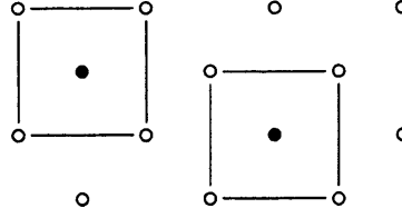
Figure 2.6: A Hard square configuration
