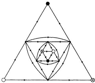
Figure 7.16: \mathbb{Z}_p \times \mathbb{Z}_3 for p = 3 .
