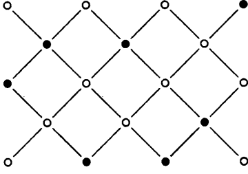
Figure 2.5: An Ising model configuration
