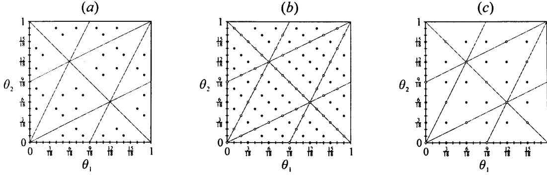
Figure 7.27: (a) the points \{g(\theta_1, \theta_2) | g \in G\} for j = 10, \dots, 15 ; (b) the points (\theta_1, \theta_2) such that (e^{2\pi i \theta_1}, e^{2\pi i \theta_2}) \in D_3 ; (c) the points (\theta_1, \theta_2) such that e^{2\pi i \theta_k} is a 6 th root of unity, k = 1, 2 .
