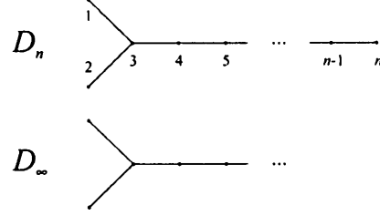
Figure 1.2: Dynkin diagrams D_n , n = 4, 5, \dots , and D_\infty
