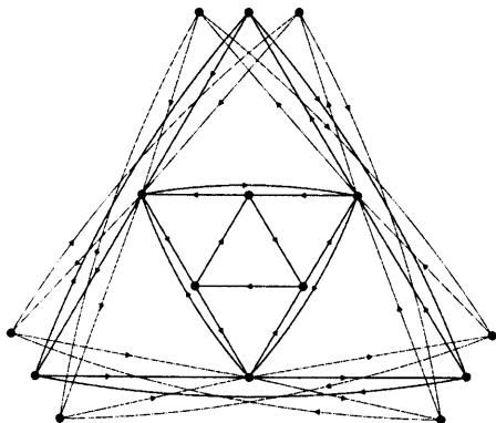
Figure 7.20: \widehat{\mathcal{D}}_4 \otimes \sigma_{123}
