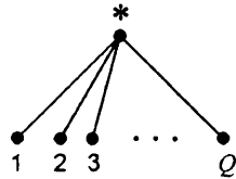
Figure 2.4: Q -State Potts Model
