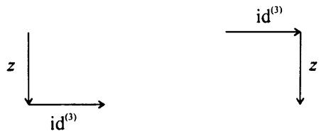
Figure 6.33: z \cdot \text{id}^{(3)} and \text{id}^{(3)} \cdot z'
