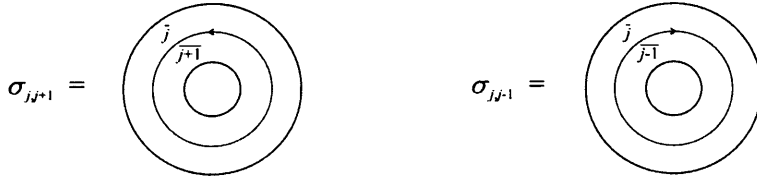
Figure 6.50: \sigma_{j,j+1} and \sigma_{j,j-1}
