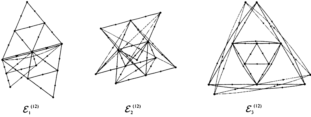
Figure 1.13: \mathcal{E}_1^{(12)} , \mathcal{E}_2^{(12)} and the virtual graph \mathcal{E}_3^{(12)}
