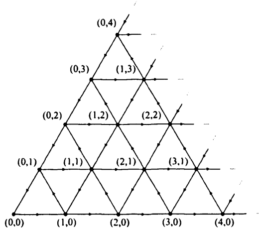
Figure 1.7: The infinite SU(3) fusion graph \mathcal{A}^{(\infty)}
