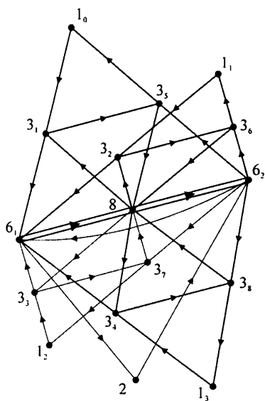
Figure 7.18: (F) = \sum(72 \times 3)
