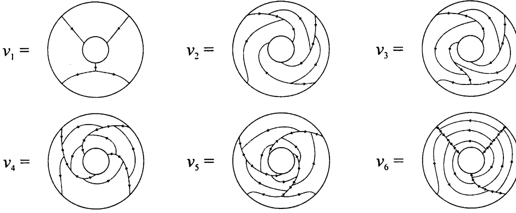
Figure 6.54: The basis elements v_i , i = 1, \dots, 6 , of V_{0,2}^{(3,0),\gamma}
