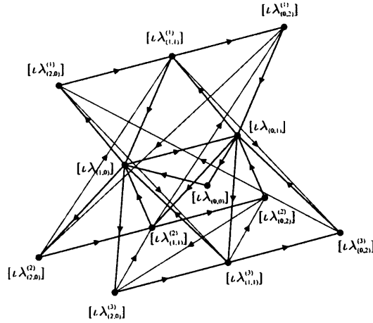
Figure 5.3: M - N graph for the \mathcal{E}_2^{(12)} A_2 -GHJ subfactor
