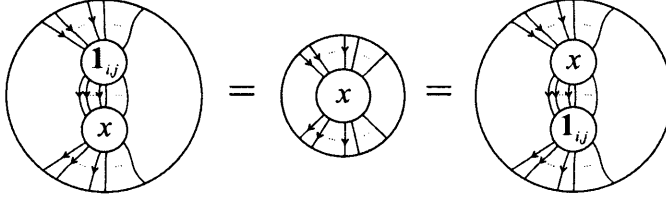
Figure 6.27: Z(1_{i,j})x = x = xZ(1_{i,j})
