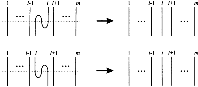
Figure 6.38: Two cup-cap simplifications
