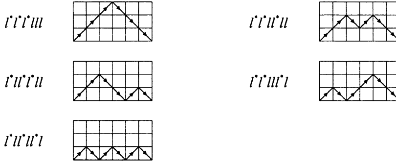
Figure 7.2: Catalan paths of length 6
