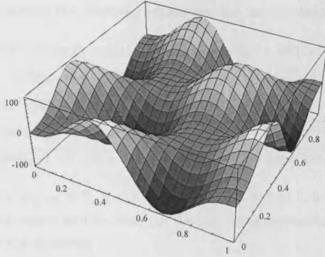
Figure 7.11: The Jacobian J .
