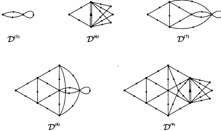
Figure 1.9: \mathcal{D}^{(n)} for n = 5, 6, 7, 8, 9
