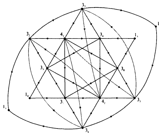
Figure 7.17: (E) = \sum(36 \times 3)
