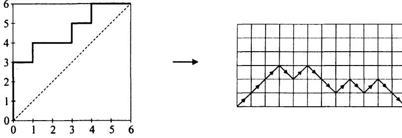
Figure 7.3: Increasing path and corresponding Catalan path for (e_3e_2e_1)(e_4e_3)(e_5e_4) .
