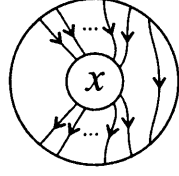
Figure 5.1: \iota(x) for x \in M_k
