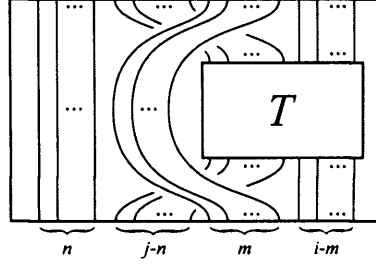
Figure 6.24: A tangle in \mathcal{P}_{i,j}^{(m,n)}
