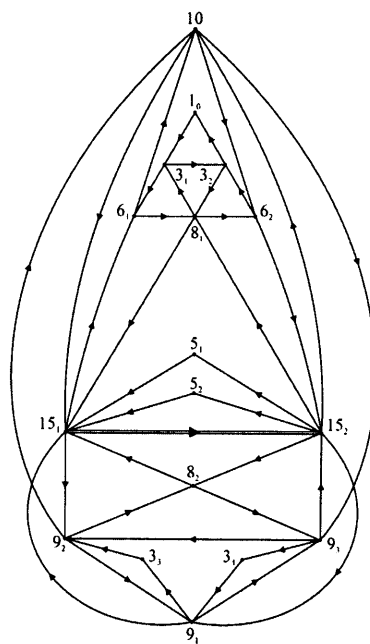
Figure 7.21: (L) = \sum(360 \times 3)
