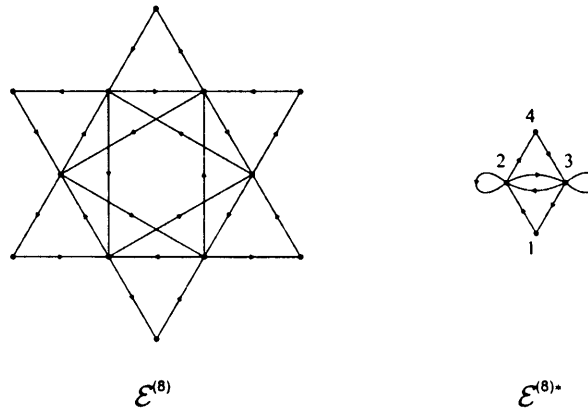
Figure 1.12: \mathcal{E}^{(8)} and its \mathbb{Z}_3 orbifold \mathcal{E}^{(8)*}
