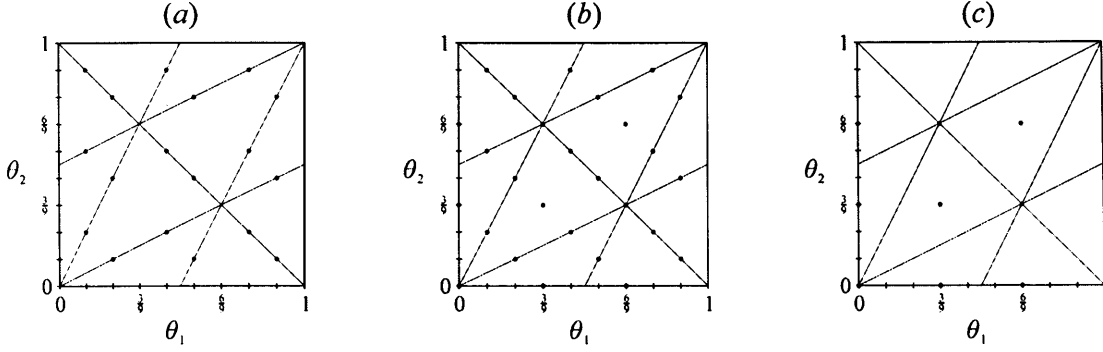
Figure 7.26: (a) the points \{g(\theta_1, \theta_2) | g \in G\} for j = 4, \dots, 9 ; (b) the points (\theta_1, \theta_2) such that (e^{2\pi i \theta_1}, e^{2\pi i \theta_2}) \in D_{3/2} ; (c) the points (\theta_1, \theta_2) such that e^{2\pi i \theta_k} is a 3 rd root of unity, k = 1, 2 .
