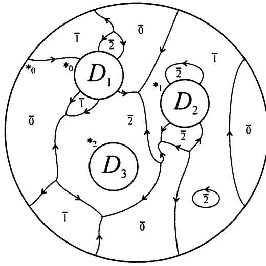
Figure 6.19: A_2 -planar tangle
