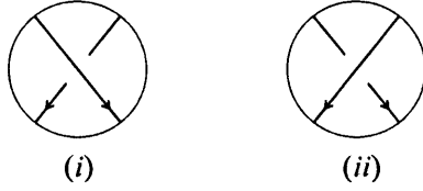
Figure 6.21: Disc b for (i) negative crossing, (ii) positive crossing
