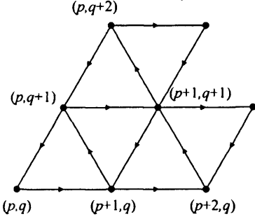
Figure 4.3: Triangles in \mathcal{A}^{(n)}
