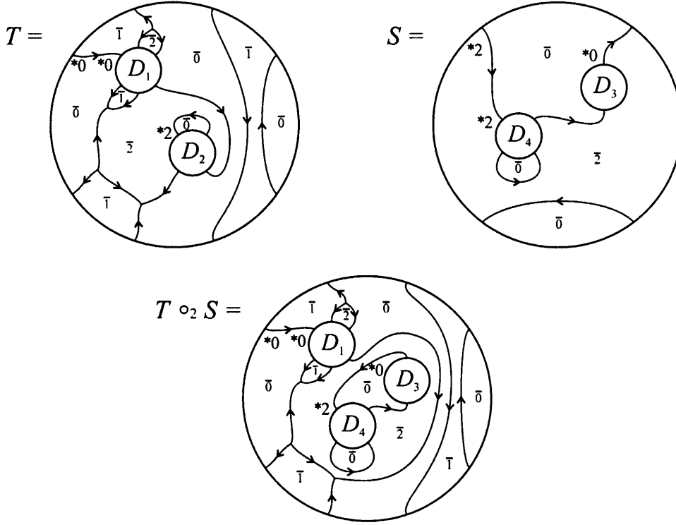
Figure 6.20: Composition of planar tangles
