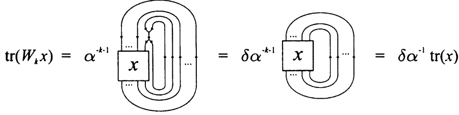
Figure 6.18: Markov trace on V^{A_2}
