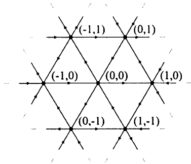
Figure 7.7: The infinite graph \mathcal{A}^{(\infty)6} .
