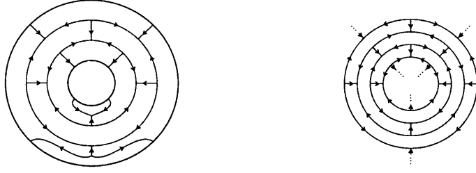
Figure 6.48: A basis A_2 -annular (2, 0 : 2, 0) -tangle containing hexagons, and the possibility of an infinite number of hexagons
