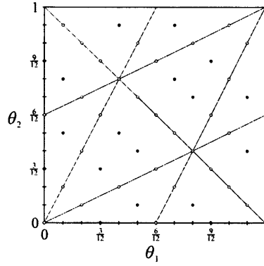
Figure 7.28: The points (\theta_1, \theta_2) such that (e^{2\pi i \theta_1}, e^{2\pi i \theta_2}) \in D_2 .
