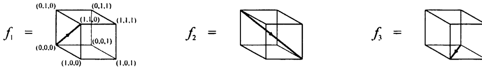
Figure 7.12: The vectors f_i \in \mathbb{Z}^3 , i = 1, 2, 3 .
