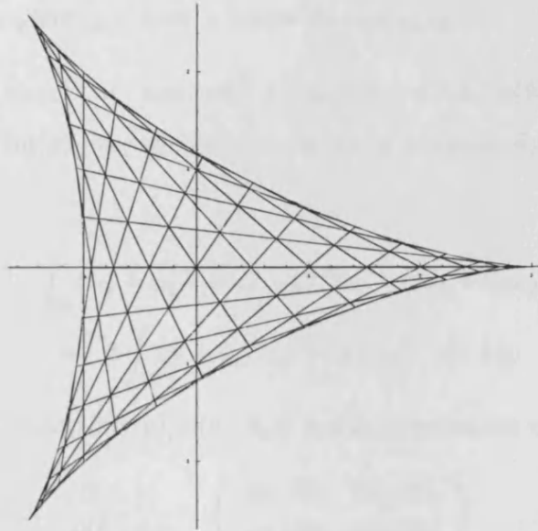
Figure 7.9: Mapping \mathbb{T}^2 onto the deltoid \mathfrak{D} .
