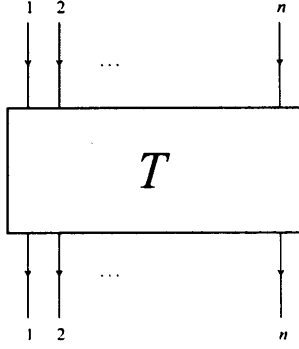
Figure 6.9: m -tangle T
