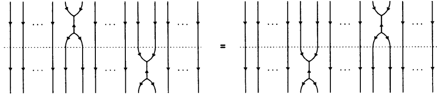
Figure 6.6: w_i w_j = w_j w_i for |i - j| > 1 .
