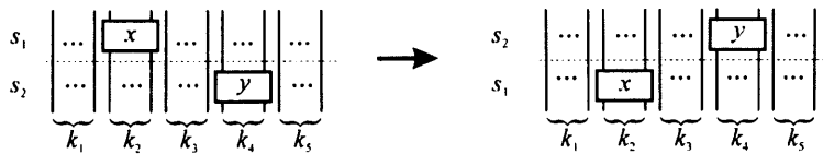
Figure 6.43: An isotopy involving two rectangles
