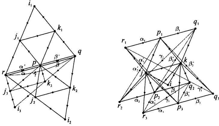
Figure 4.10: \mathcal{E}_1^{(12)} and \mathcal{E}_2^{(12)}
