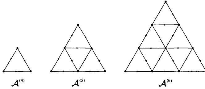
Figure 1.8: \mathcal{A}^{(n)} for n = 4, 5, 6
