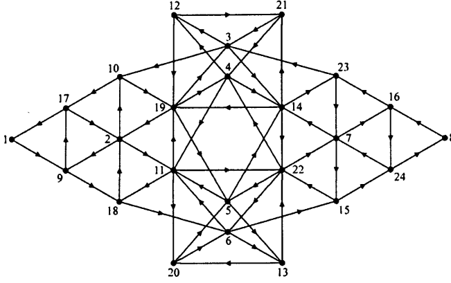
Figure 4.12: Labelled graph \mathcal{E}^{(24)}
