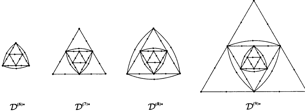
Figure 1.11: \mathcal{D}^{(n)*} for n = 6, 7, 8, 9
