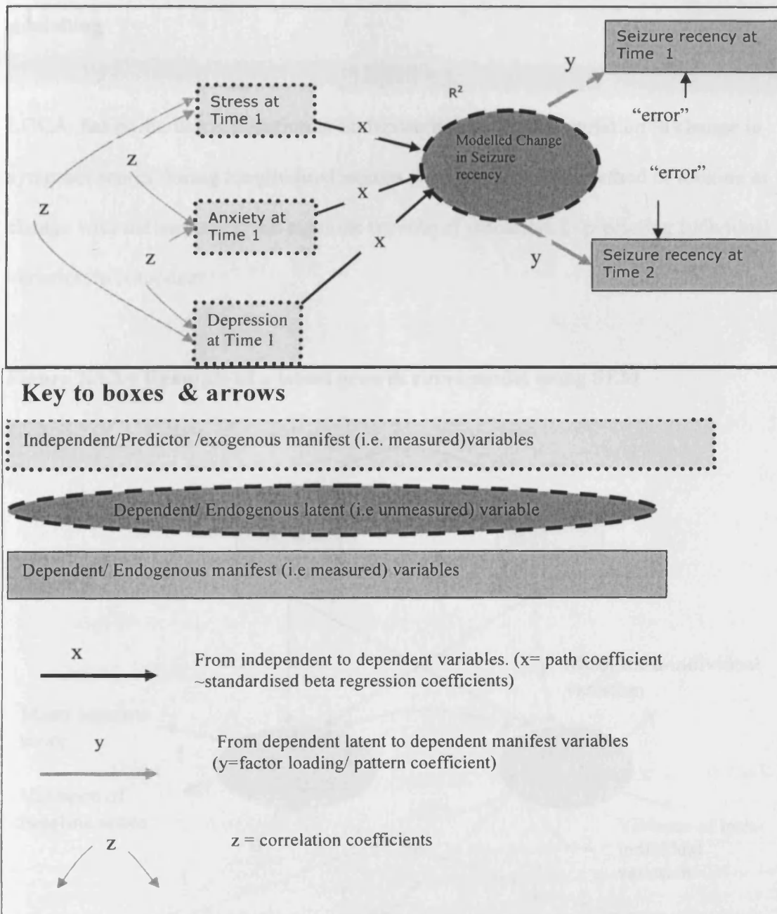
Figure 2.3.3.3: An example of a random effects structural equation model .
