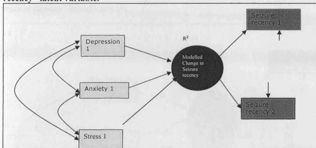
Figure 1: General form of the structural equation model with “change in seizure recency” latent variable.
