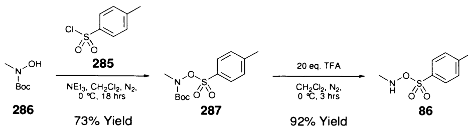
Reaction scheme 7.1: Synthesis of achiral tosyl reagent 86 . 53
