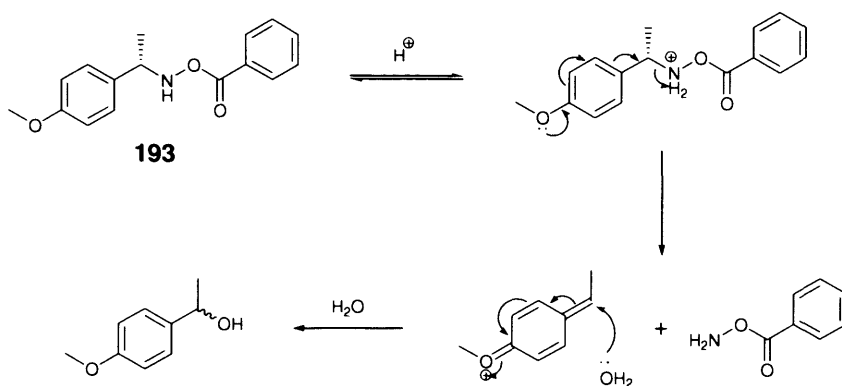
Reaction scheme 4.4: Possible acid decomposition of reagent 193.
