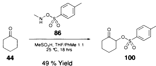
Reaction scheme 7.2: Synthesis of racemic \alpha -oxytosyl cyclohexanone 100 .
