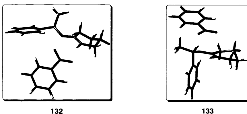
Figure 3.1: Possible transition states for asymmetric transformation generated using computer modeling.
