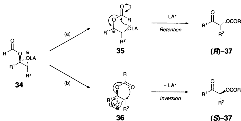
Reaction scheme 1.10: Proposed mechanisms for competing reaction pathways, leading to opposite enantiomers of the product 37. 28
