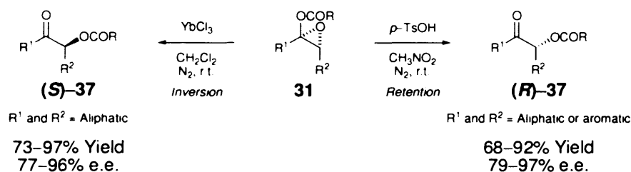
Reaction scheme 1.11: Rearrangement of chiral enol ester epoxides 31 to \alpha -acyloxy ketones 37.
