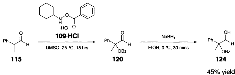
Reaction scheme 2.6: \alpha -Oxybenzoylation of 2-phenyl propionaldehyde 115, followed by reduction to alcohol 124.
