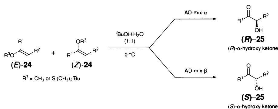
Reaction scheme 1.6: Application of the AD of enol ethers (24) to the synthesis of chiral α-hydroxy ketones (25). 20
