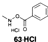
Figure 1.7: Novel reagent for the \alpha -oxybenzoylation of carbonyl compounds.
