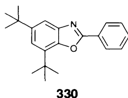
Figure 8.3: Benzoxazole product resulting from reaction of benzaldehyde.
