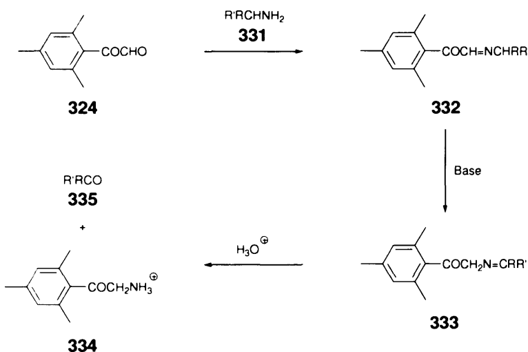
Reaction scheme 8.5: Synthesis of carbonyl compounds using mesitylgyoxal 324.
