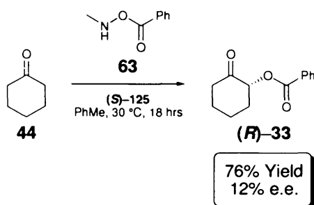
Reaction scheme 2.10: Reaction of achiral reagent 63 with (S)-CSA (S)-125.
