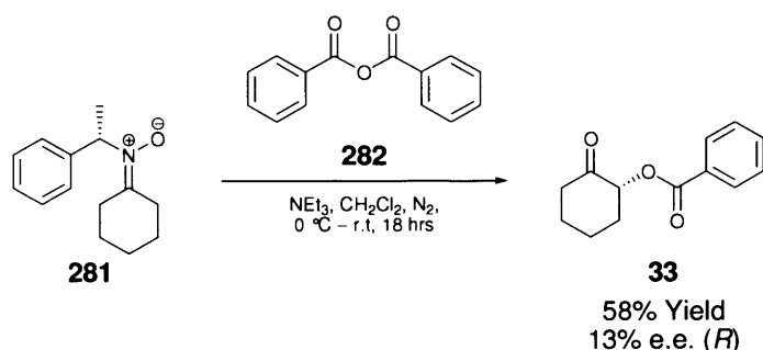
Reaction scheme 6.12: Reaction of nitron 281 with benzoic anhydride 282 .
