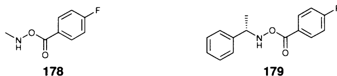
Figure 4.1: Reagents synthesised using 4-fluorobenzoic acid.
