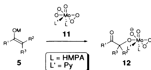
Reaction scheme 1.3: \alpha -Oxygenation using \text{MoOPH} 11 involving transfer of a peroxidic oxygen.
