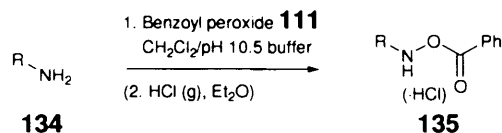
Reaction scheme 3.1: Traditional method used for reagent synthesis. 55
