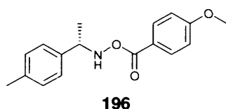
Figure 4.9: Electron-rich chiral reagent designed to maximize electronic effects.
