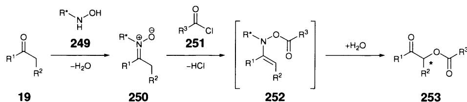
Reaction Scheme 6.1: General reaction for the \alpha -oxygenation of carbonyl compounds, employing the use of nitrones.
