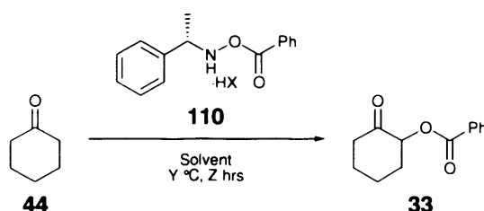
Reactions Scheme 2.7: Reaction of cyclohexanone 44 with chiral reagent 110 , illustrating variables.
