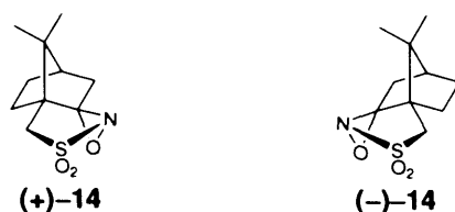
Figure 1.4: Structures of (+)- and (-)-(camphorylsulphonyl)oxaziridine.
