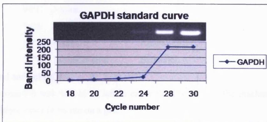
Figure 2.3 Graph showing GAPDH standard curve with corresponding PCRs.
