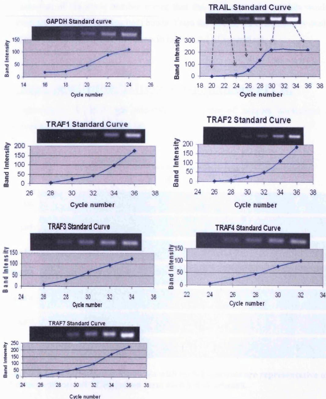
Figure 3.2 Shows PCR standard curves for selected genes. In the TRAIL standard curve the arrows from the bands point to their corresponding points in the graph.
