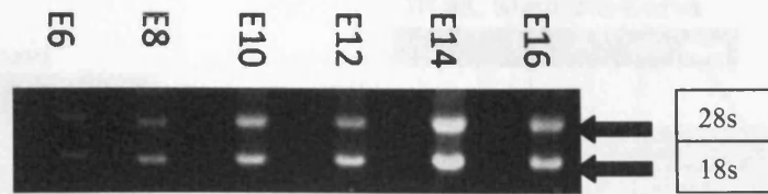
Figure 3.1 Image of RNA denaturing gel.
