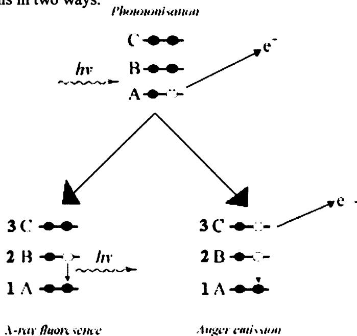
Fig. 2.5 Neutralising the core hole
