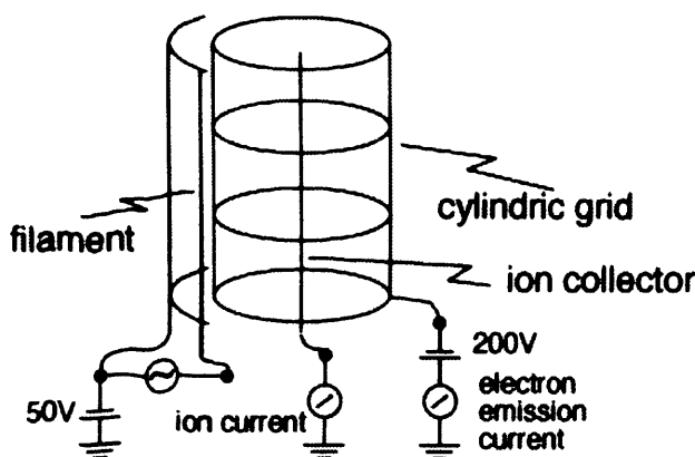
Figure 4.5 Schematic of a Bayard-Alpert ion gauge.
