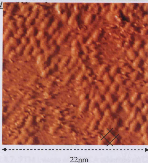
Fig. 8.6: STM images of BPDCA adsorbed on Cu(110) after 240 second exposure [bias: negative, voltage = 1.09V, current = 2.32nA].
