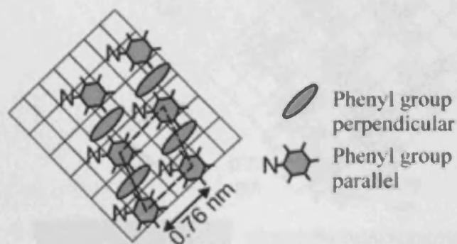
Fig. 14: A model to show the T-shaped structure formed at the surface which would result in only half the aniline molecules being imaged at the Cu(110) surface.
