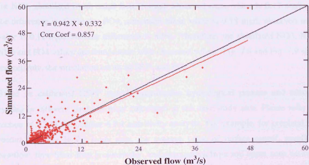
Fig. 7.6. Scatter plot of simulated and observed river flow
