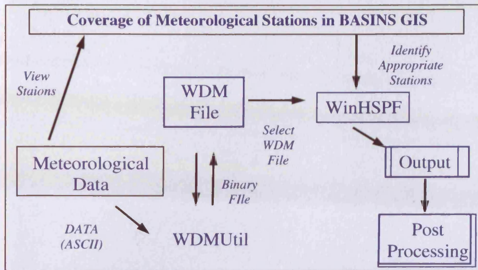
Fig. App.B.7. Processing of meteorological data in BASINS-HSPF
