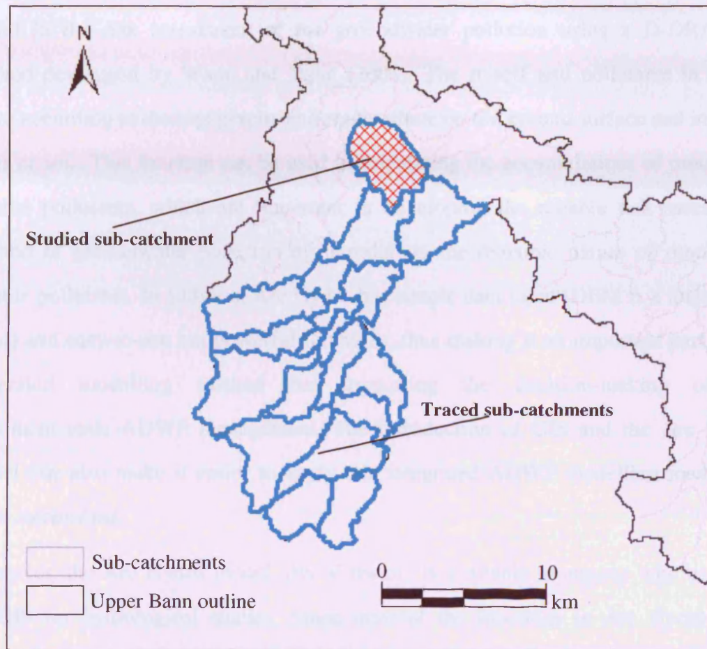
Fig. 3.7. Upstream sub-catchment tracing in the study area
