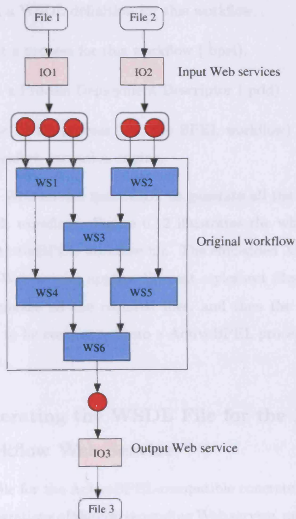
Figure 6.11: The concrete workflow with the added IO Web services.
