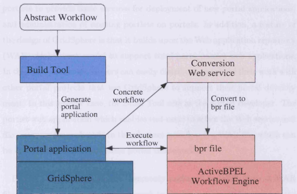
Figure 6.1: The relationship between the Build Tool and other software components.
