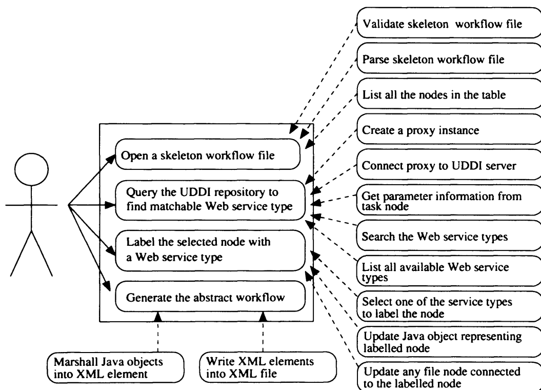
Figure 5.13: User case diagram for the Label Tool.
