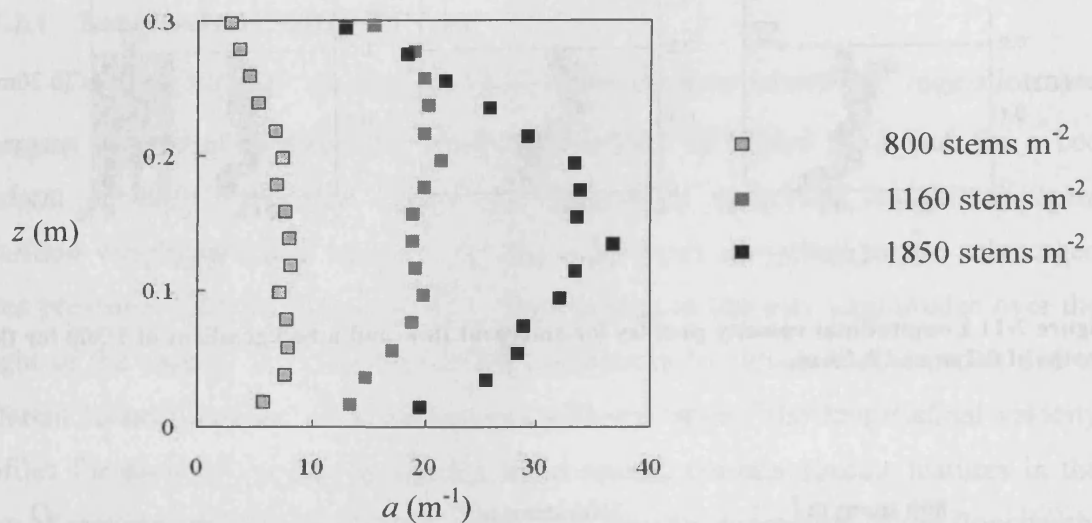
Figure 7-13 Profiles of projected area per unit volume for three Spartina anglica canopies with stem densities of 800, 1160 and 1850 stems \text{m}^{-2} . z is the elevation above the bed and a is the projected area per unit volume of the vegetation.
