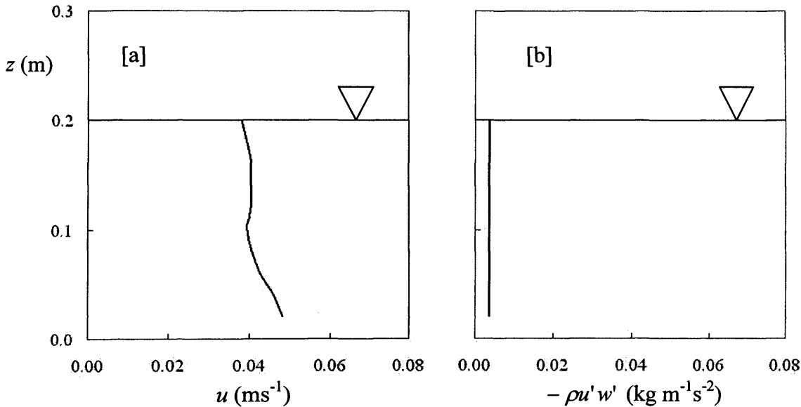
Figure 8-23 Predicted [a]: velocity and [b]: Reynolds stress profiles for a uniform flow through an emergent Spartina anglica canopy with a stem density of 1160 stems \text{m}^{-2} , for a flow depth of 0.2m and a bed gradient of 1/1000.
