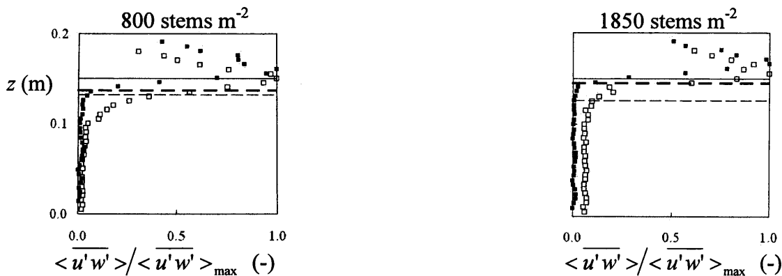
Figure 6-14 Normalised Reynolds stress profiles for submerged uniform cylinder arrays with a stem diameter of 6.0 mm ( \square ), and constructed vegetation canopies ( \blacksquare ) for a submergence level of 1.33, bed gradient of 1/300 and stem densities of 800 and 1850 stems \text{m}^{-2} . The bold dotted lines denotes Reynolds stress penetration for constructed vegetation canopies and faint dotted line denotes penetration for uniform cylinder arrays. Solid lines denote the top of the canopy.
