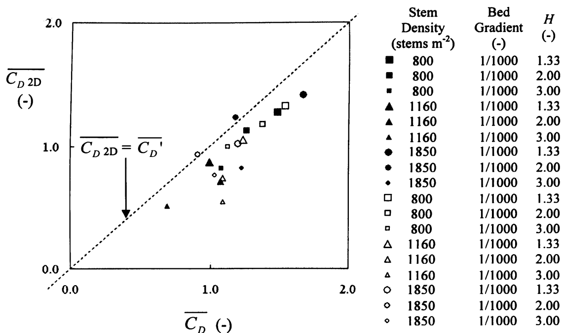
Figure 7-60 A comparison between the bulk drag coefficient, \overline{C_D} , and the depth-average of the two-dimensional drag coefficient, \overline{C_{D\ 2D}} for submerged Spartina anglica canopies for submergence levels of 1.33, 2.00 and 3.00, for August and February vegetation canopies.
