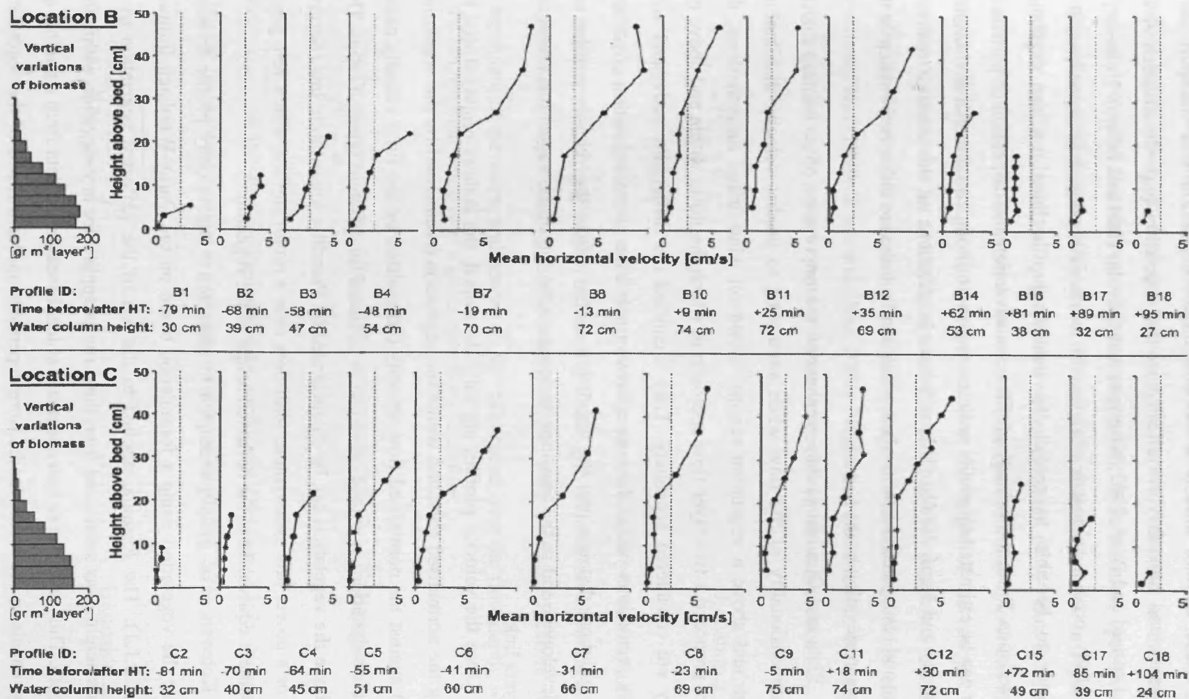
Figure 2-29 Velocity profiles through a Spartina maritima canopy at various stages during a tidal cycle. The vertical dashed lines mark the 2.5 \text{ cm s}^{-1} position (taken from Neumeier & Ciavola, 2004)
