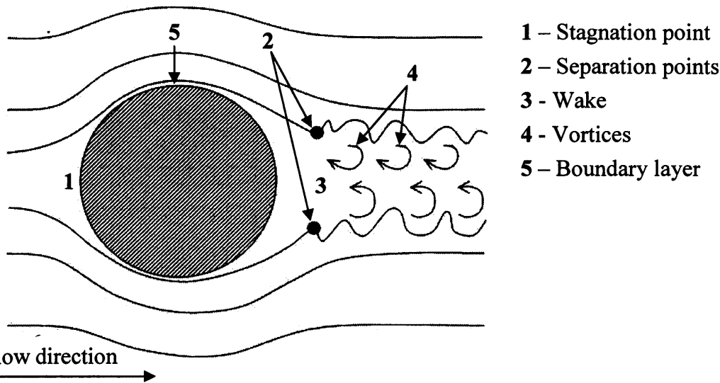
Figure 2-4 Flow structure around an immersed body (taken from Douglas et al. , 1979)
