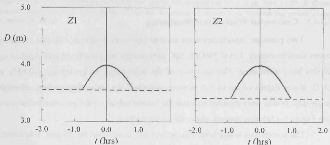
Figure 3-21 Simultaneous water level measurements at locations Z1 and Z2 during 03/05/2007 (High Tide at 19:59). Time is in hours from high tide and the depth is in metres Above Ordinance Datum. Dotted lines show the bed level for each sampling location.
