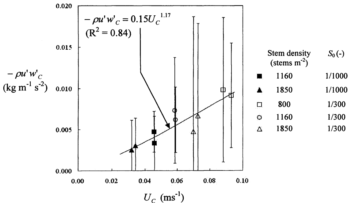
Figure 8-6 The relationship between the mean canopy Reynolds stress, -\rho u'w'_c , and the mean velocity, U_c , for emergent canopies with stem densities of 800, 1160 and 1850 stems m -2 , flow depths of 0.20m and 0.25m, and bed gradients of 1/1000 and 1/300. For each stem density and bed gradient, the higher mean Reynolds stress value corresponds to a flow depth of 0.20m, and the lower value corresponds to a flow depth of 0.25m. The vertical bars show the standard deviations.
