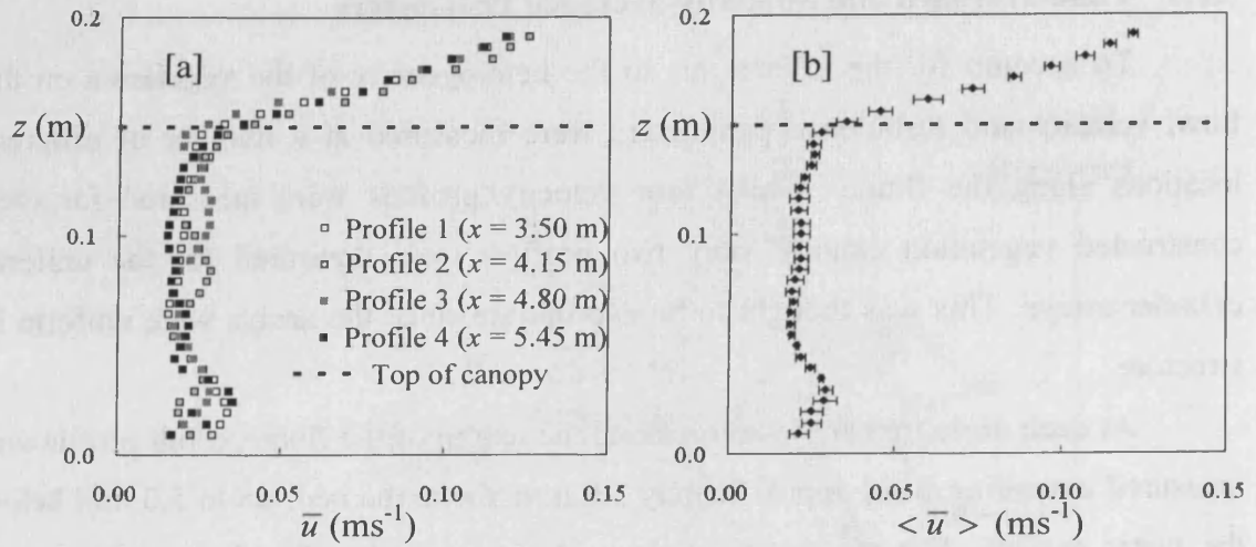
Figure 5-8 a: Single-point time-averaged and; b: double-averaged longitudinal velocities for a 1850 stems \text{m}^{-2} canopy, 0.001 bed gradient, and vegetation height of 150 mm where x is the longitudinal distance along the flume. "Bars" indicate the standard deviation of the spatial variation.
