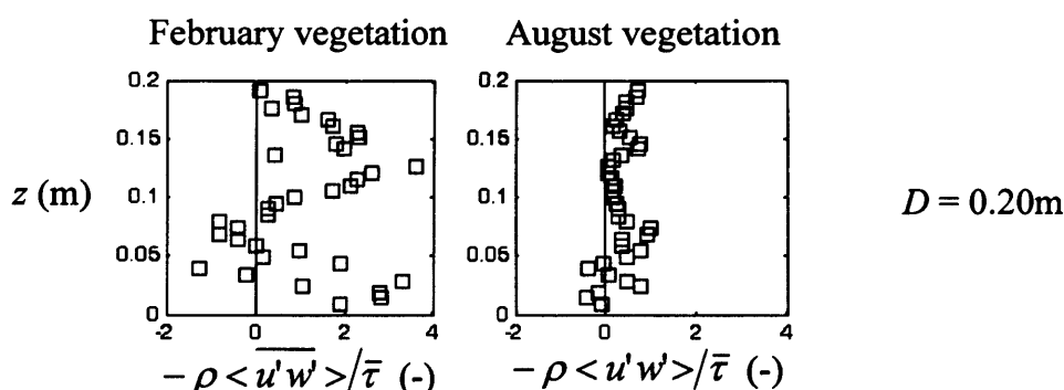
Figure 7-51 Profiles of normalised Reynolds stress (normalised by the depth-averaged total shear stress values) for emergent February and August vegetation canopies, a bed gradient of 1/1000, a stem density of 800 stem m^{-2} and a flow depth of 0.20m. \bar{\tau} is the depth-averaged total shear stress.
