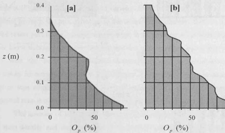
Figure 4-5 Profiles of vegetation obstruction, O_p , from [a]: Neumeier (2005) and [b]: the current study (Location A2, July 2005).
