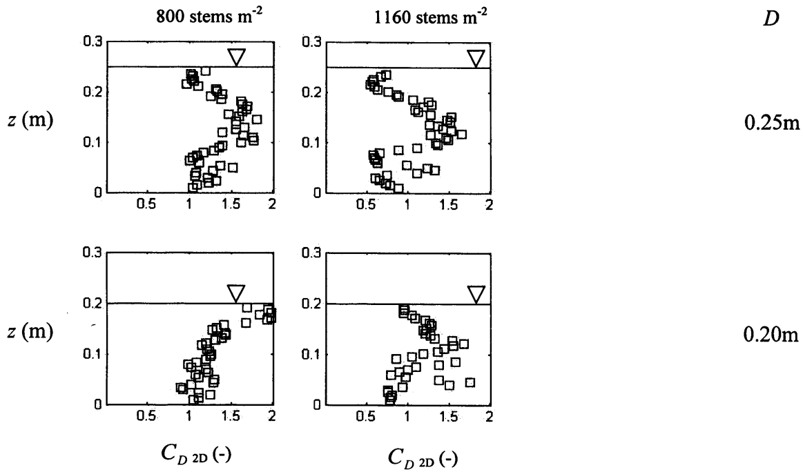
Figure 7-56 C_{D\ 2D} profiles for emergent flow conditions and a bed gradient of 1/1000 for flow depths, D , of 0.20 m and 0.25 m
