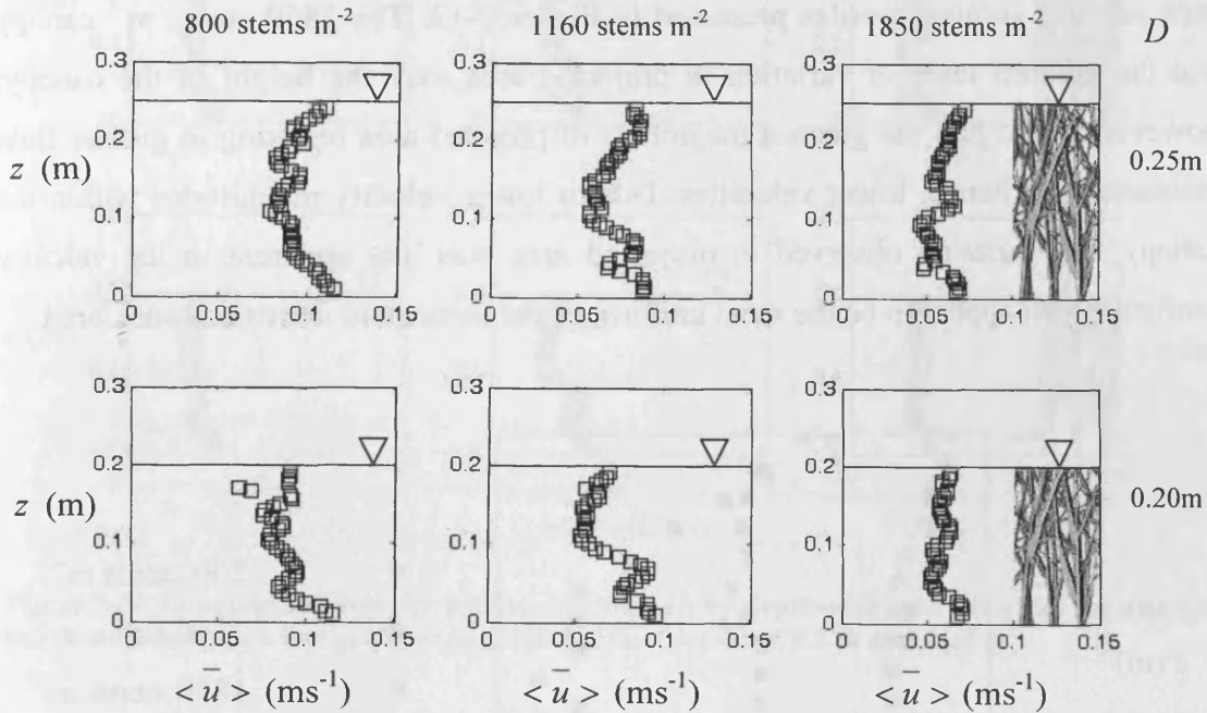
Figure 7-11 Longitudinal velocity profiles for emergent flow and a bed gradient of 1/300 for flow depths of 0.2 m and 0.25 m.
