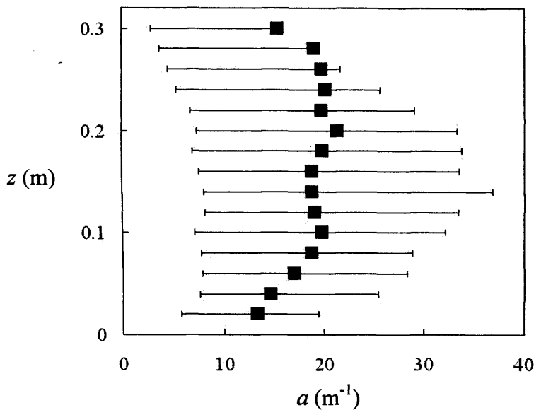
Figure 8-2 A profile of the projected area per unit volume over the canopy height for a stem density of 1160 stems \text{m}^{-2} . The error bars show the range of values encompassed by stem densities ranging between 800 and 1850 stems \text{m}^{-2} .
