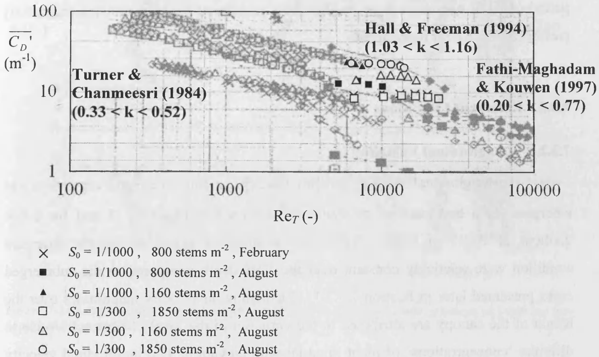
Figure 7-10 The relationship between the bulk roughness coefficient, \overline{C_D'} , and the canopy height Reynolds number, Re_T , for the emergent Spartina anglica canopies implemented in this study and some of the data presented in Tsihrintzis et al. (2001). S_0 is the bed gradient.
