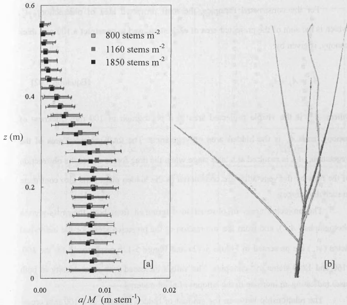
Figure 5-11 [a]: Average projected area of obstruction per stem used to construct three canopies with stem densities of 800, 1160 and 1850 stems \text{m}^{-2} to investigate variations in the degree of vegetation overlap. a is the projected area per unit volume, M is the number of stems per unit bed area, and z is the elevation above the bed. [b]: a typical Spartina anglica stem.
