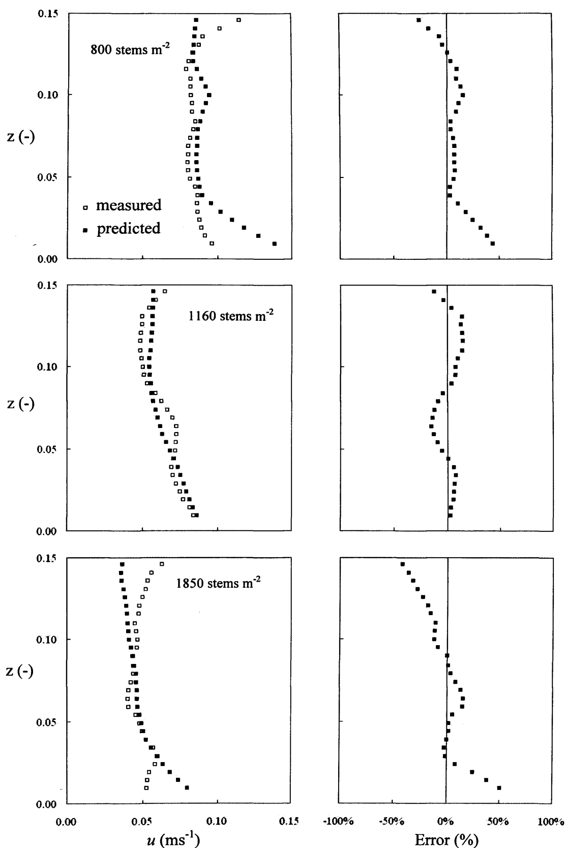
Figure 8-13 Measured ( \square ) and predicted ( \blacksquare ) longitudinal velocity profiles and the errors incurred in the predicted values for submerged Spartina anglica canopies, for stem densities of 800, 1160 and 1850 stems m -2 , a canopy height of 0.15m, a flow depth of 0.20m and a bed gradient of 1/300.
