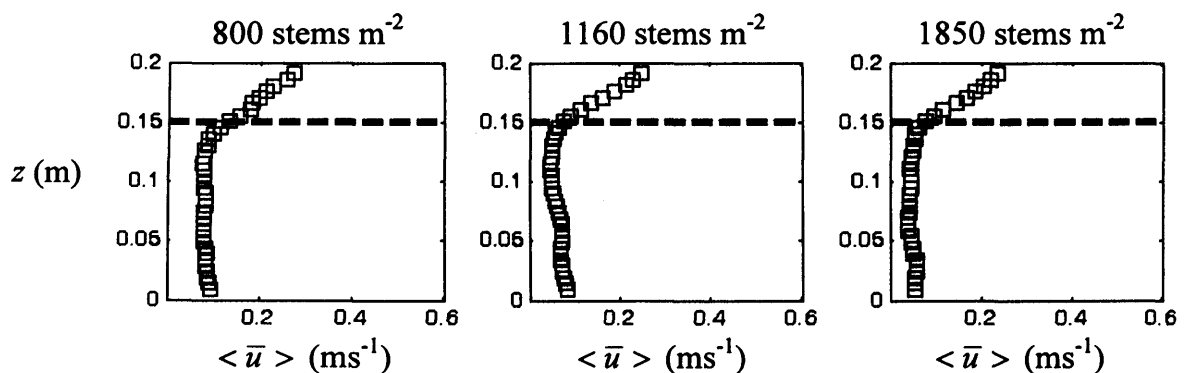
Figure 6-7 Longitudinal velocity ( u ) profiles for submerged constructed vegetation canopies for a submergence level of 1.33, a bed gradient of 1/300, stem densities of 800, 1160 and 1850 stems \text{m}^{-2} . The bold dotted lines denote top of the canopy.
