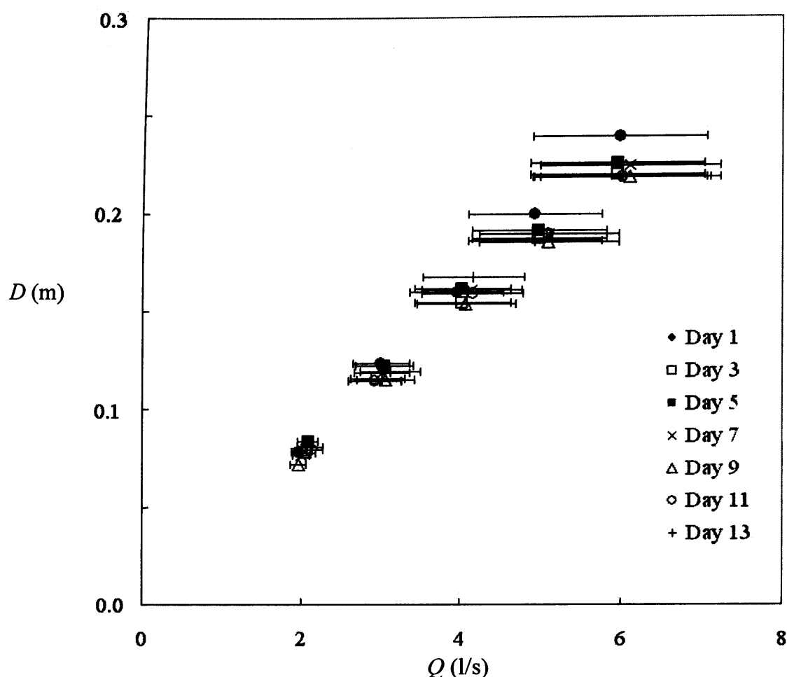
Figure 5-5 Variations in the stage-discharge relationship for an emergent, sparse Spartina anglica canopy with a stem density of 800 \text{ stems m}^{-2} over a two-week period. D is the flow depth and Q is the flow rate. Error bars indicate the errors in flow rates based on the pump reliability evaluation conducted in Section 5.2.2. The error in flow depth measurements is estimated at \pm 0.1 mm.
