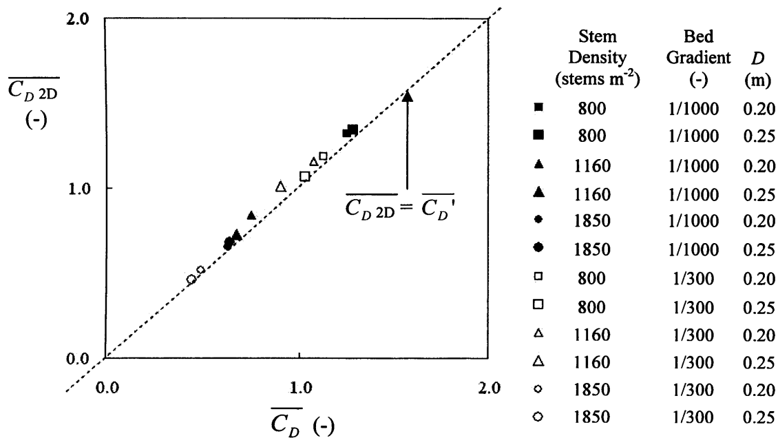
Figure 7-59 A comparison between the bulk drag coefficient, \overline{C_D} , and the depth-average of the two-dimensional drag coefficient, \overline{C_D'_{2D}} for emergent Spartina anglica canopies for flow depths of 0.20m and 0.25m, and for August and February vegetation canopies.
