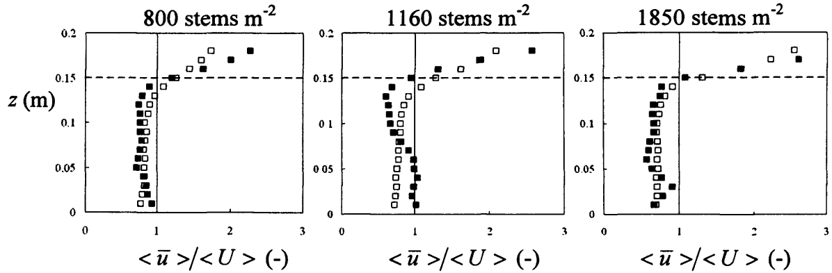
Figure 6-11 Normalised longitudinal velocity ( u ) profiles for submerged uniform cylinder arrays with a stem diameter of 6.0 mm ( \square ) and constructed vegetation canopies ( \blacksquare ), for a submergence level of 1.33, a bed gradient of 1/1000, and stem densities of 800, 1160 and 1850 stems \text{m}^{-2} . U is the depth-averaged longitudinal velocity for the flow depth. The bold dotted lines denote the top of the canopy, and the faint vertical lines denote a longitudinal velocity equal to the depth-averaged value, U .
