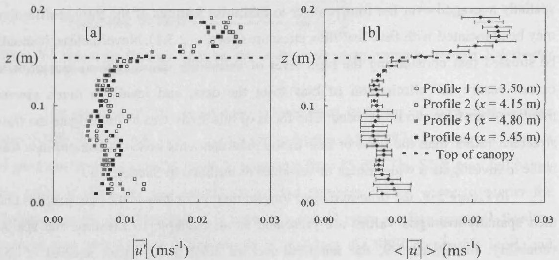
Figure 5-9 a: Single-point time-averaged and; b: double-averaged RMS values of instantaneous fluctuations in longitudinal velocities for a 1850 stems \text{m}^{-2} canopy, 0.001 bed gradient, and vegetation height of 150 mm where x is the longitudinal distance along the flume. "Bars" indicate the standard deviation of the spatial variation.
