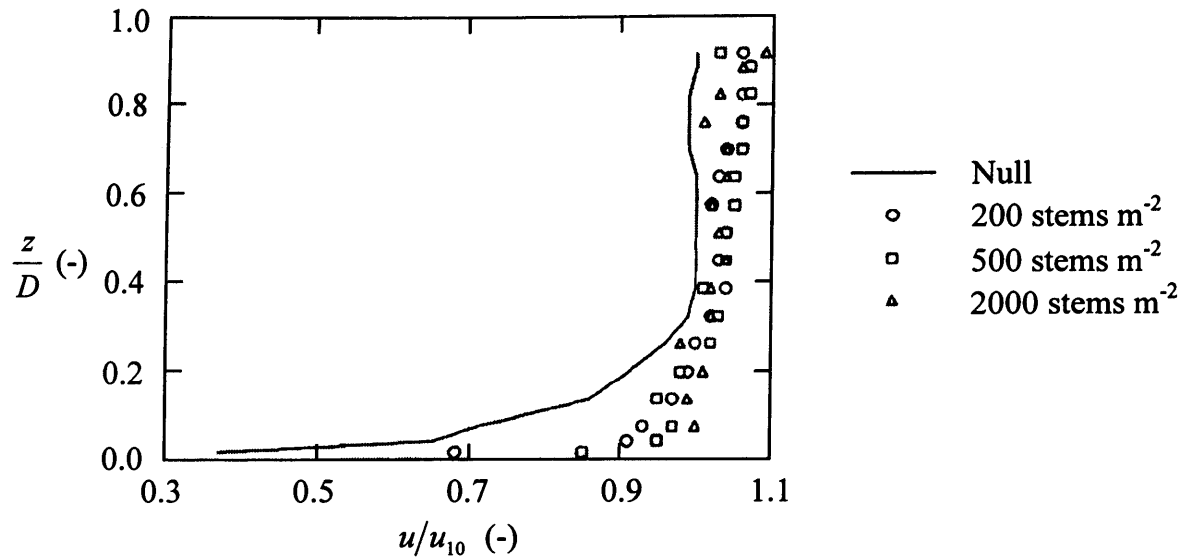
Figure 6-13 Profiles of normalised mean longitudinal velocity for emergent uniform cylinder arrays with densities of 0 (null), 200, 500 and 2000 stems \text{m}^{-2} . z is the elevation, D is the flow depth, u is the longitudinal velocity and u_{10} is the longitudinal velocity at an elevation of 100 mm for the null condition. Taken from Nepf et al. (1997b).
