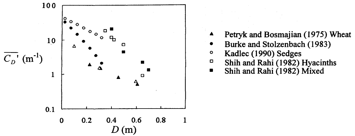
Figure 2-19 The exponential decrease in the vegetation resistance coefficient, \overline{C_D}' , with flow depth, D , for a range of vegetation types from various studies (taken from Kadlec, 1990)
