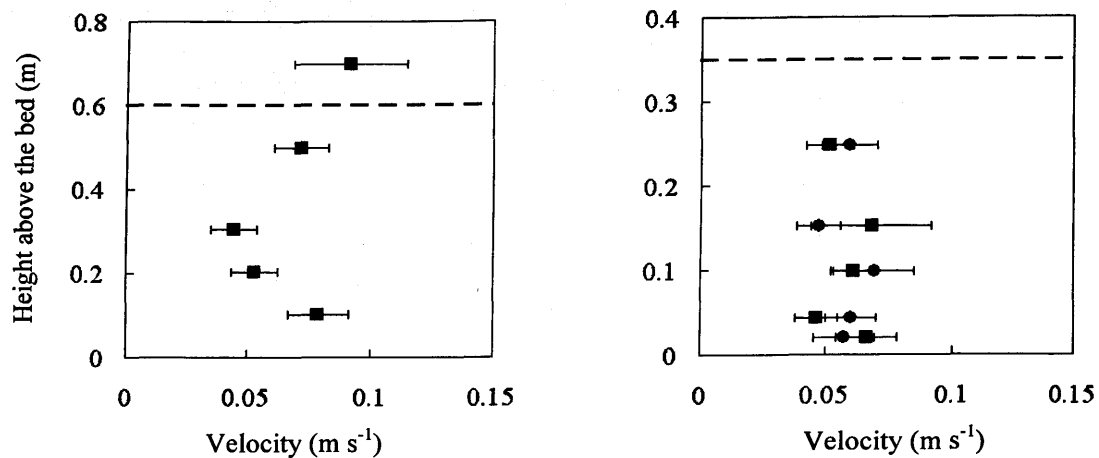
Figure 2-28 Longitudinal velocity profiles through (a) a submerged Spartina alterniflora canopy and (b) an emergent Atriplex portuloides canopy in (b), ■ and ● represent profiles that were collected during separate and consecutive inundation events respectively (Leonard & Reed, 2002)
