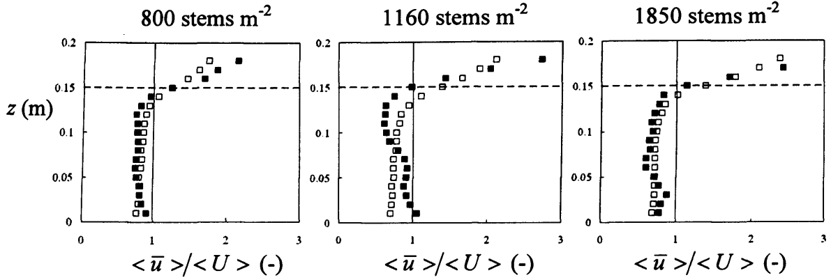
Figure 6-10 Normalised longitudinal velocity ( u ) profiles for submerged uniform cylinder arrays with a stem diameter of 6.0 mm ( \square ) and constructed vegetation canopies ( \blacksquare ), for a submergence level of 1.33, a bed gradient of 1/300, and stem densities of 800, 1160 and 1850 stems \text{m}^{-2} . U is the depth-averaged longitudinal velocity for the flow depth. The bold dotted lines denote the top of the canopy, and the faint vertical lines denote a longitudinal velocity equal to the depth-averaged value, U .
