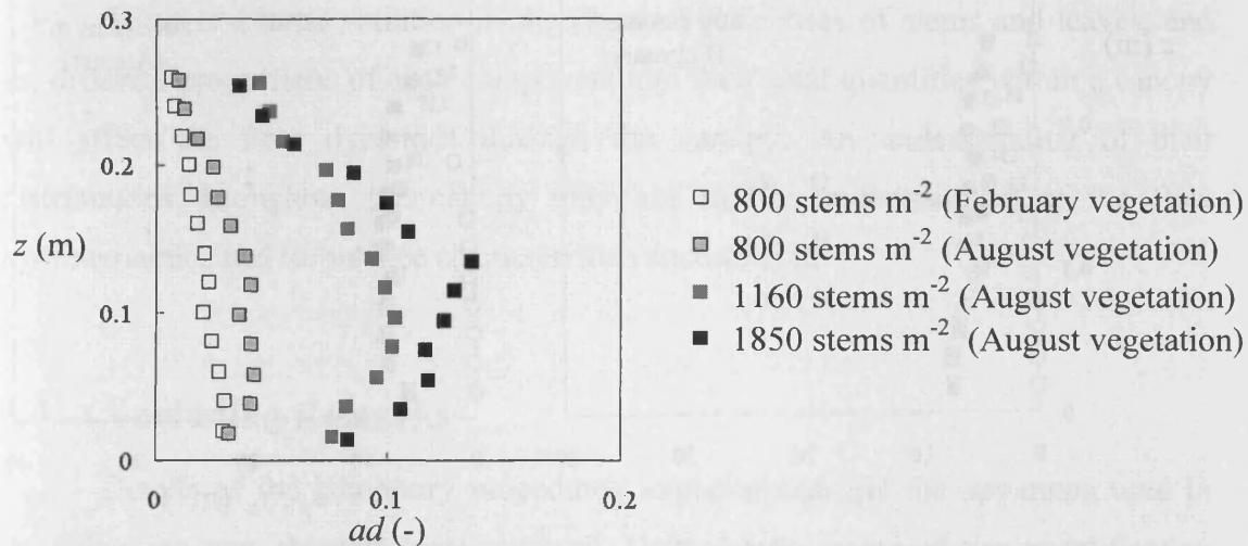
Figure 5-16 Profiles of the vegetation density parameter, ad , for three constructed canopies
