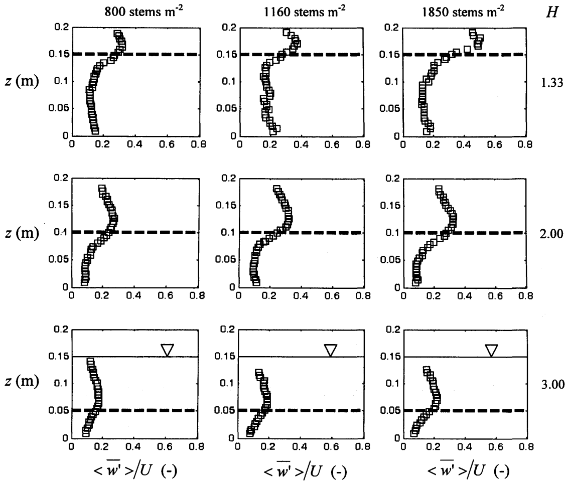
Figure 7-39 Profiles of the vertical velocity fluctuating component, w' , normalised by the depth-averaged velocity, U , for a bed gradient of 1/1000, and submergence levels of 1.33, 2.00 and 3.00. The dashed line denotes the top of the canopy.
