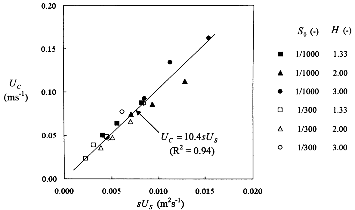
Figure 8-10 The relationship between the mean canopy layer velocity, U_c , and the product parameter sU_s for submerged canopies, where s is the stem spacing and U_s is the mean surface flow layer velocities. Data is presented for stem densities of 800, 1160 and 1850 stems m -2 , submergence levels of 1.33, 2.00 and 3.00, and bed gradients of 1/1000 and 1/300.
