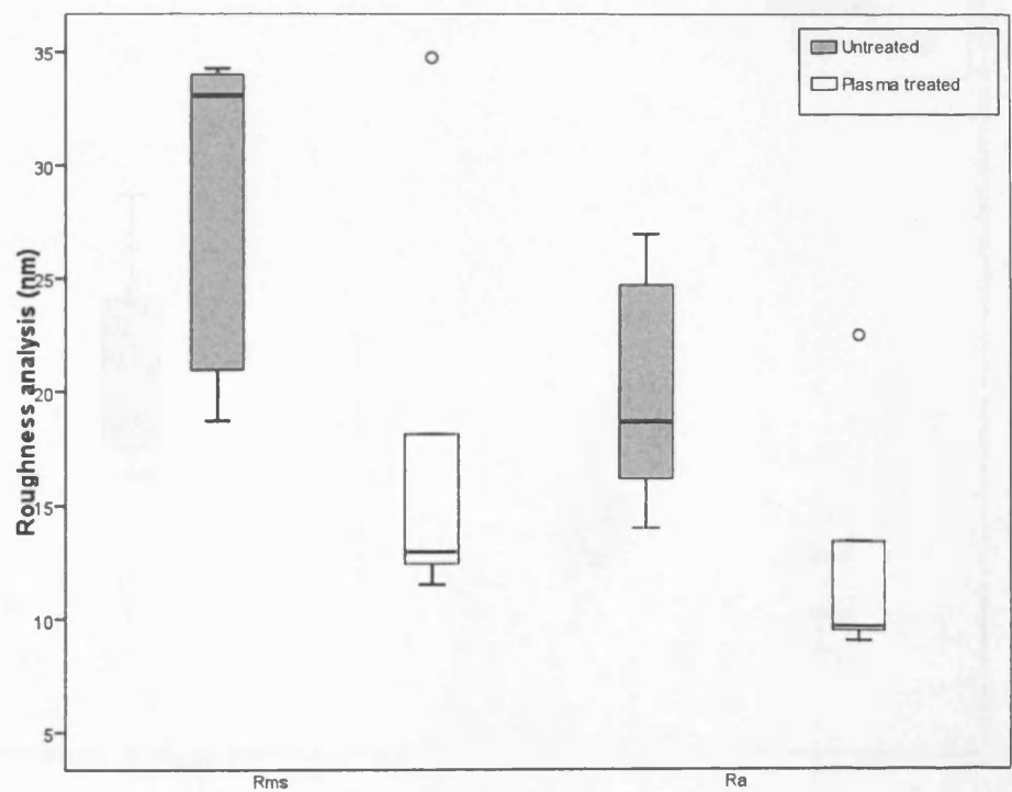
Figure 5.11 A box plot showing median and range values for surface analysis of unworn plasma treated and untreated lenses (2 lenses, 2 samples from each lens, 5 readings per sample).
