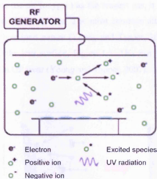
Figure 1.4 Radio frequency glow discharge set-up adapted from (Young and Tapper, 2007).
