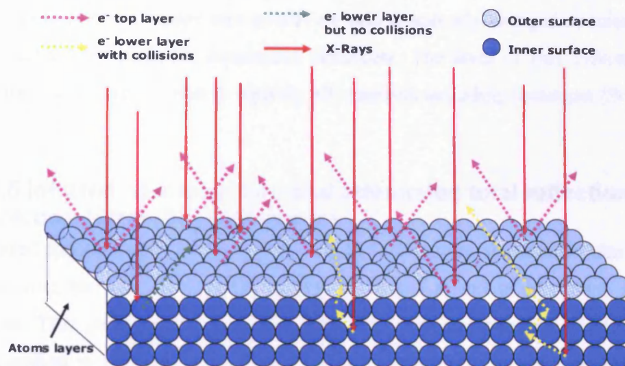
Figure 5.2 The x-ray interaction with the outer surface atom layers, adapted from Torres (2006).
