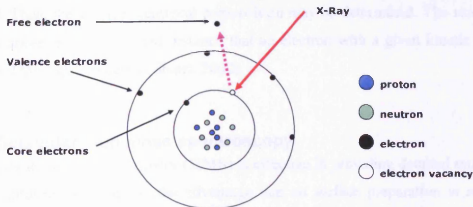
Figure 5.1 The x-ray and the atom, demonstrating that the core electrons respond well to the x-ray, adapted from Torres (2006).
