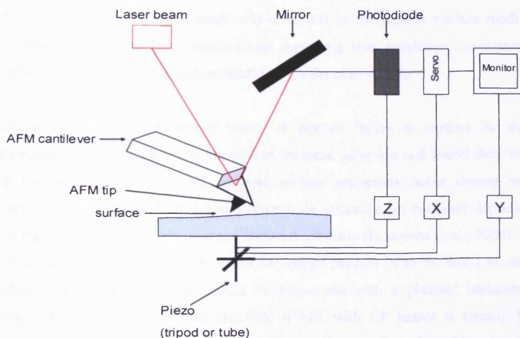
Figure 5.4 Basic AFM operation (adapted from Baguet, Sommer and Duc, (1993).
