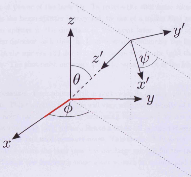
FIGURE 1.2: The sky angles \theta , \phi and \psi , between an IFO (located at the origin of the unprimed coordinates and aligned with the x - y axes) and a gravitational wave propagating in the z' direction in the TT gauge.
