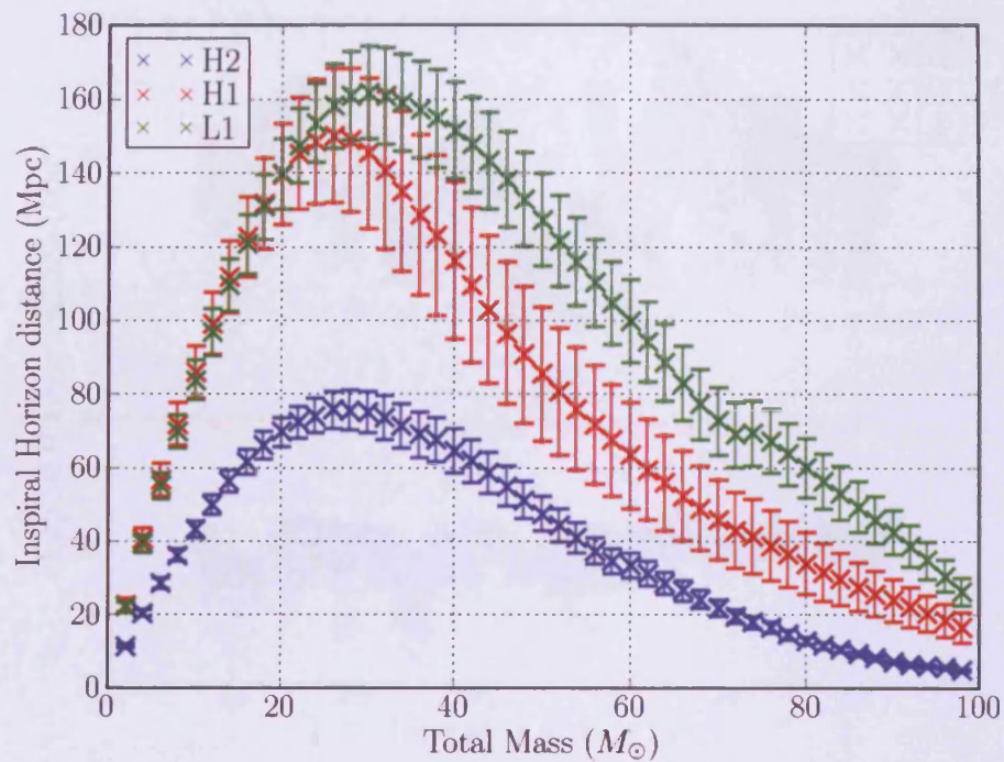
FIGURE 3.2: The inspiral-range (3.46) vs. mass for equal mass systems for each of the interferometers averaged over the course of month 1.
