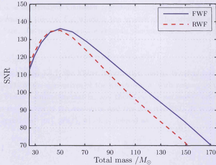
FIGURE 4.1: SNR vs. mass for both the RWF and FWF in Advanced LIGO. The signals are overhead the detector at a distance of 100 Mpc, with a constant mass ratio of 1 : 4 and inclination angle of 45^\circ .
