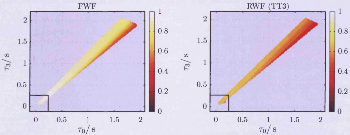
FIGURE 4.9: The ambiguity function of an IMBBH of (10, 100)M_{\odot} . There is no well defined maximum for the 0.5PN templates (left) - the overlap is close to unity for a large range of templates. As in Figure 4.8, the RWF templates (right), show similar behaviour, but do not recover the signal as well.
