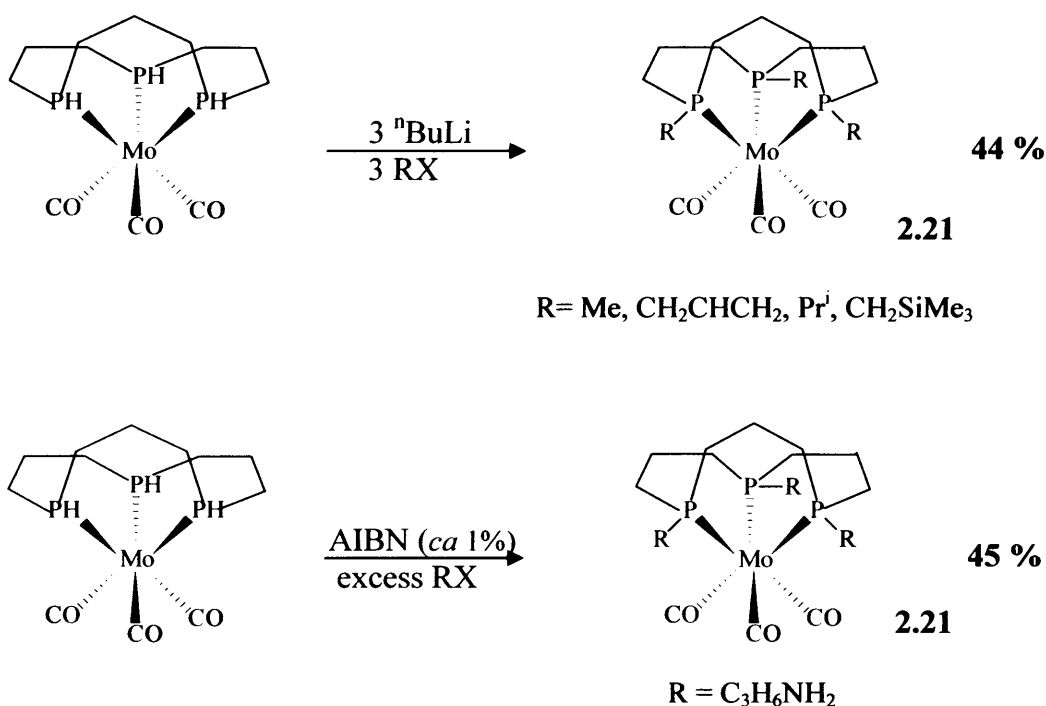
Scheme 2.6: Synthesis of tertiary phosphine macrocycles
