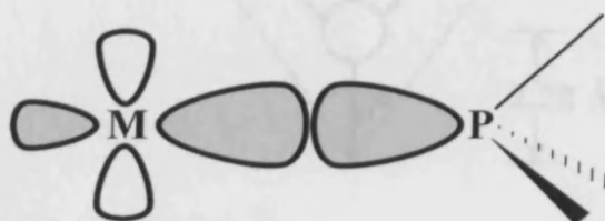
Figure 1. 2 A representation of the frontier-orbital \sigma -bonding in metal-phosphine complexes
