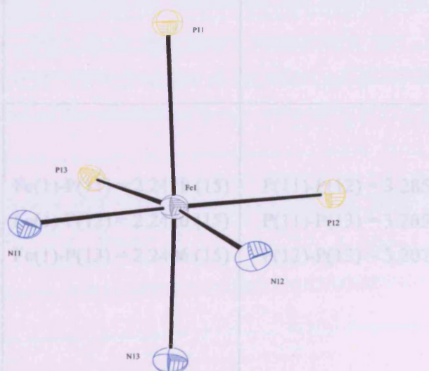
Figure 2.5: A view of the core geometry of 2.27 showing the atom numbering. Displacement ellipsoids are shown at the 30 % probability level.
