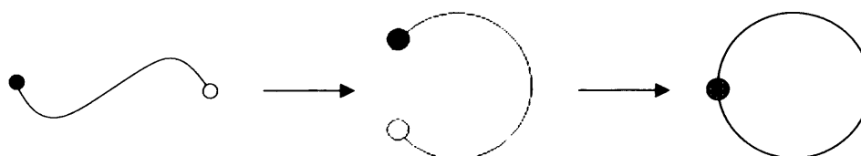
Figure 1. 8 A schematic view of the cyclization step involved in macrocycle synthesis
