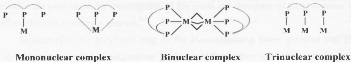
Figure 1. 5 Possible coordination modes of linear tripodal phosphines [9a, 9b, 9c]
