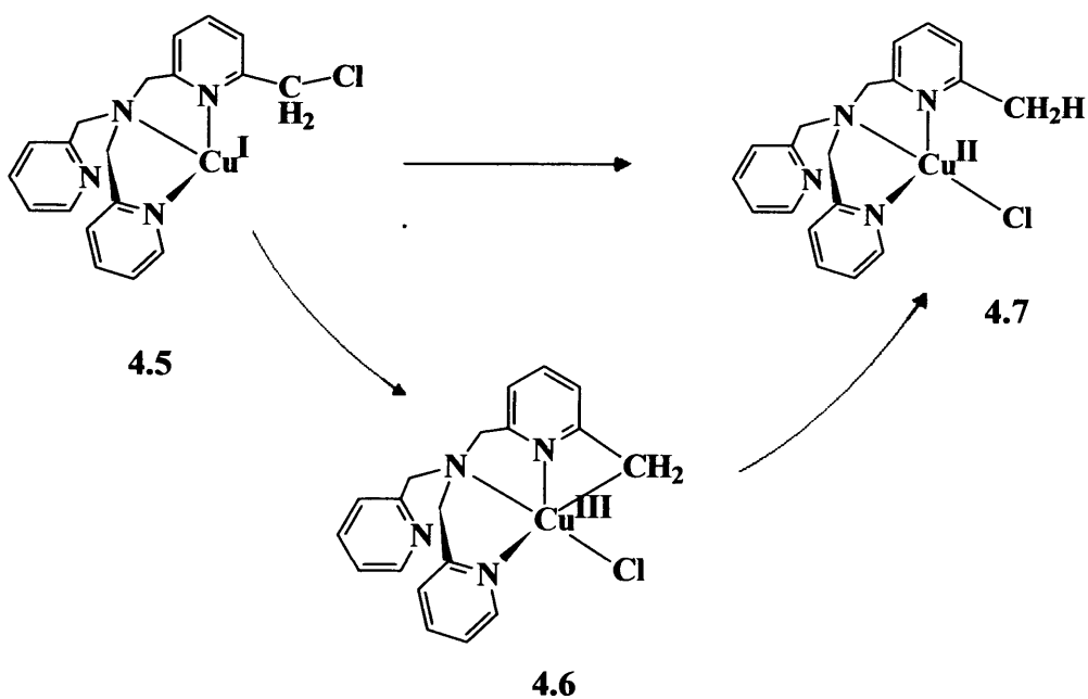
Scheme 4.3: Dehalogenation of R-Cl via Cu(III) state [10, 11]
