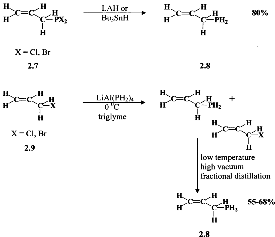
Scheme 2.1: Synthetic method for the preparation of allylphosphine. [14, 15]
