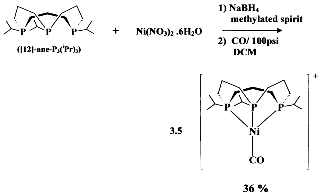
Scheme 3.6: Synthesis of mono(carbonyl)- fac -η 3 - cis -1, 5, 9-triisopropyl-1, 5, 9-triphosphacyclododecane]nickel(I)nitrate, 3.5
