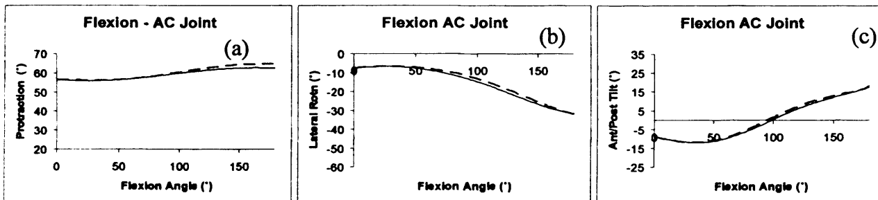
Figure 4: Flexion of the AC joint (5 th order polynomial fits). (a) protraction, (b) lateral rotation, (c) anterior/posterior tilt. Solid line: static results. Dashed line: results with adjusted scapula markers
