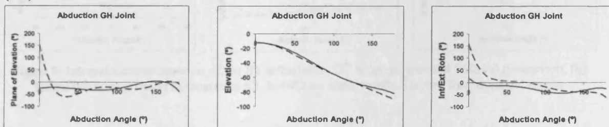
Figure 4: Abduction of the GH joint (5 th order polynomial fits). (a) plane of elevation, (b) elevation, (c) internal/external rotation. Solid line: static results. Dashed line: dynamic results
