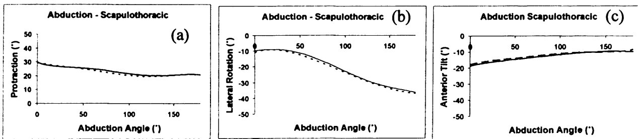
Figure 5: Abduction of the ST articulation (5 th order polynomial fits). (a) protraction, (b) lateral rotation, (c) anterior/posterior tilt. Solid line: static results. Dashed line: results with adjusted scapula markers
