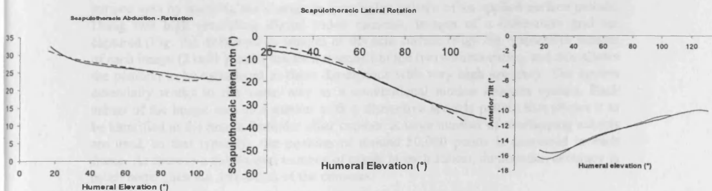
Figure 5: 5 th order polynomial fits to the kinematic waveforms for the scapulothoracic articulation during arm abduction. (a) retraction of the scapula, (b) lateral rotation of the scapula, (c) anterior tilt of the scapula. Solid line: dynamic elevation,, dashed line static elevations
