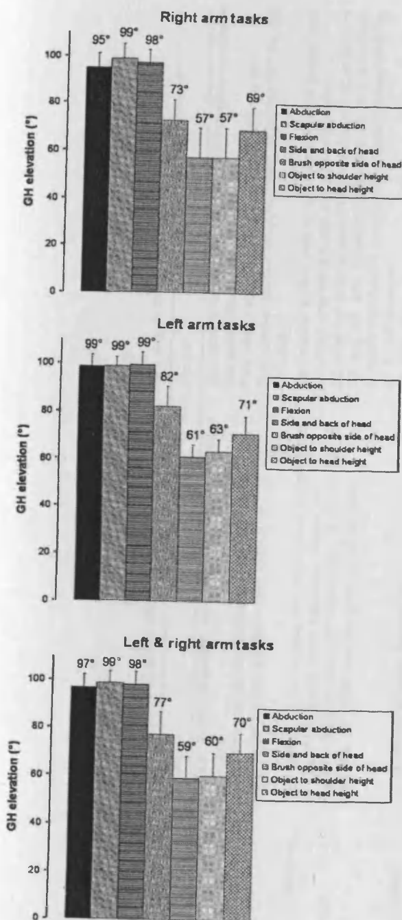
Figure 2. Average glenohumeral elevation required by five subjects to perform abduction, scapular abduction, flexion, touching the side and back of the head, brushing the opposite side of the head, lift a 20 N object to shoulder height and lift a 20 N object to head height. (a) Right arm ( n = 5 ), (b) left arm ( n = 5 ) and (c) average of both arms ( n = 10 ).
