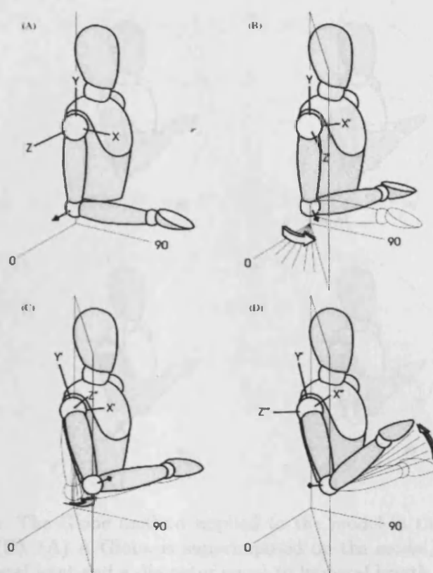
FIGURE 1.22: The I.S.B. method of measuring joint rotations: (A) shows the initial position with a vector pointing laterally (parallel to the humeral Z-axis) at 0^\circ on the XZ plane. (B) The humerus is rotated about its Y-axis until the humeral Z'-axis points to the plane of elevation. (C) The humerus is elevated about its X'-axis. (D) The humerus is externally rotated about its Y'-axis to the final position. The Y'-axis is normal to the plane containing the rotating forearm. Taken directly from [108].
