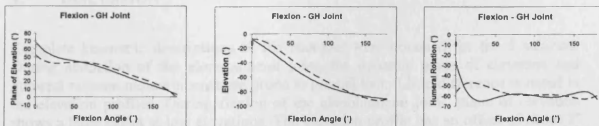
Figure 5: Flexion of the GH joint (5 th order polynomial fits). (a) plane of elevation, (b) elevation, (c) internal/external rotation. Solid line: static results. Dashed line: dynamic results
