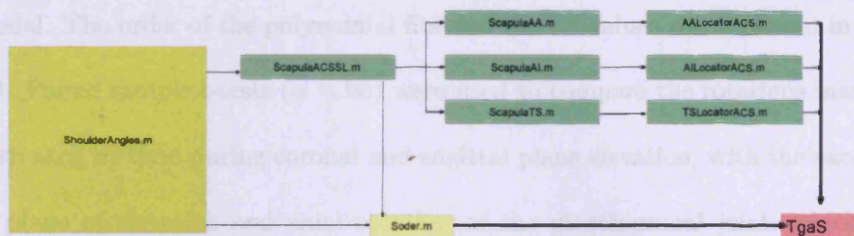
FIGURE 2.10: Schematic of the sub-routine to calculate the rotations of the shoulder complex using the scapula locator. A description of each function and a glossary of the variables used in the schematic can be found in Tables 2.2 and 2.3.
