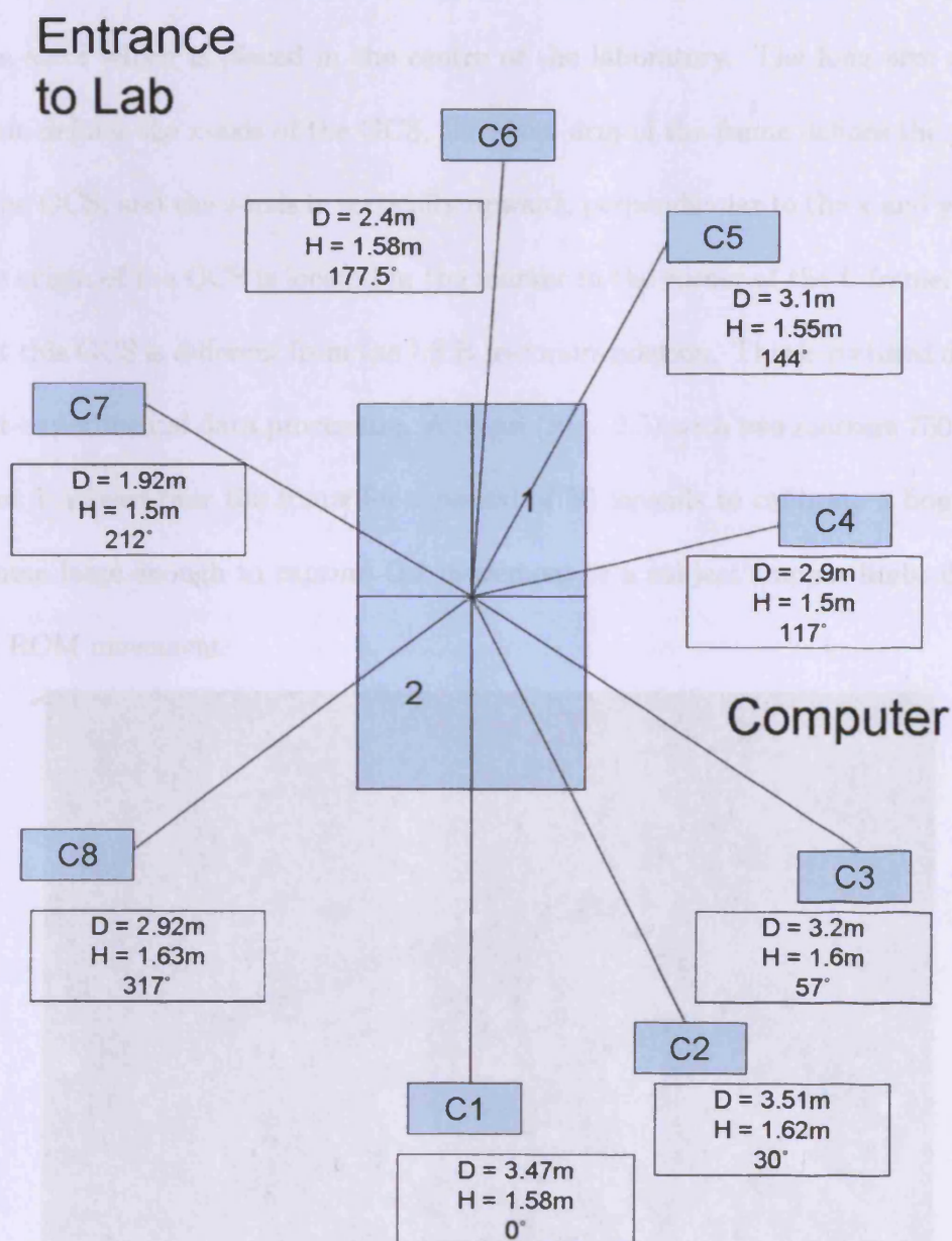
FIGURE 2.2: A schematic showing the positions and heights of the eight cameras during testing relative to two force plates (1 and 2) in the centre of the gait lab. C1-C8 indicate cameras 1-8.
