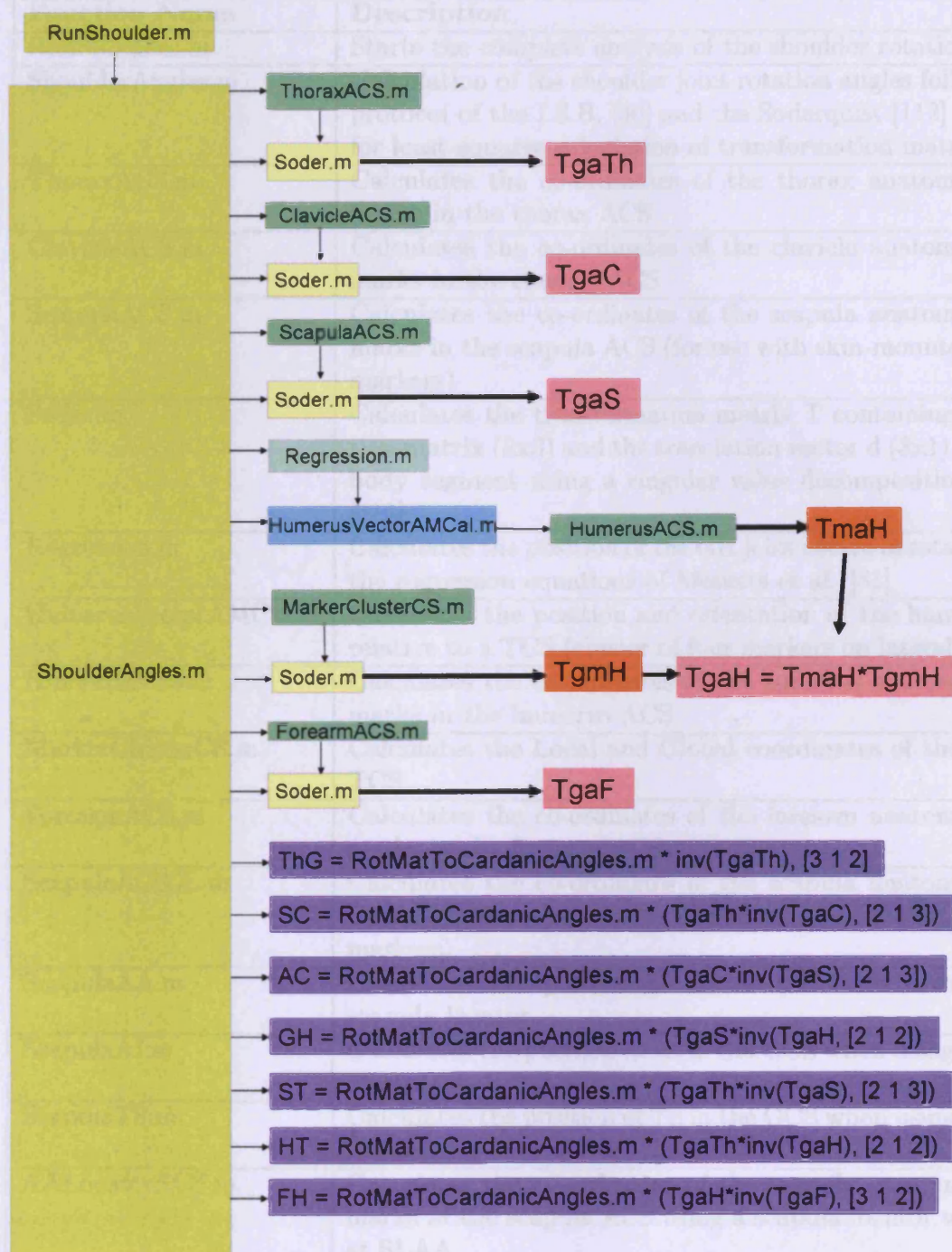
FIGURE 2.9: Schematic of the software used to calculate the rotations of the shoulder complex using skin-markers on the scapula. A description of each function and a glossary of the variables used in the schematic can be found in Tables 2.2 and 2.3.
