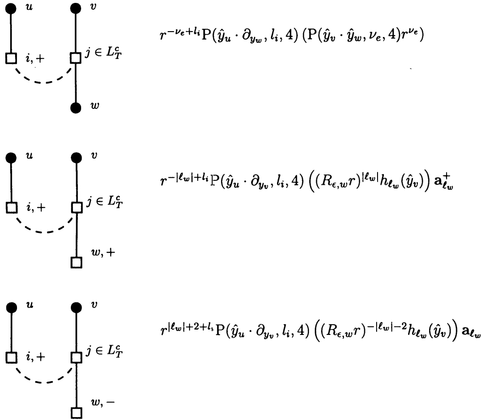
Figure 4.8: Second part of the rules for the amplitude of a renormalization tree T . The above objects correspond to bullet point number 7 of the rules in the main text.
