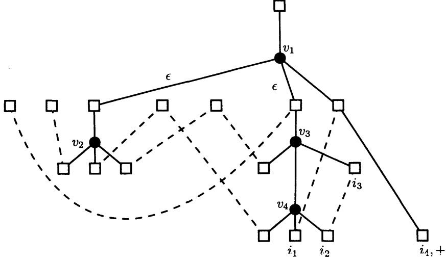
Figure 4.10: A renormalization tree contributing to Y_4(\varphi, x) .
