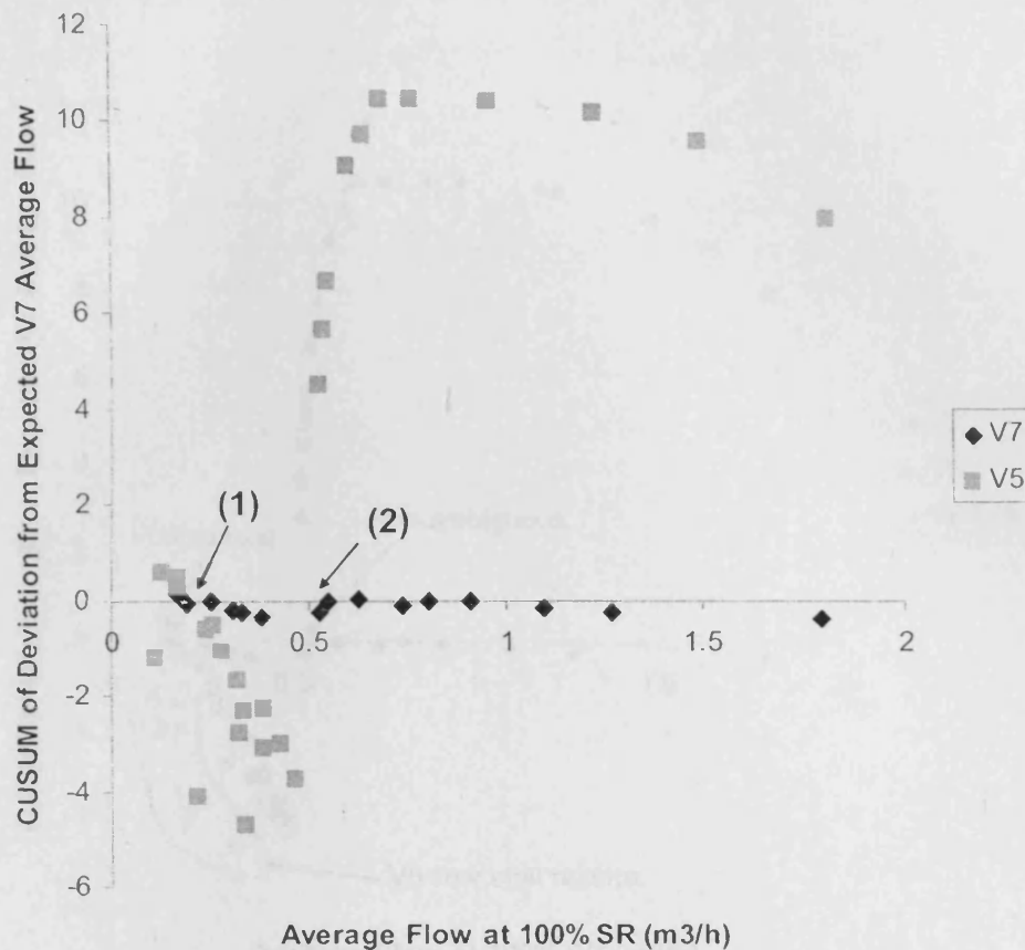
Figure 4.18: Test results for 100% to 55% speed request test cycle.
