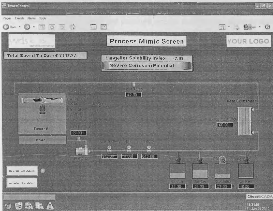
Figure 7.22: Process mimic with LSI indicator.
