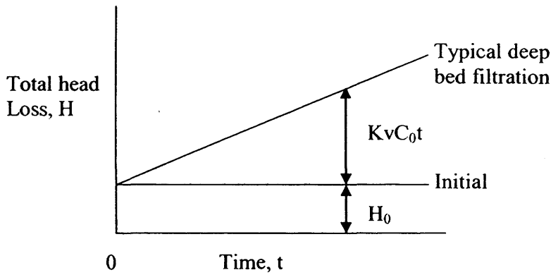
Figure 5.4: Total head loss varying with time.
