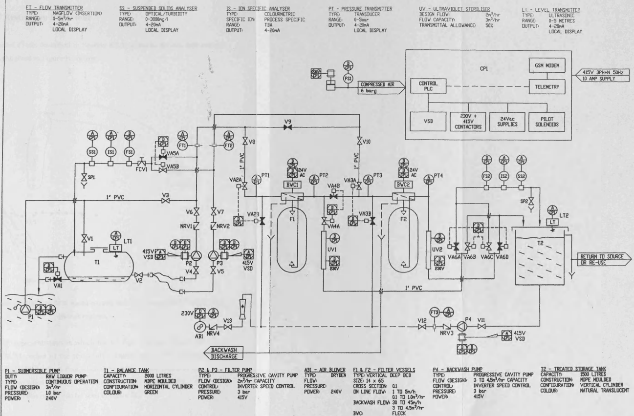
Appendix B: WRAP Rig Piping and Instrumentation Diagram
