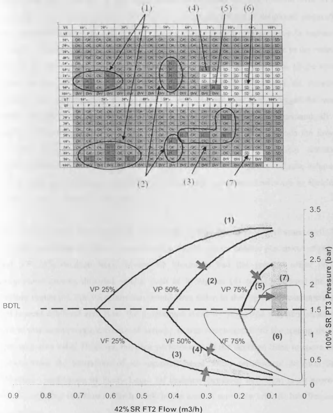
Figure 6.11: Explanation of combined blockage diagnostic test results.
