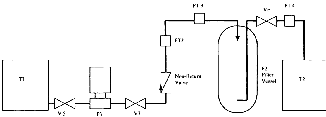
Figure 5.3: Simplified Schematic of the filter 2 subsystem showing filter fouling simulation valve VF.
