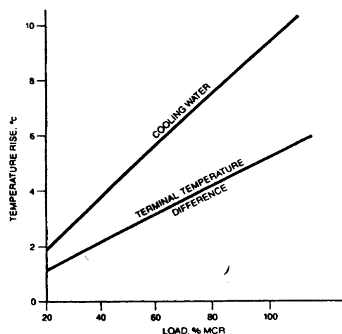
Figure 7.15: Condenser cooling water temperature rise and TTD for a typical condenser. (Gill [90])
