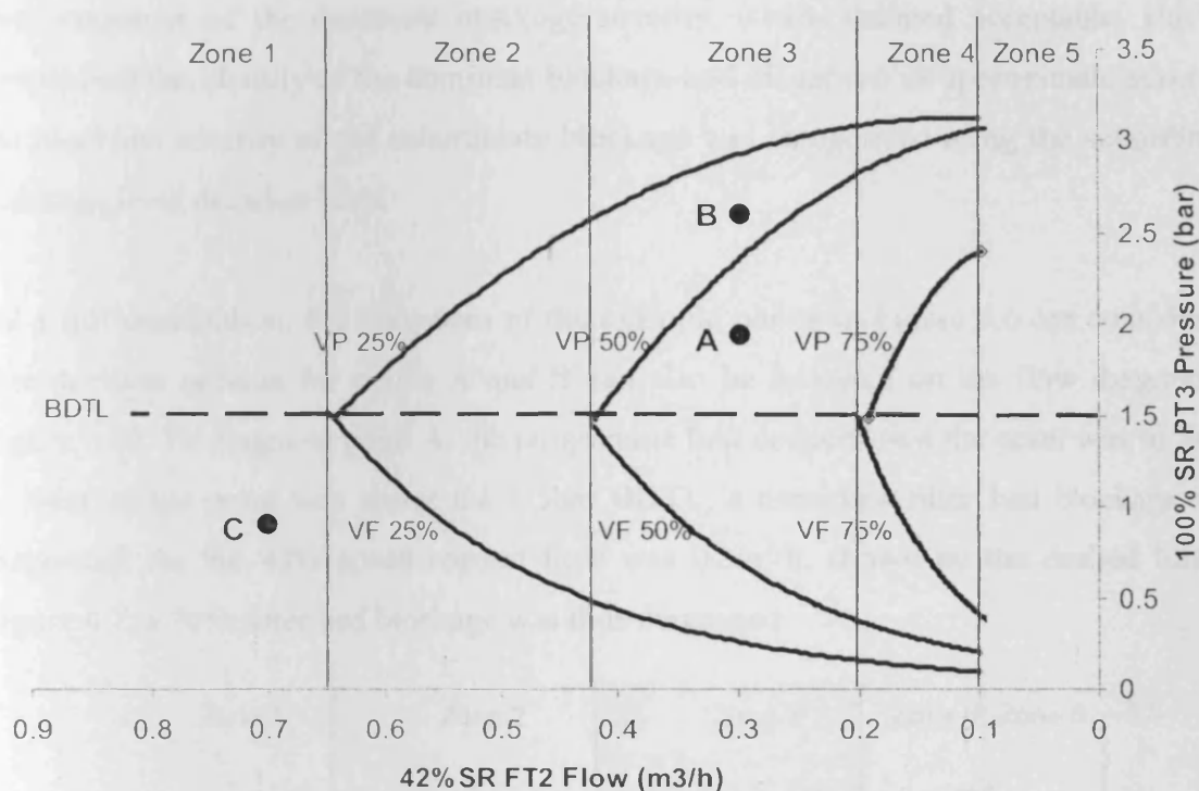
Figure 6.6: Threshold template.
