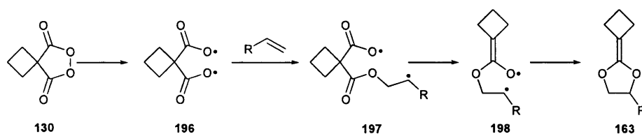
Scheme 3.21
