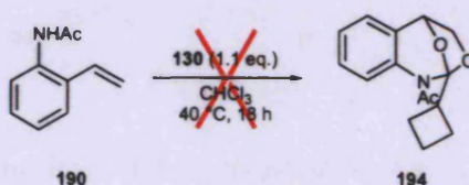
Scheme 3.19
