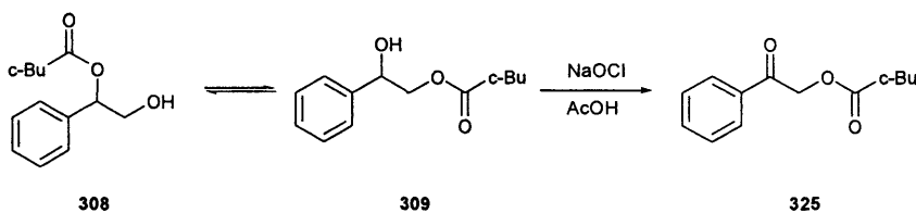
Scheme 4.19
