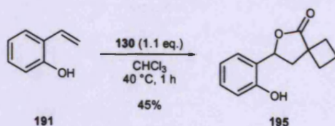
Scheme 3.20
