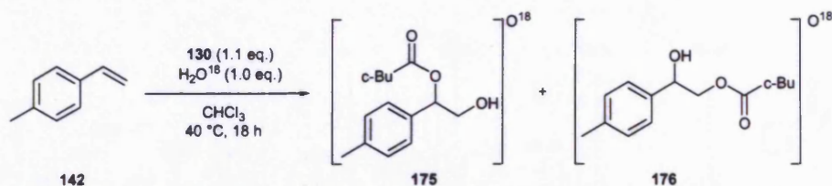
Scheme 3.11
