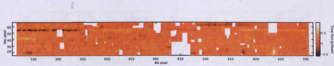
Figure 7.17: Integrated flux maps for the VC1 cubes, velocity range 300-3,000 km/s.
