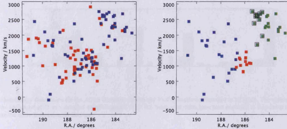
(a) 59 AGES detections (blue squares) together with 55 VCC non-detections (red circles) with available redshift measurements
