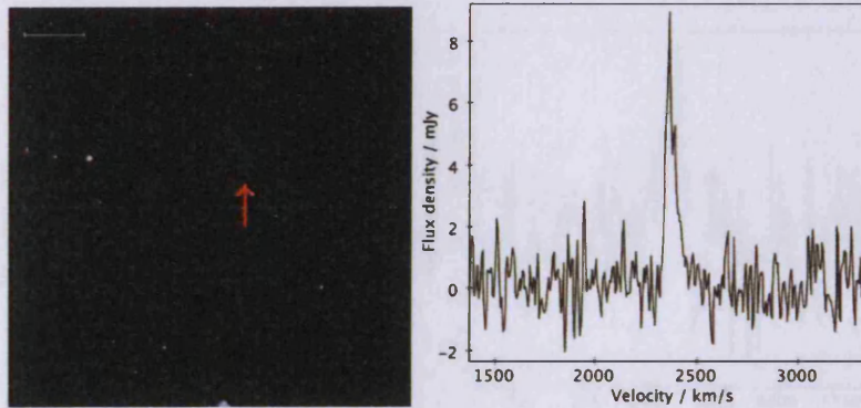
(c) Source 56 RGB, VCC 190.
