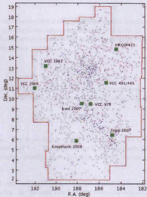
Figure 8.8: Map of the Virgo Cluster showing VCC galaxies as blue points, with green squares highlighting the approximate centers of known extended HI features spanning more than 3.5^\circ .
