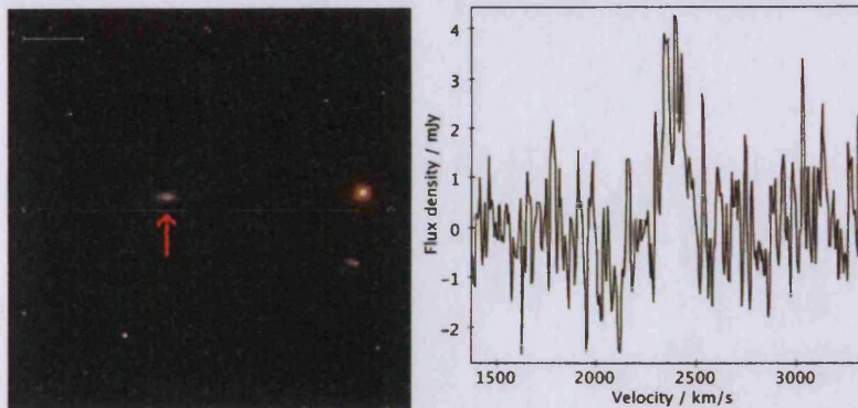
(a) Source 47 RGB, VCC 450. VCC 439 is visible to the west.
