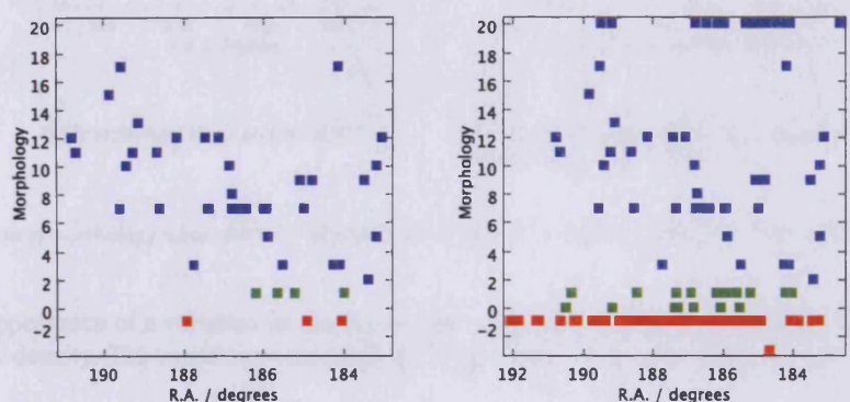
(a) Morphology of the HI detections, with an existing classification, varying across the cube.
