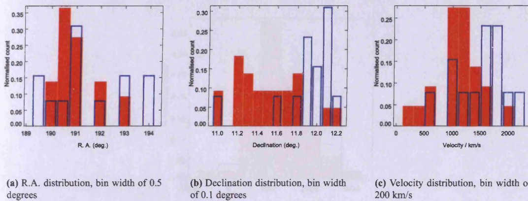
Figure 6.5: Distribution histograms of HI detections with cz < 3,000 km/s (blue) and VCC cluster members not detected in HI (red). All 60 VCCs without AGES detections are used in the spatial histograms, only those 23 with optical redshifts are used in the velocity distribution. In all histograms the count of both samples has been normalised to give a total of 1.0 for each.
