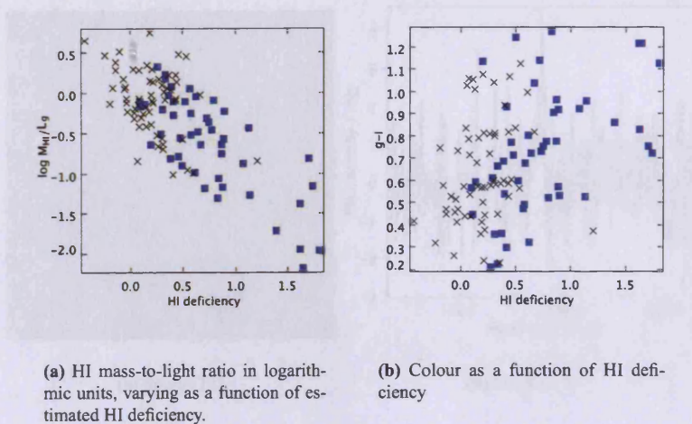
Figure 5.20: Relations between HI deficiency, M_{HI}/L_g ratio and colour. Blue squares are Virgo detections while black crosses are background galaxies.
