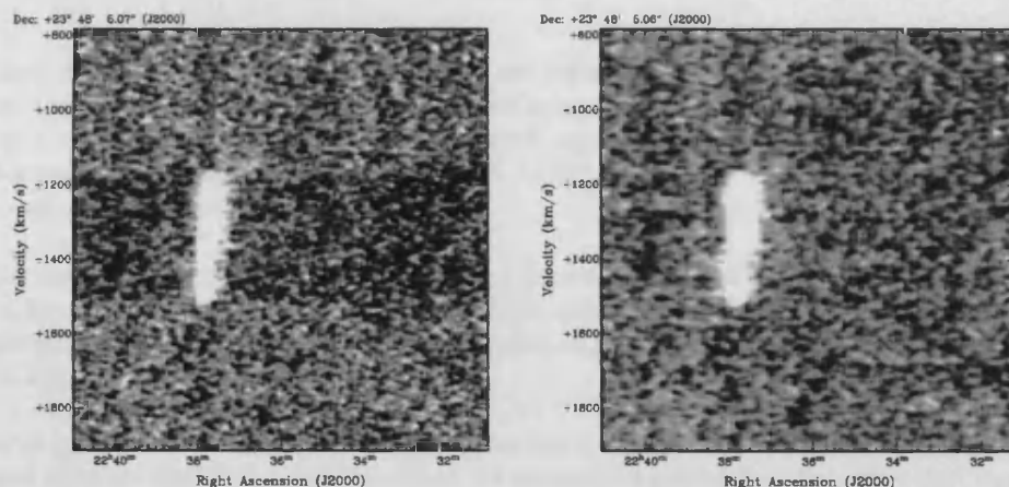
Figure 2.4: Example of over-subtraction of the bandpass from an extended source, using the standard median estimation (left). Using the "MinMed" estimator effectively removes the negative lobes (right). The image is of NGC 7339, courtesy Robert Minchin.
