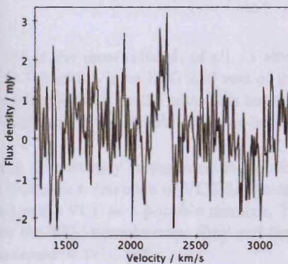
(f) Source 145 HI profile.
