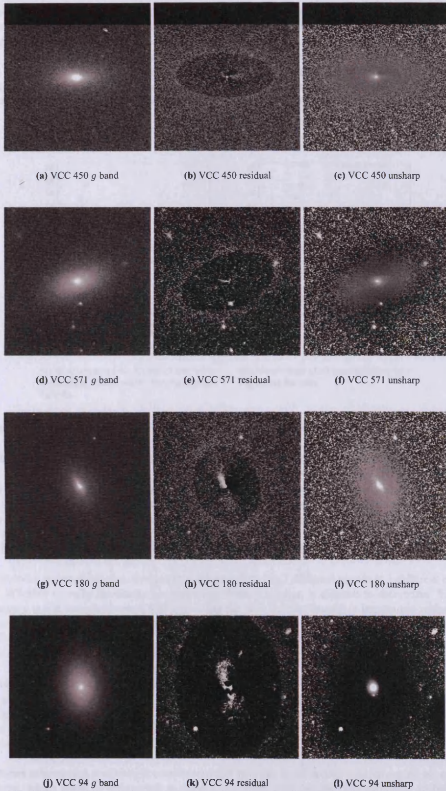
Figure 5.11: SDSS g -band, residual images and unsharp masks (using elliptical profiles with kernel sizes of 20 pixels) for the S0s detected in HI. Images are 1.7' across. The model from IRAF does not quite extend to the outer edge of each galaxy, hence the appearance of a cutoff ring in the residual images. The type 2 VCC 94 is shown for comparison.
