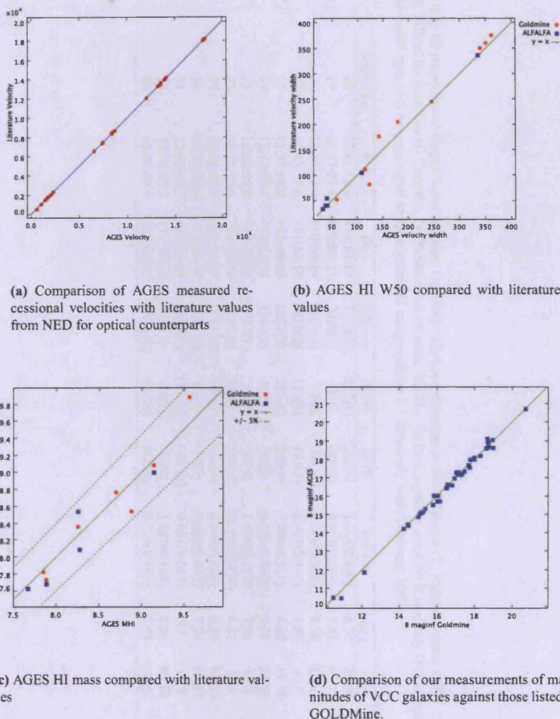
Figure 6.2: Comparisons of optical and HI data with existing measurements from the literature. The solid line shows the one to one correlation.
