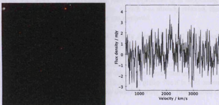
(a) SDSS RGB image, 6" across. VCC 52 is the blue object west of center.
