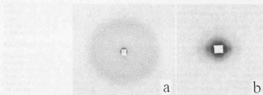
Figure 18. Small-angle patterns of chromatin taken from living cells. (a) Living rabbit erythrocytes, and (b) living whole sea urchin sperm Echinus esculentus in semen. Reproduced with permission from [104], J. P. Langmore and J. R. Paulson, J. Cell Biol. 96, 1120–1131 (1983). © 1983, Rockefeller University Press.
