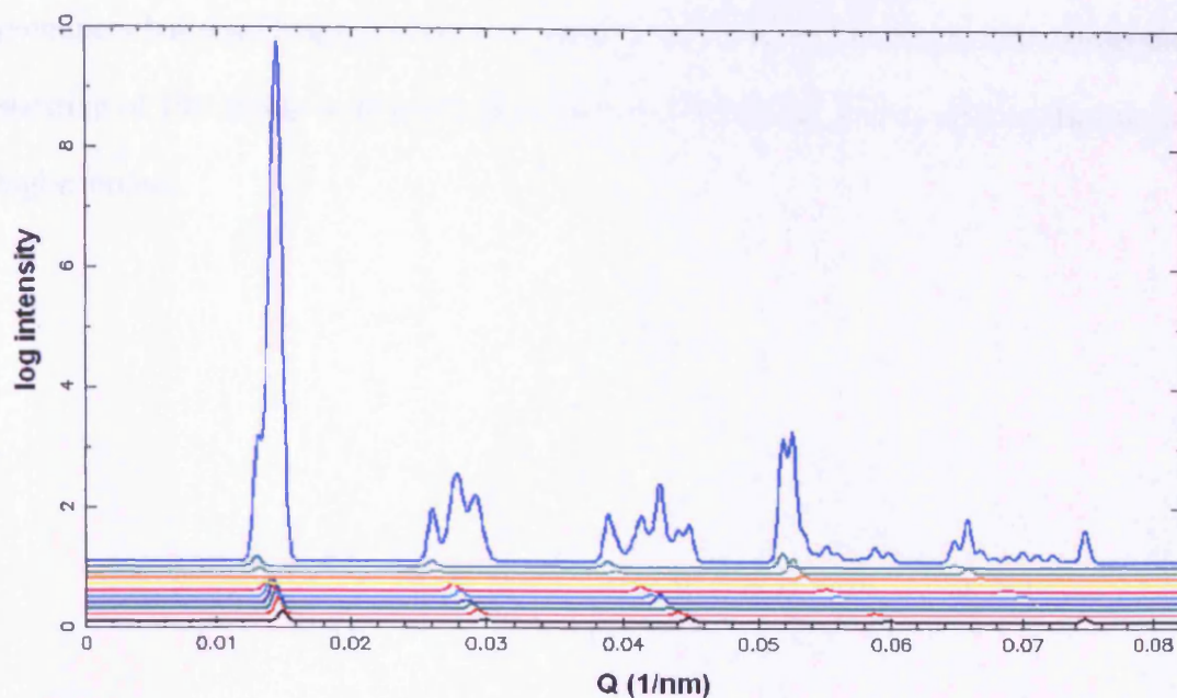
Figure 6.9: Simulated meridional X-ray diffraction pattern for ten different structures from 234 amino acids to 274 amino acids at an increment of four amino acids per structure. This shows the first five orders of collagen axial diffraction and the accumulative structure.
