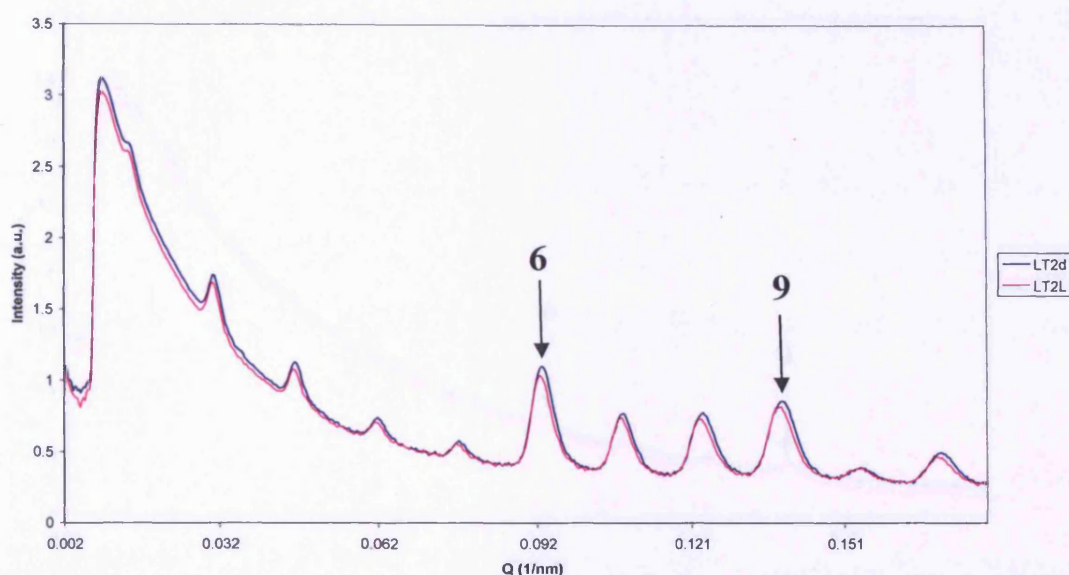
Figure 5.7: Small angle X-ray diffraction one-dimensional linear trace for samples LT2d and LT2L. A shift in the D-period (axial periodicity) is visible, from a lower D-period for the parchment kept at constant conditions (LT2d) to a higher D-period value for the parchment kept at fluctuating conditions (LT2L). The sixth and ninth orders of diffraction are indicated.
