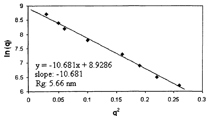
Figure 5. Guinier plot of \ln I(q) against q^2 . The innermost part of the scattering curve is used to calculate the size of the molecule. The slope from the Guinier plot is directly related to the radius of gyration.
