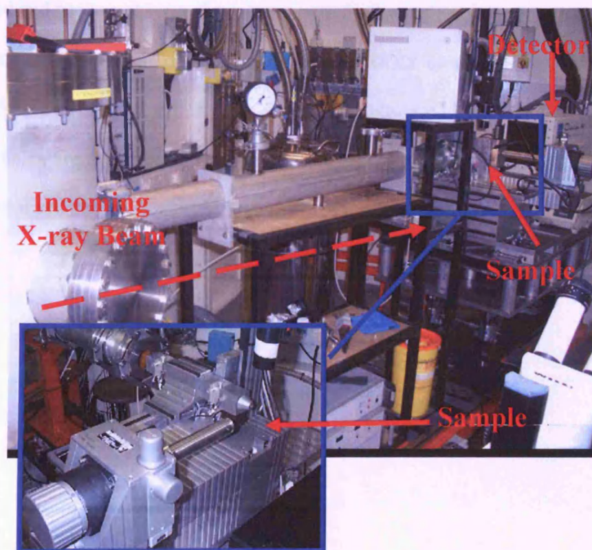
Figure 3.8: Image of station 14.1 at SRS Daresbury at a sample to detector distance of 140mm. The sample area is shown in detail in an additional image (see inset). The red dashed arrow indicates the direction of the incoming X-ray beam.
