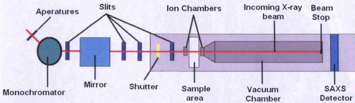
Figure 3.6: Schematic representation of Station 2.1, SRS Daresbury, UK. Adapted from http://srs.dl.ac.uk/ncd/station21/2.1_floorplan.html (Snigirev et al., 1996).
