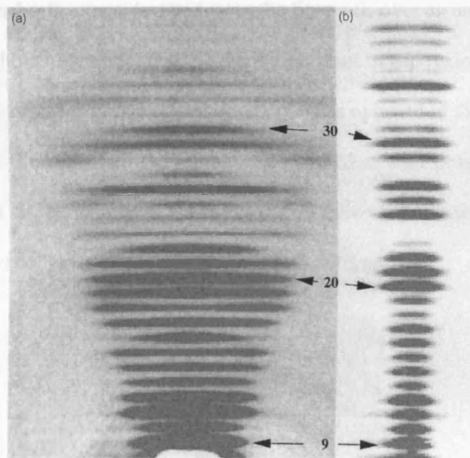
Figure 1.11: Two small-angle meridional X-ray diffraction patterns of collagen taken from Wess and Orgel (2000). (a) Dry rat-tail tendon. (b) Hydrated rat-tail tendon. The meridional peaks shown are for orders 9 to 34 with the 9th, 20th and 30th orders identified.
