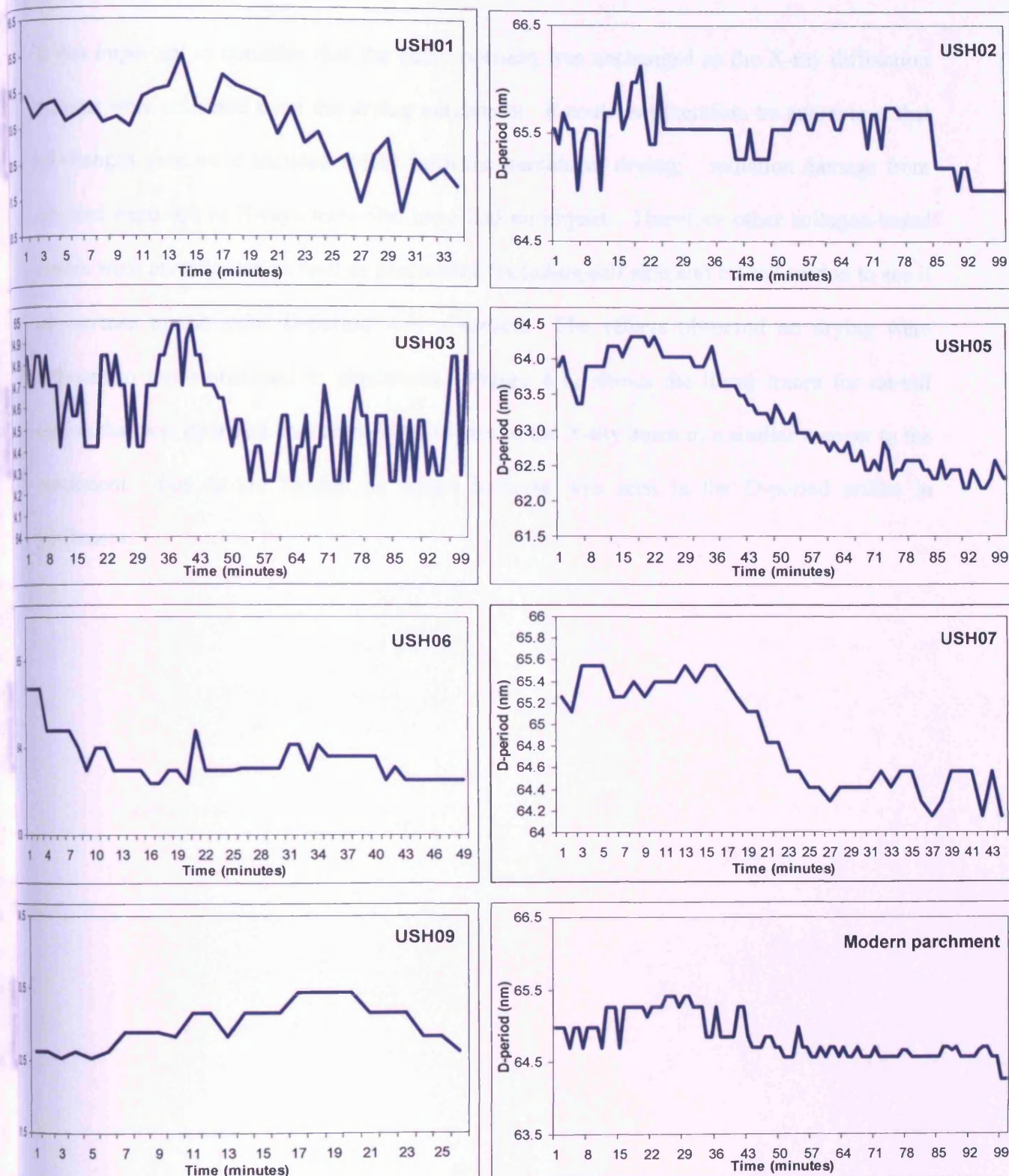
Figure 4.10: The D-period as a function of drying time for all parchment samples that were hydrated and allowed to dry. The x-axis and y-axis are plotted on different scales for all samples.
