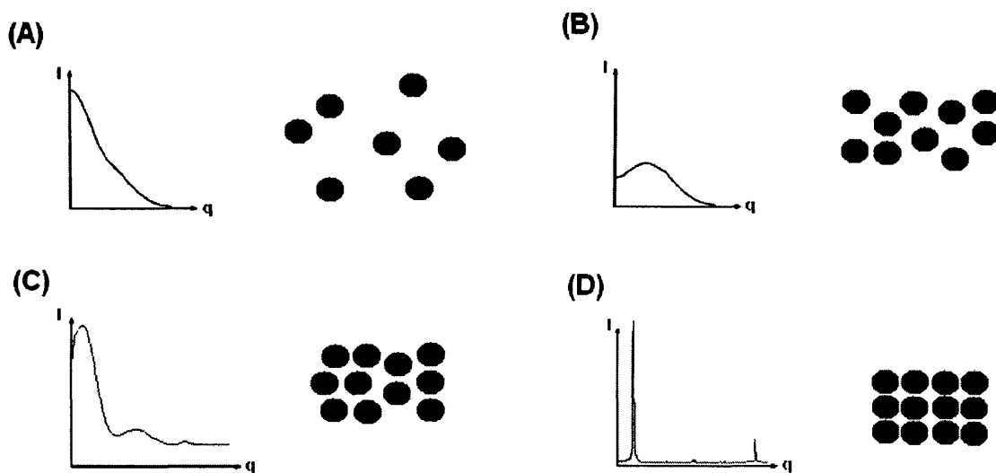
Figure 2.1: Scattering curves generated from various states of matter: (A) gas-type sample, (B) liquid-type, (C) quasi-crystalline and (D) solid state. Adapted from (Glab, Wess and Thomas, Due to be published in 2009) and (Cullity, 1978).
