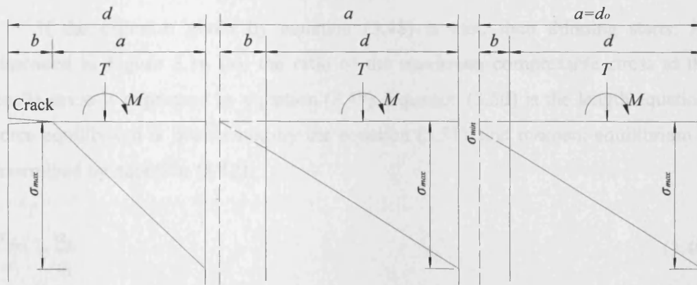
(a) No tension model thinning
