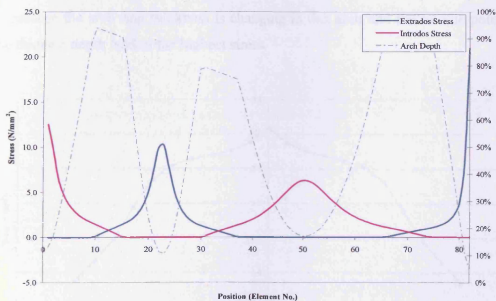
Figure 7.17 The stress over Shinafoot bridge
