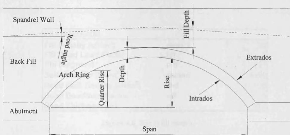
Figure 4.3 Arch geometry
