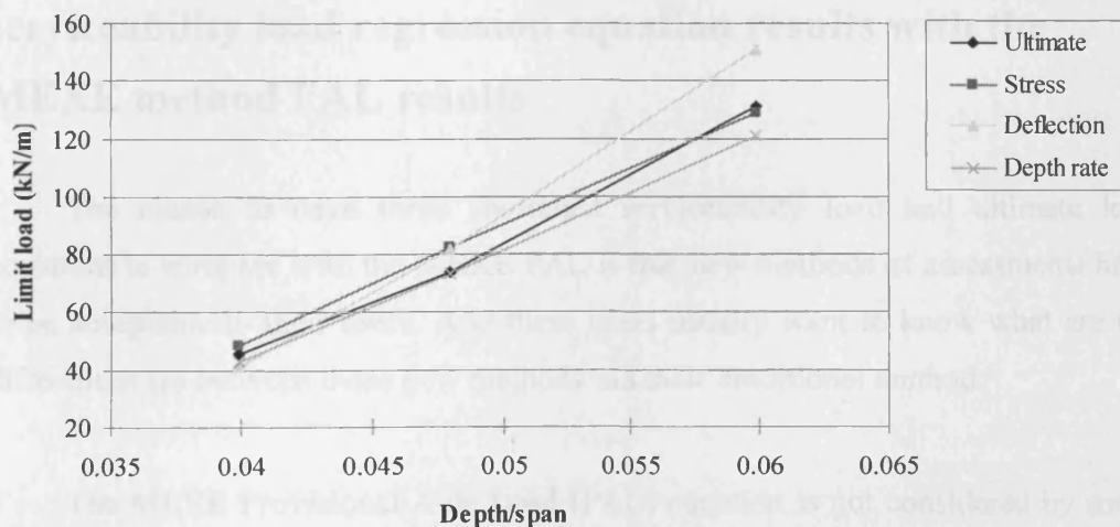
Figure 6.32 Spreadsheet results comparison by different depth/span
