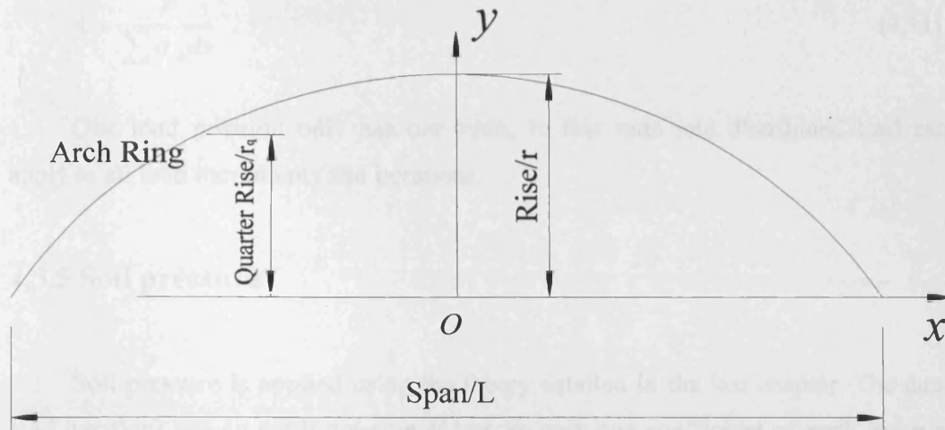
Figure 4.26 Arch geometry coordinate
