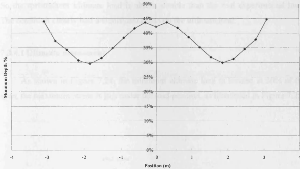
Figure 7.22 The minimum depth when moving load over Shinafoot bridge
