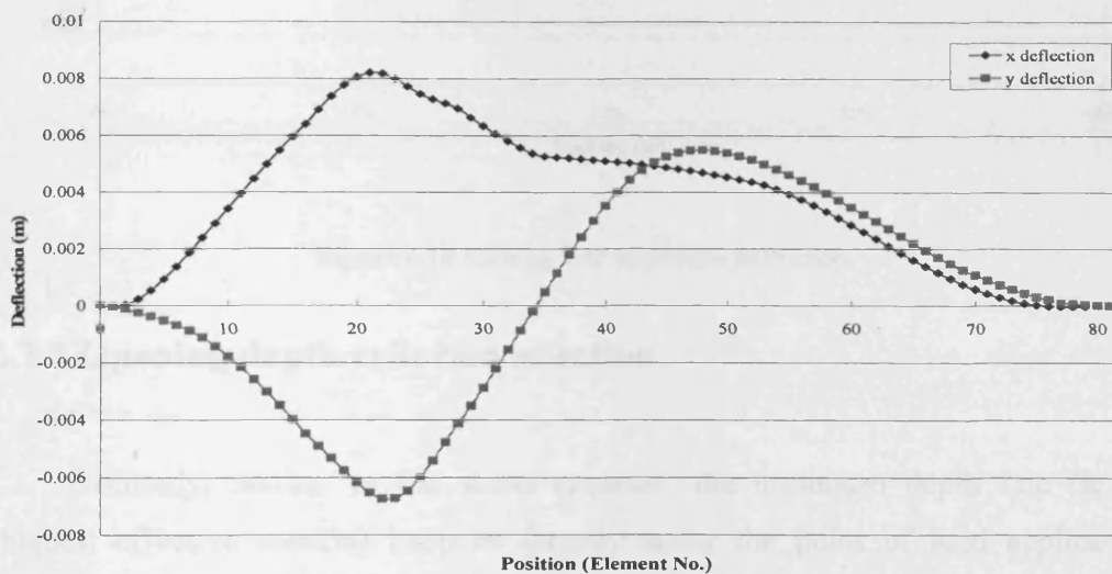
Figure 6.8 Normal bridge vertical and horizontal deflection
