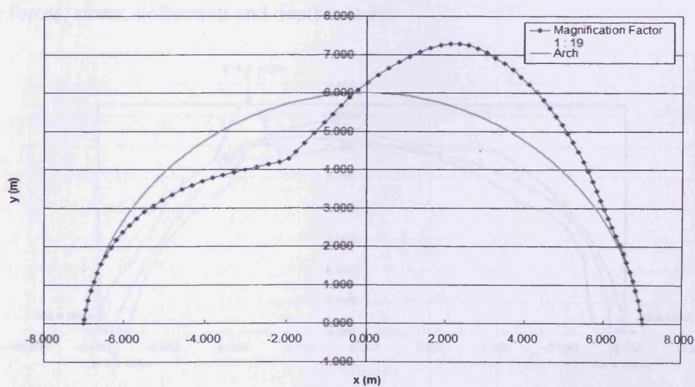
Figure 4.39 Deflected shape
