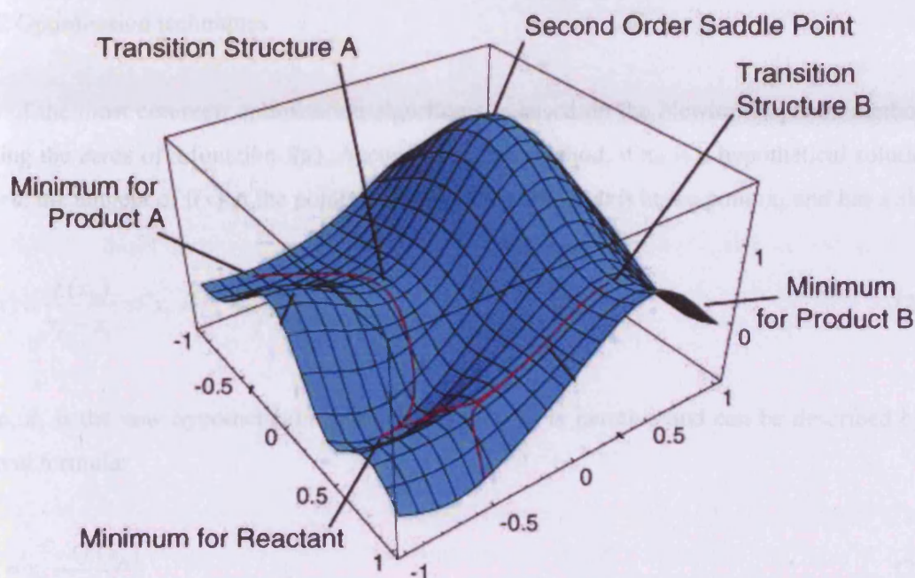
Figure 2.4.1: Example of a PES.
