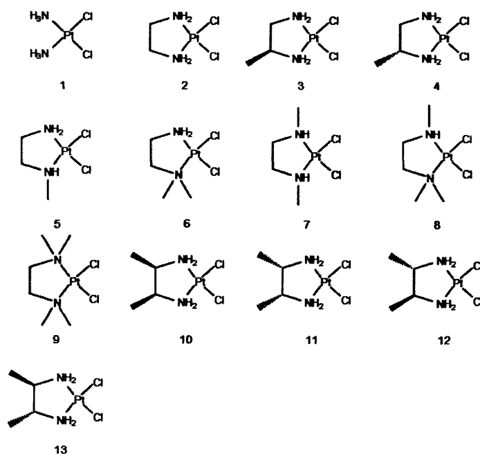
Figure 4.3.1: Structures of compounds 1 – 13.
