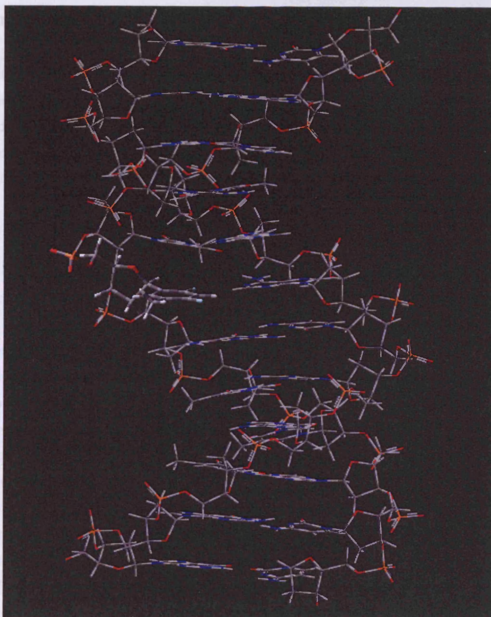
Figure 4.5.8: Structure of DNA dodecamer containing the dF-A pair (pdb entry: 1BW7).
