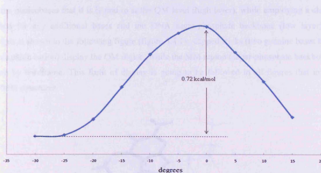
Figure 3.3.3: Energy barrier to rotation of the benzene ring in the [(\eta^6\text{-ben})\text{Fe}(\text{en})\text{Cl}]^+ complex.
