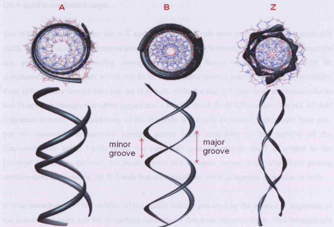
Figure 1.4.2: Axial (top) and side (bottom) view of A-, B- and Z-DNA forms.
