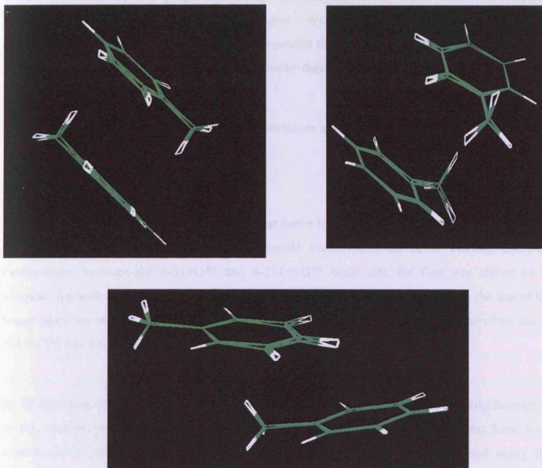
Figure 3.1.6: Superposition of literature and BHandH optimised geometries for the three toluene dimers.
