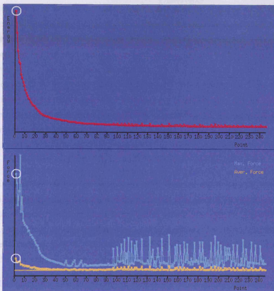
Figure 4.5.6: Energy (top) and forces (bottom) during optimisation of complex 2.
