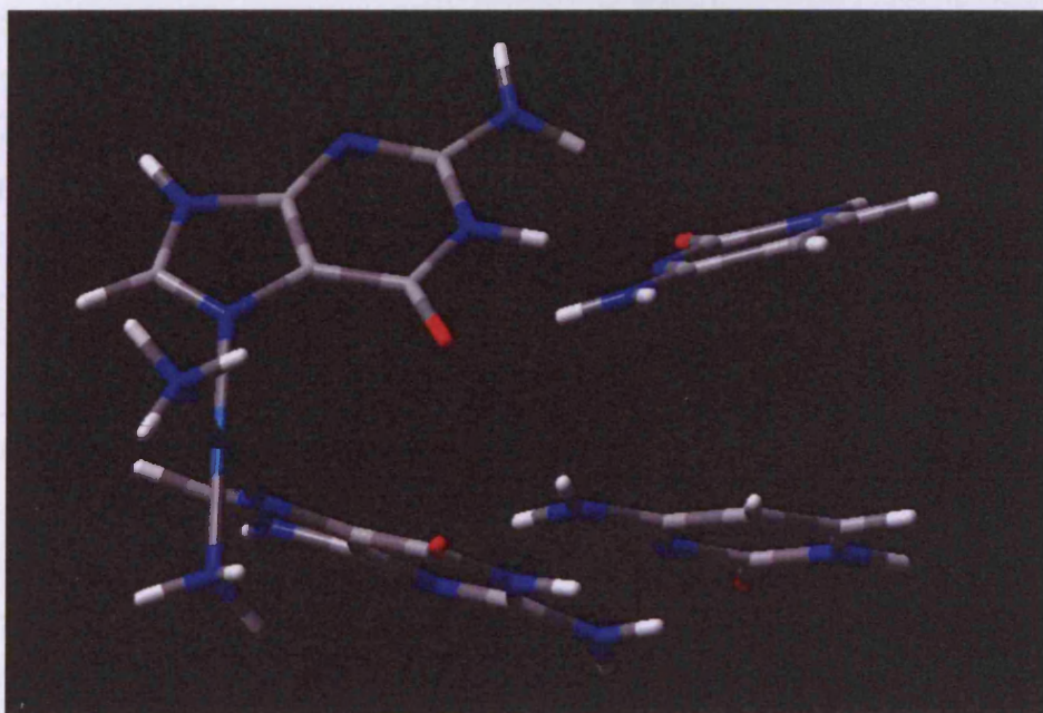
Figure 3.5.1: Truncated model from the 1AU5 structure.
