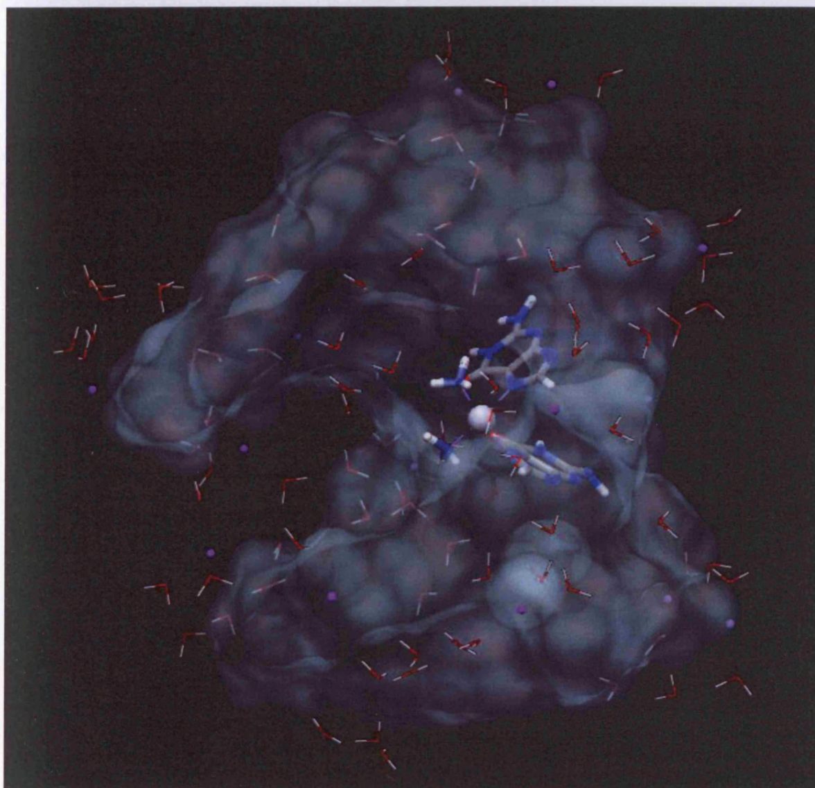
Figure 3.4.17: Optimised structure of the solvated cisplatin-DNA structure (solv90). The Pt atom is shown as white sphere and the rest of the QM region as capped sticks; \text{Na}^+ ions shown as purple spheres and solvent molecules as wireframe. The MM part has been replaced by a solid surface of 60% transparency for clarity. 162,163
