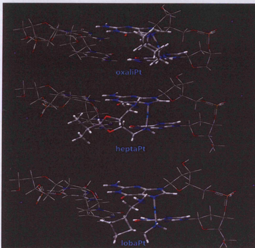
Figure 4.4.2: Optimised geometries of the three platinum complexes with ds-GpG.CpC.
