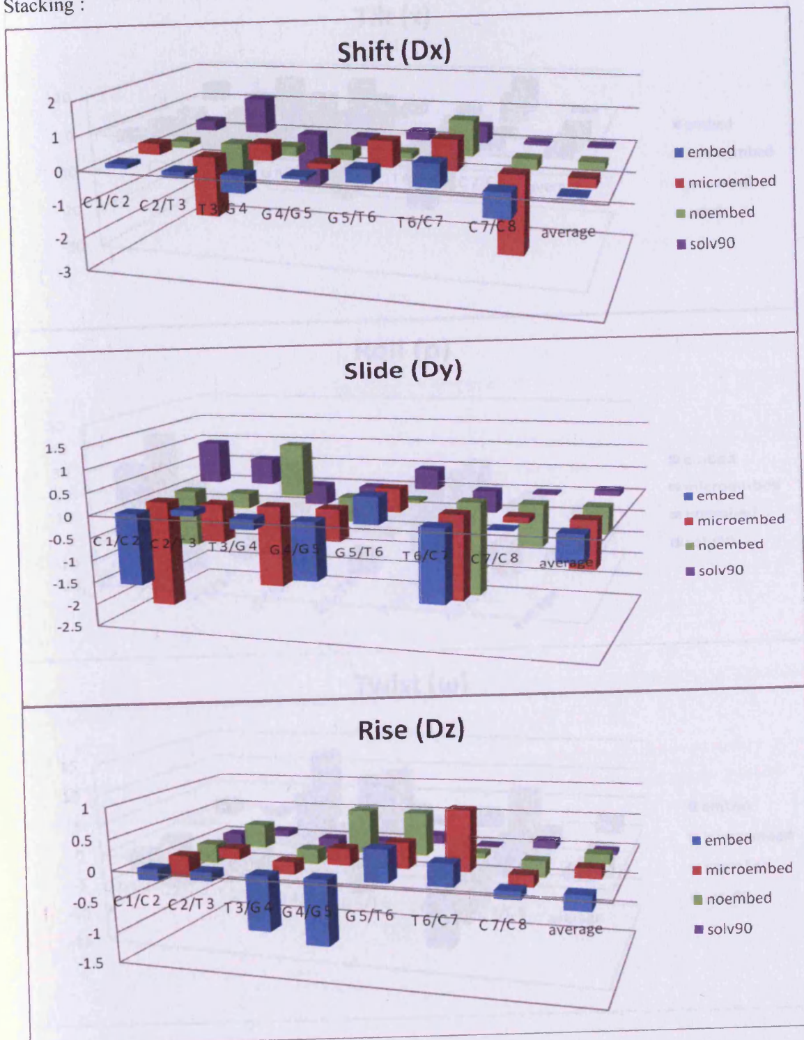
Figure 3.4.19: Changes in lattice parameters for stacked bases compared to 3D lattice structure
