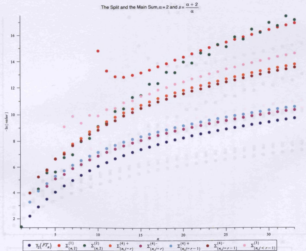
FIGURE 3.4. The partition -\log(\cdot) -scale. \alpha = 2 and s = \frac{\alpha+2}{\alpha}
