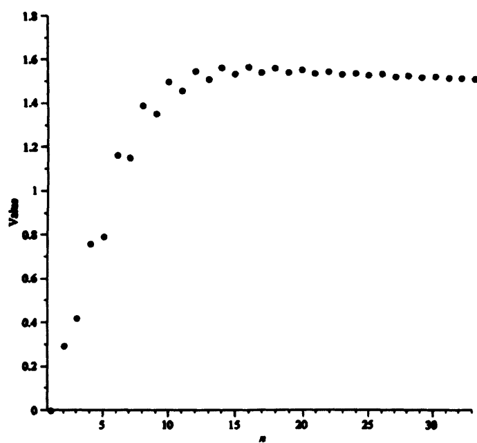
(b) Values of n^{\alpha+2}\Sigma_{(n,j=r-1)}^{(4)-} , \alpha = 2
