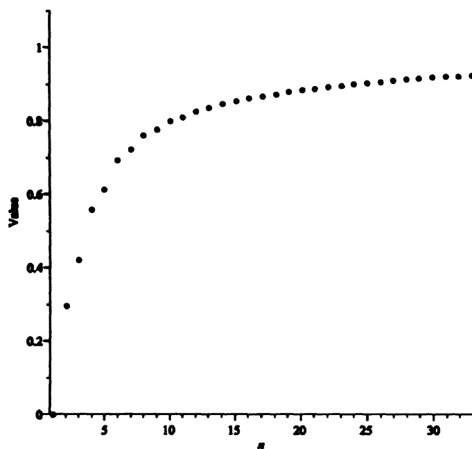
(a) Values of n^{\alpha+1}\Sigma_{(n,j=r-1)}^{(4)+} , \alpha = 2
