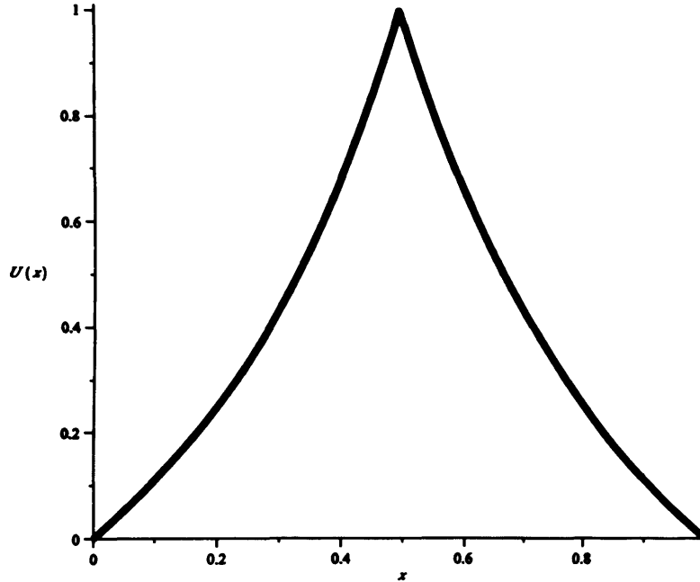
FIGURE 1.3. The Farey Map
