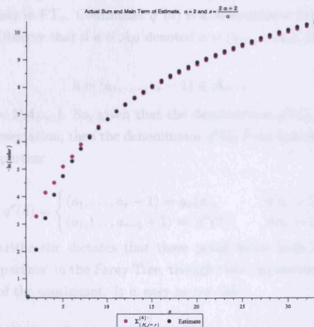
(b) \Sigma_{(N,j=r)}^{(4)-} with Main Term, s = \frac{2\alpha+2}{\alpha}
