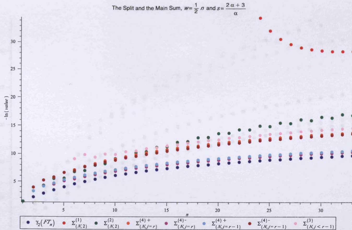
FIGURE B.12. The partition, -\log(\cdot) -scale. \alpha = 2 and s = \frac{2\alpha+3}{\alpha}
