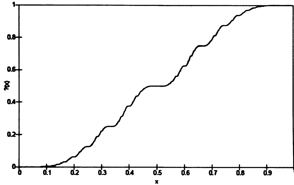
FIGURE 1.6. Minkowski ?-Function
