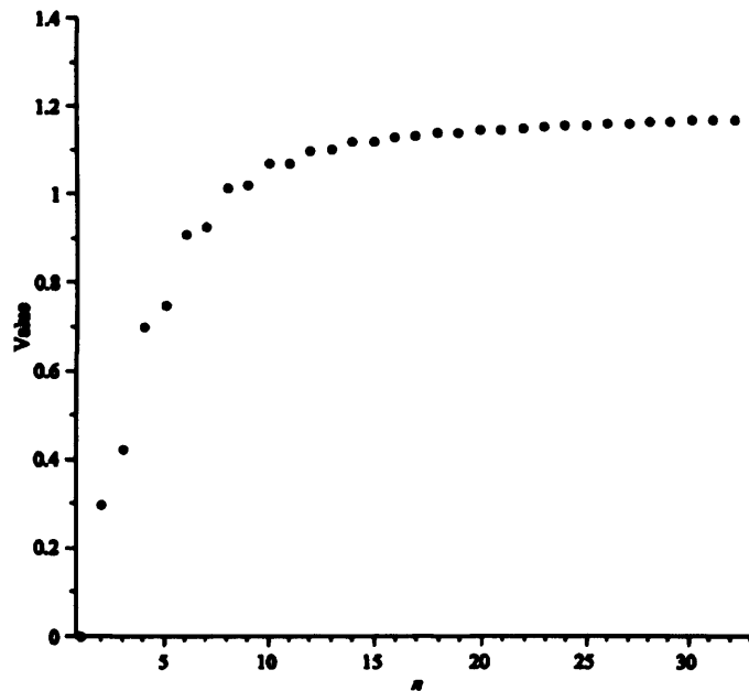
(b) Values of n^{\alpha+1}\Sigma_{(n,j=r)}^{(4)-} , \alpha = 2
