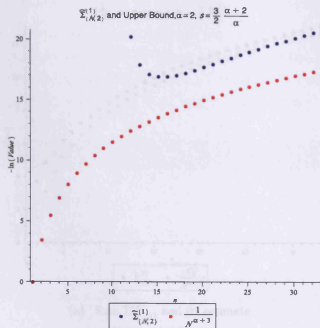
(a) Sum \tilde{\Sigma}_{(N,2)}^{(1)} and its upper bound
