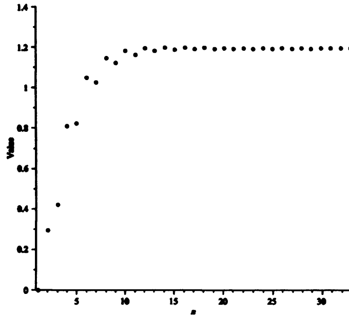
(a) Values of n^{\alpha+2}\Sigma_{(n,j=r)}^{(4)+} , \alpha = 2
