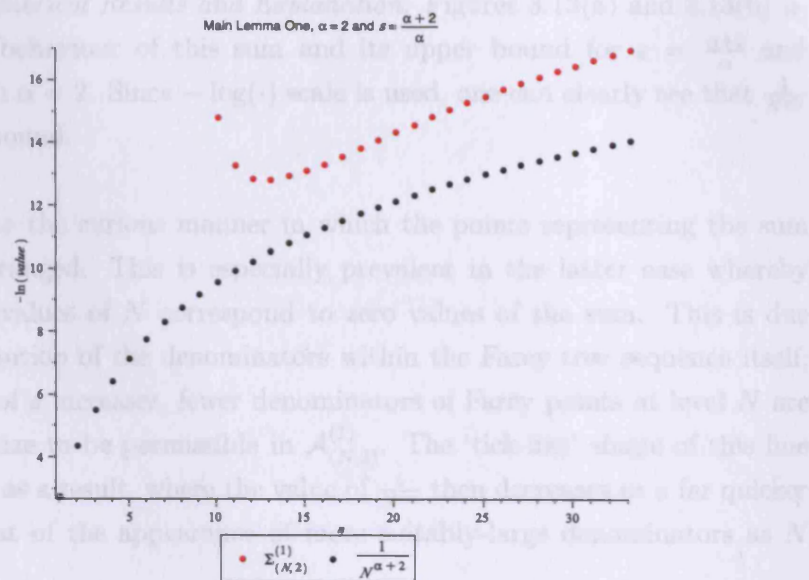
(a) \Sigma_{(N,2)}^{(1)} and upper bound, for s = \frac{\alpha+2}{\alpha}
