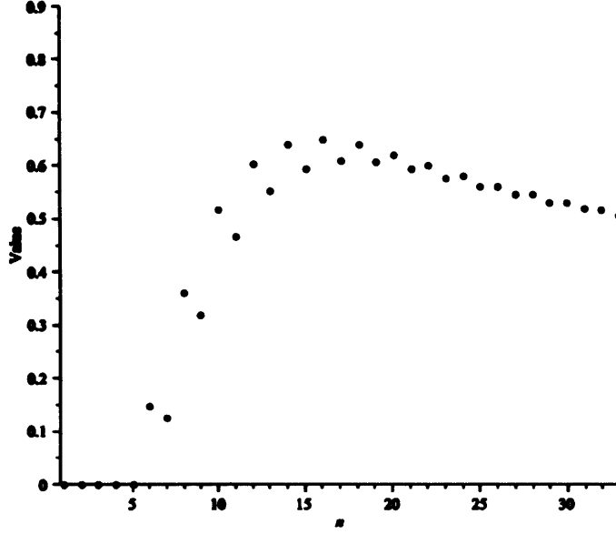
FIGURE 3.9. Values of n^{\alpha+2}\Sigma_{(n,j<r)}^{(3)} , \alpha = 2
