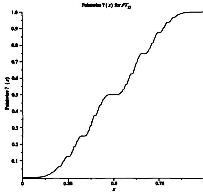
FIGURE 1.5. Pointwise Minkowski \gamma -Functions for n = 4 and n = 13
