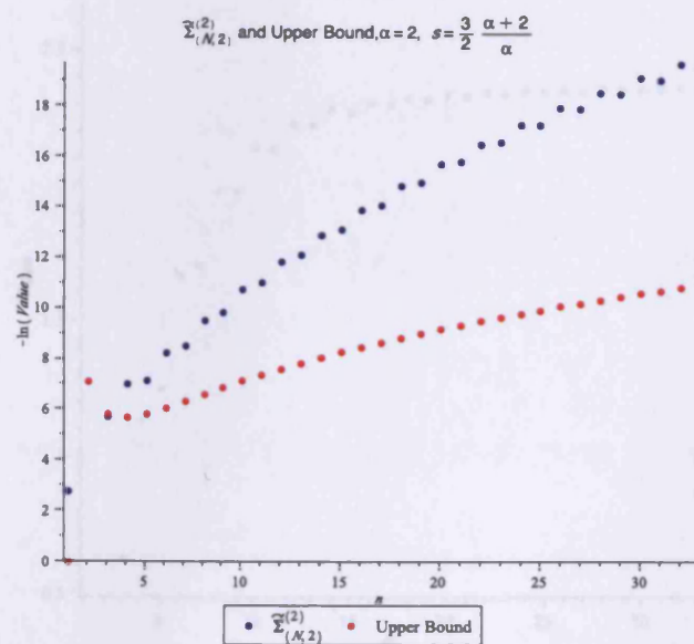
(b) Sum \tilde{\Sigma}_{(N,2)}^{(2)} and its upper bound
