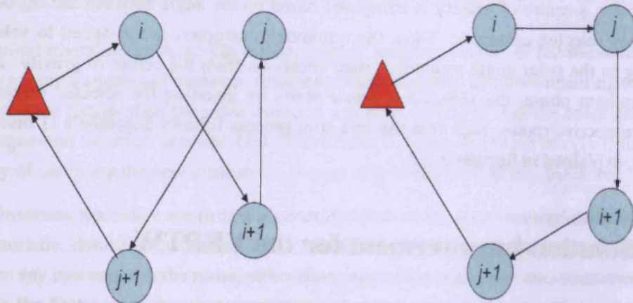
Figure 3.7: 2-exchange move.
