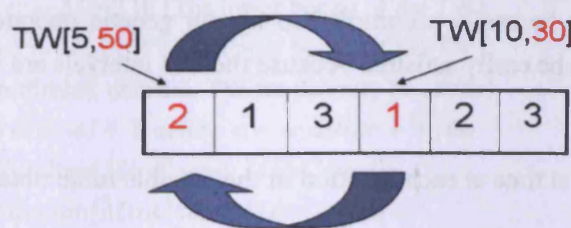
Figure 5.6: Directed Mutation.
