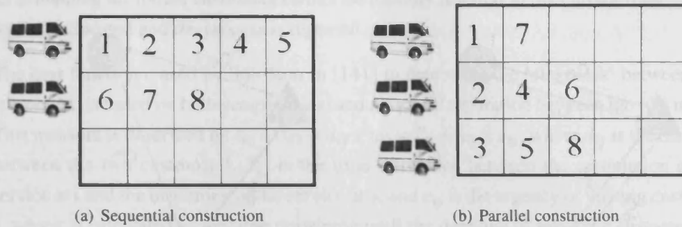
Figure 3.4: Solution Construction.
