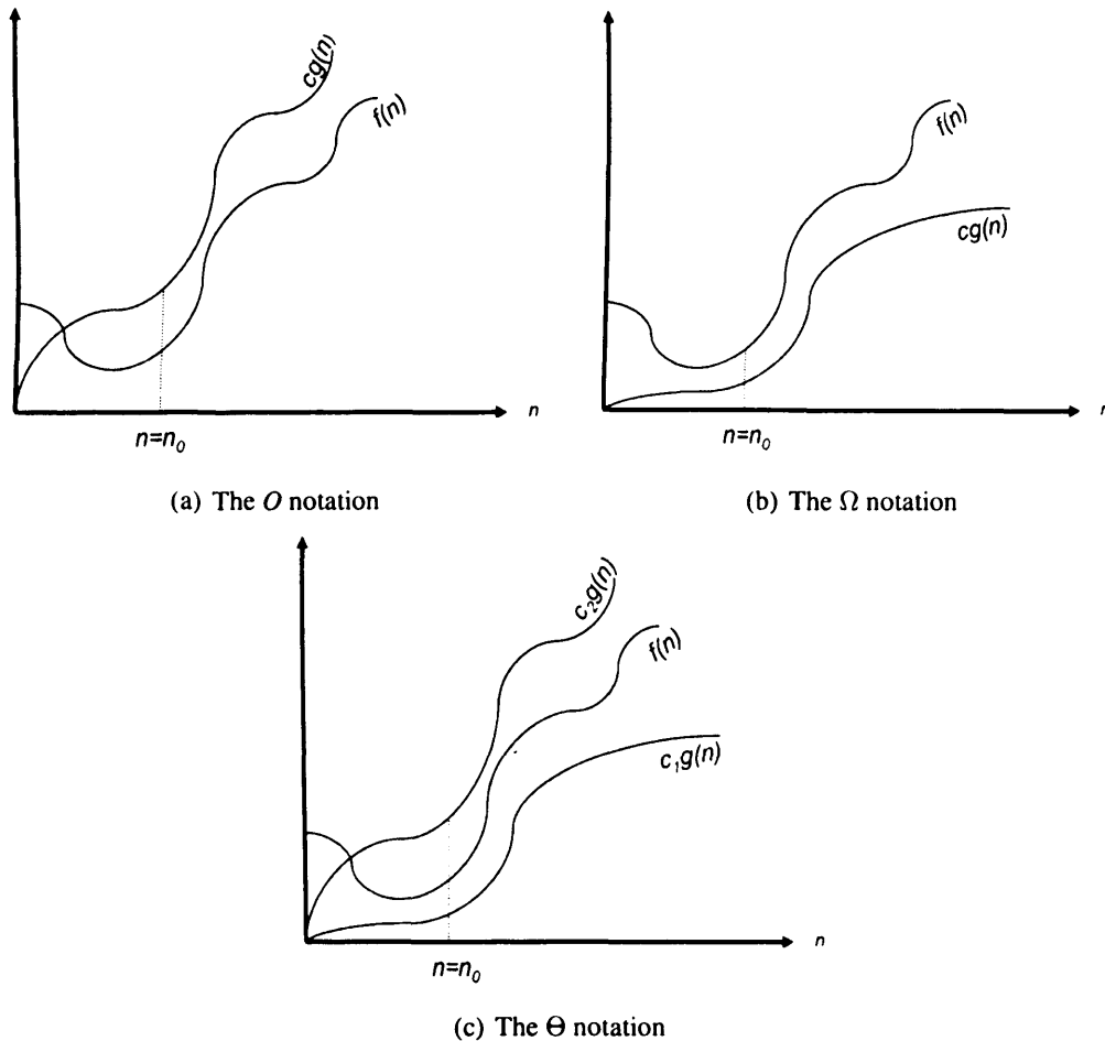
Figure 2.1: Asymptotic Notations.
