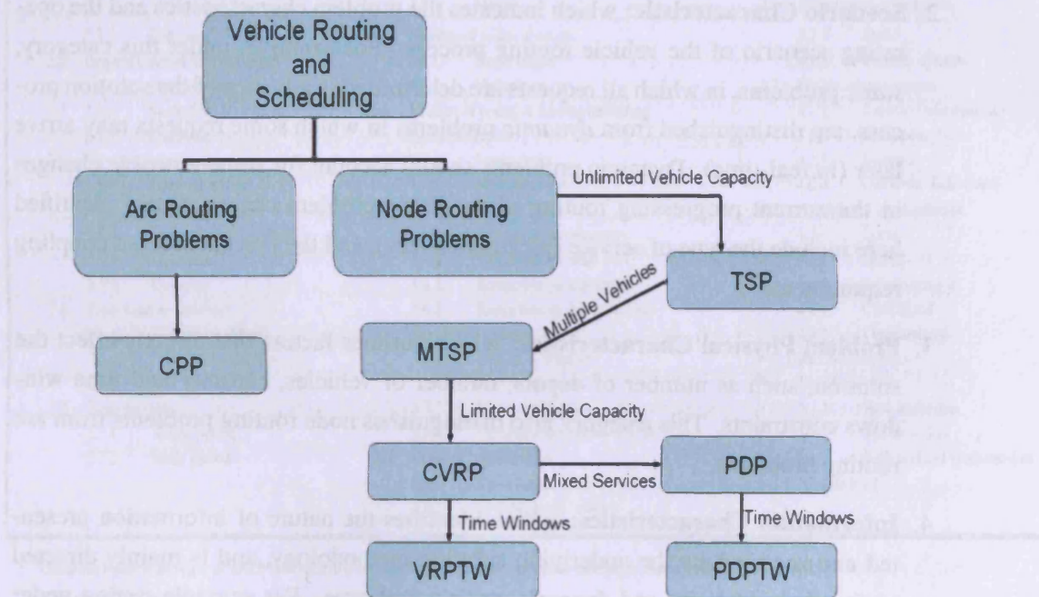
Figure 3.1: Vehicle routing and scheduling problems.
