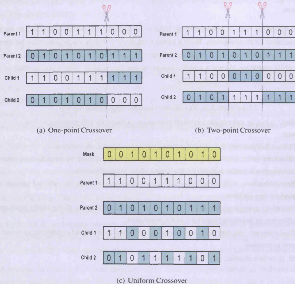
Figure 2.6: Crossover.
