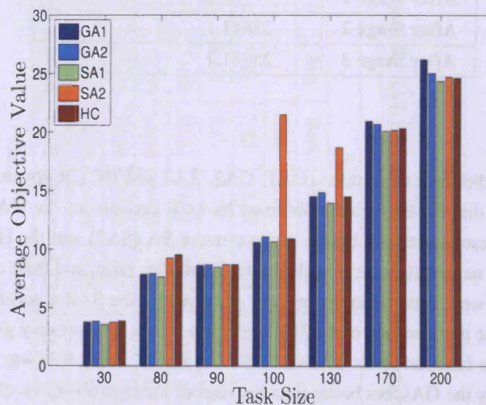
Figure 6.1: Average objective value for all algorithms.
