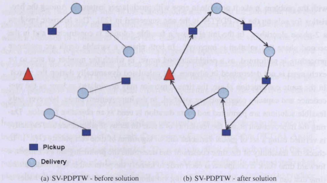
Figure 5.1: The single vehicle pickup and delivery problem with time windows.
