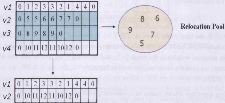
(a) VMM - two vehicles selected for merging, and their request placed in the relocation pool. Remaining routes copied to the new solution without change
