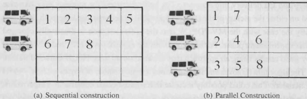
Figure 7.2: Solution Construction.
