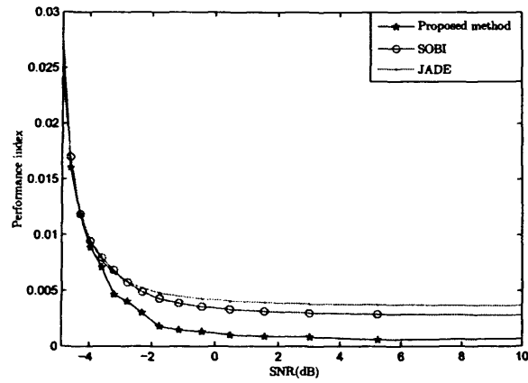
Figure 5.3: Performance comparison of the proposed method, SOBI and JADE algorithms for different levels of noise.
