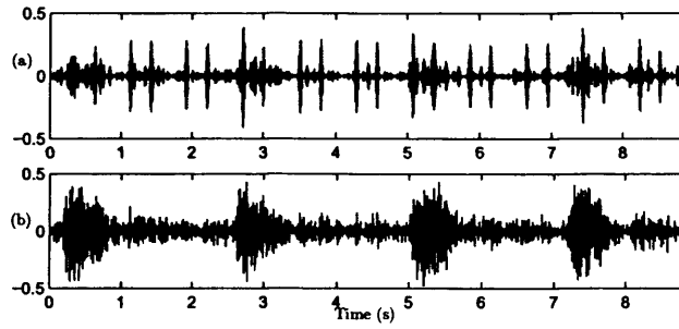
Figure 4.3: Result of SSA applied to the signal of Fig. 4.1.(c); (a) reconstructed signal using the first six eigentriples and (b) the remaining signal.
