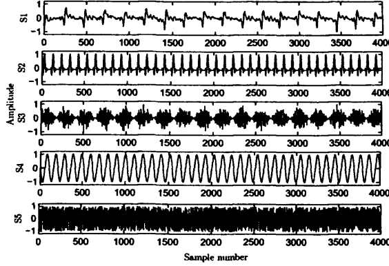
Figure 6.1: Five signals are synthetically mixed to evaluate the performance of the proposed method. S1 and S3 have a common cycle frequency.
