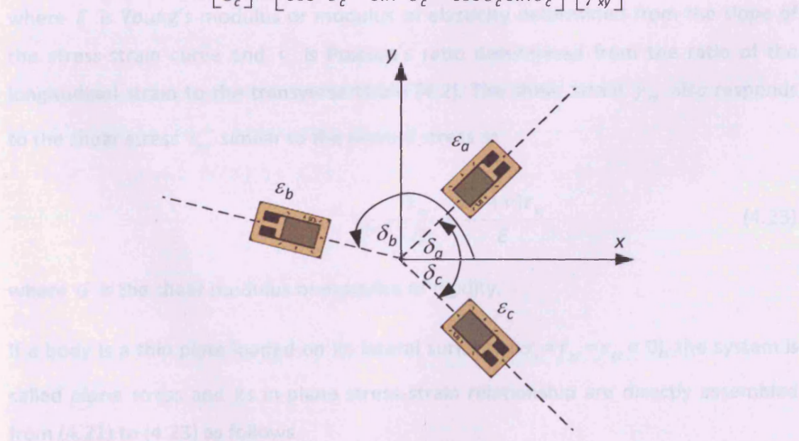
Fig. 4-5 Rosette strain gauge arrangement for measurement of components of in-plane strains
