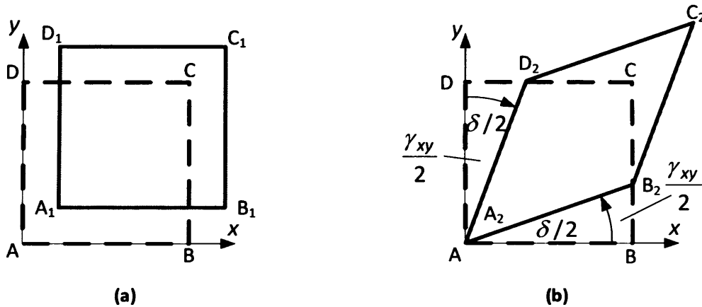
Fig. 4-3 Illustration of (a) normal strain and (b) shear strain for an infinitesimal element in two dimensions
