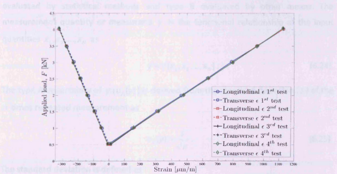
Fig. 6-21 Applied load versus longitudinal and lateral strains of an Epstein strips cut along the RD
