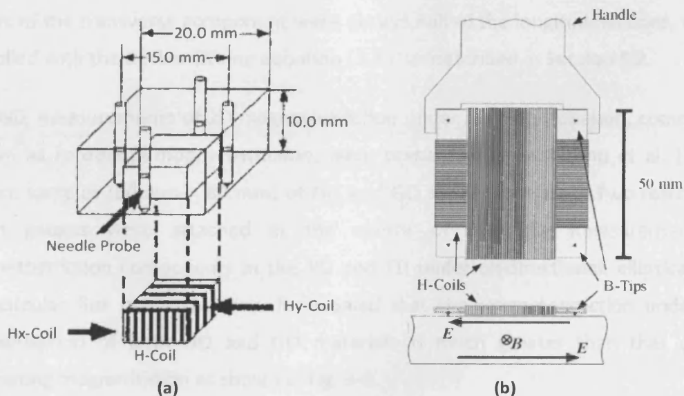
Fig. 3-2 Localised magnetic sensors based on orthogonal needle probes and h coils developed by: a) Enokizono et al [3.3], b) Krismanić et al. [3.5].
