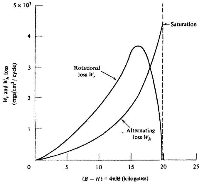
Fig. 2-10 Loss of a 3.13 % SiFe GO steel under rotational and alternating magnetisation at quasi static magnetising frequency (magnetisation of 1 kilogauss = 0.1 T and loss per unit volume of 1 \text{erg/cm}^3 = 0.1 \text{ J/m}^3 ) [2.2]
