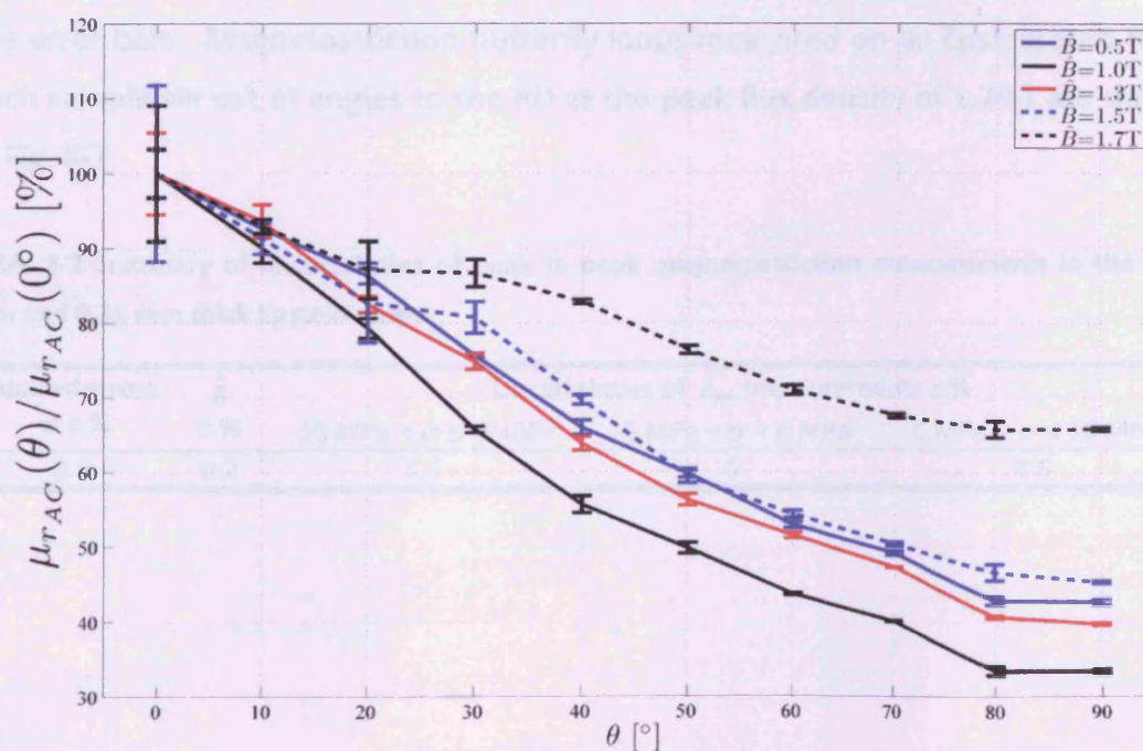
Fig. 8-4 Percentage variation of the AC relative permeability in the Epstein strips of the 0.50 mm thick steel cut at angles \theta relative to that in the sample set cut along the RD at various flux densities
