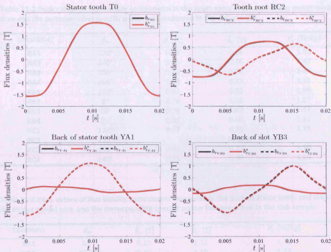
Fig. 11-7 Comparisons of the radial and tangential flux density components of the stator tooth T0, tooth root RC2, back of the stator tooth YA1, and back of the slot YB3, measured in the motor model core and simulated in the 0.50 mm thick disc sample (The symbol * denotes the simulated waveforms in the 2D magnetisation system)
