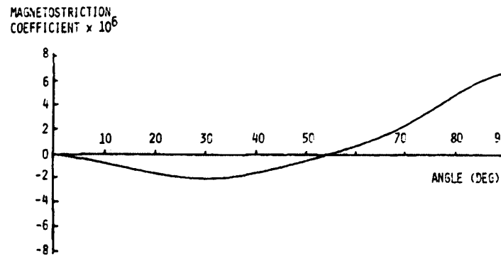
Fig. 3-6 Experimental magnetostriction coefficient of GO steel at angles to the RD [3.28]
