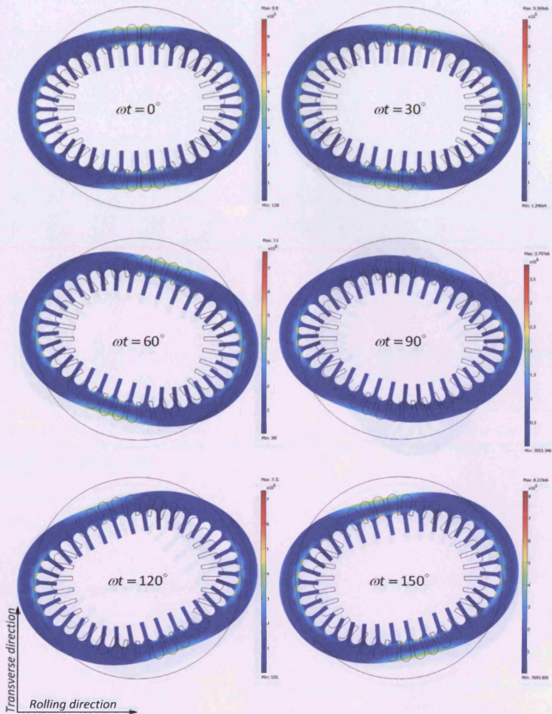
Fig. 11-13 Simulated core deformation due to the magnetostrictive-profiled stresses \sigma_{Tn}^\lambda at the time instances \omega t = 0^\circ, 30^\circ, 60^\circ, 90^\circ, 120^\circ and 150^\circ . The colour bars indicate the von Mises (scalar) stress.
