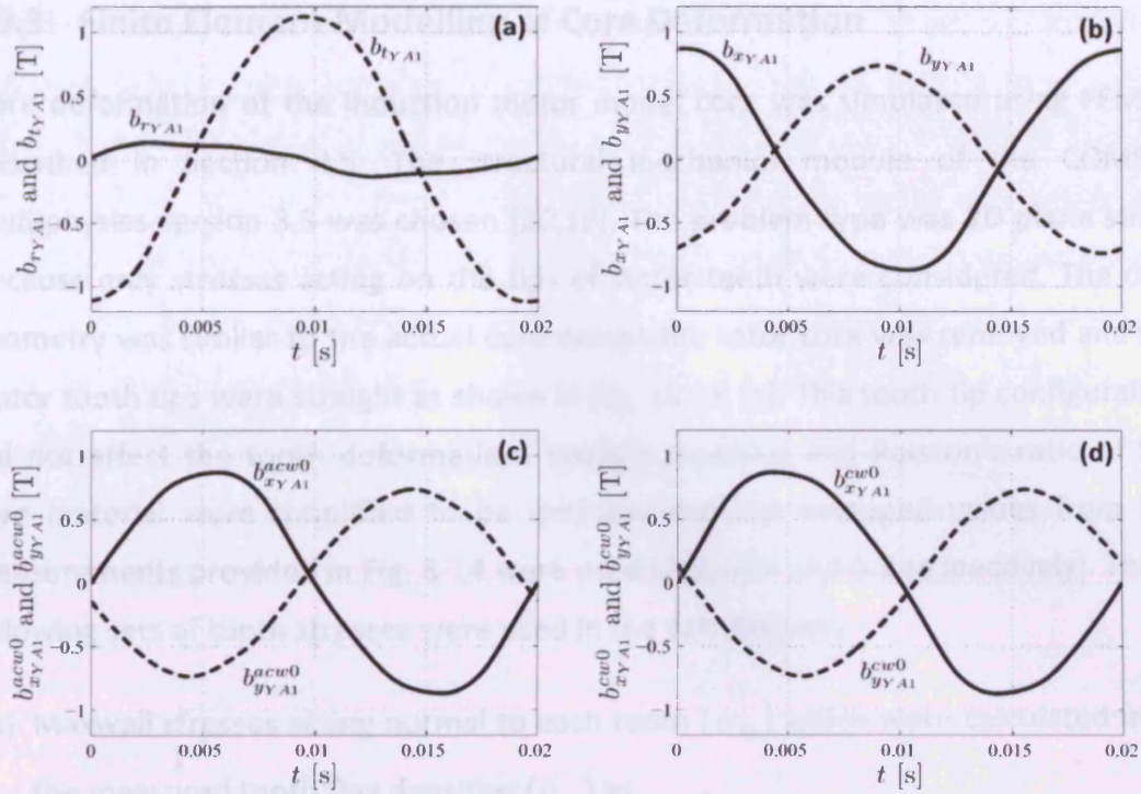
Fig. 10-14 Components of flux density at point YA1 of the induction motor model core: (a) radial and tangential components, (b) components in the RD and TD ( b_{xYA1} and b_{yYA1} ), (c) shifted b_{xYA1} and b_{yYA1} , and (d) reversed and shifted b_{xYA1} and b_{yYA1} . Note that (c) and (d) were used as the reference signals of the 2D magnetisation system in the ACW and CW field rotation directions.
