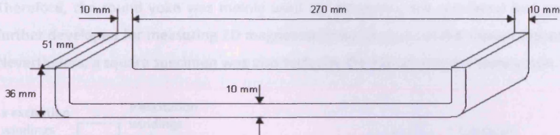
Fig. 6-6 Physical dimensions of the flux closure yoke of the AC magnetostriction measurement system [6.4]
