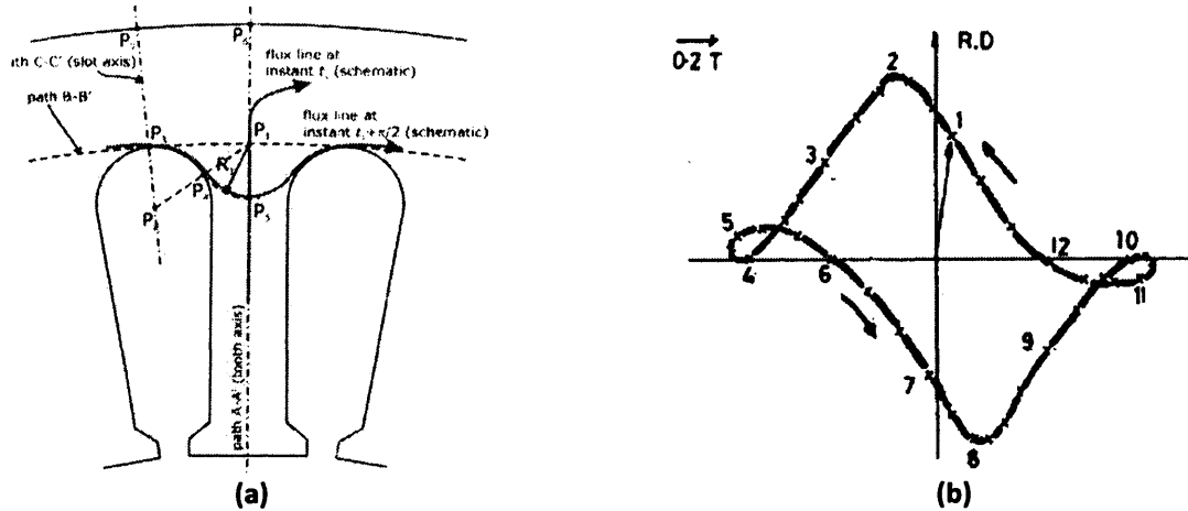
Fig. 2-8 (a) Illustration of a flux line at time instant t_1 and t_1 + \pi/2 in an induction motor stator core [2.13], (b) Magnitude and direction of flux density at the T joint of a three-phase transformer core at 30° intervals in time [2.14]
