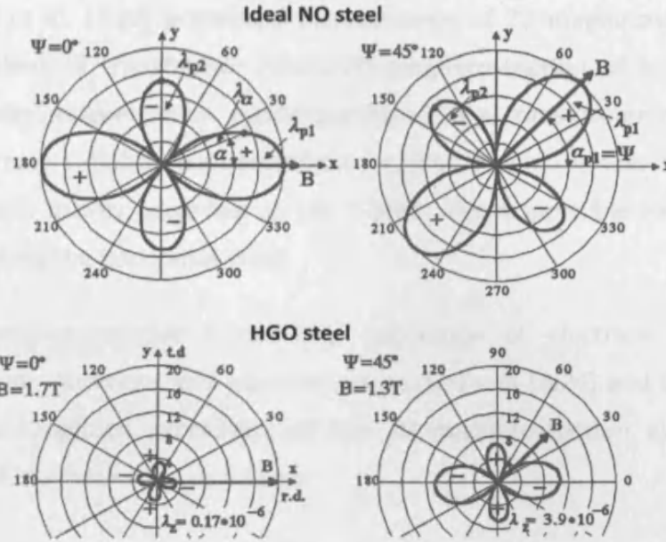
Fig. 3-4 Polar plots of magnetostriction of ideal NO and HGO steels when the magnetisation vector at 0^\circ and 45^\circ to the RD [3.17], where the plus (+) and minus (-) denote positive and negative magnetostriction respectively.
