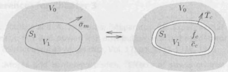
Fig. 3-10 Definition of the long-range magnetic forces [3.55]
