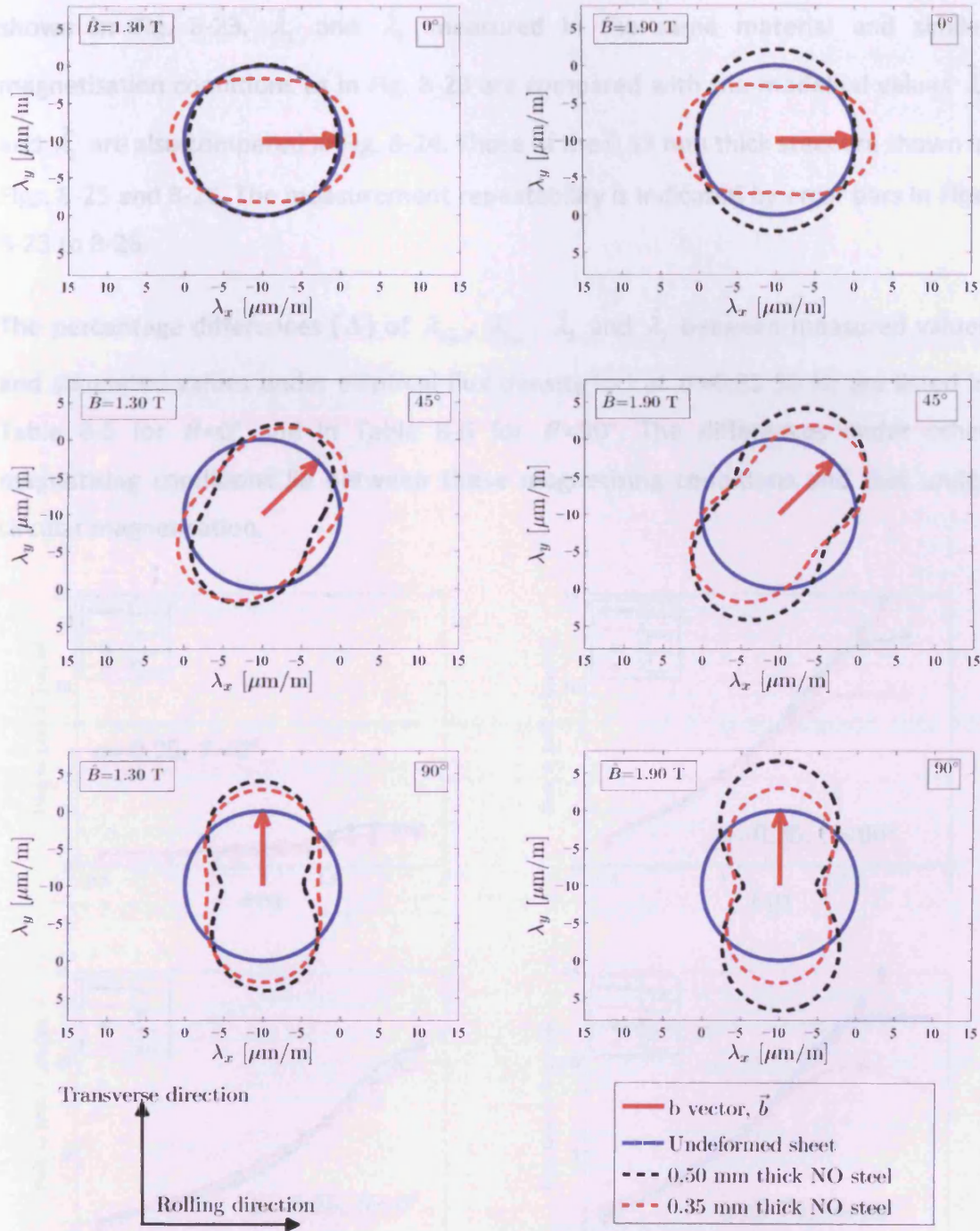
Fig. 8-22 In-plane deformation plots of the 0.50 mm and 0.35 mm thick steels under circular magnetisation at 1.30 and 1.90 T, 50 Hz and \vec{b} vector ( \vec{b} ) at 0°, 45° and 90° with respect to the RD
