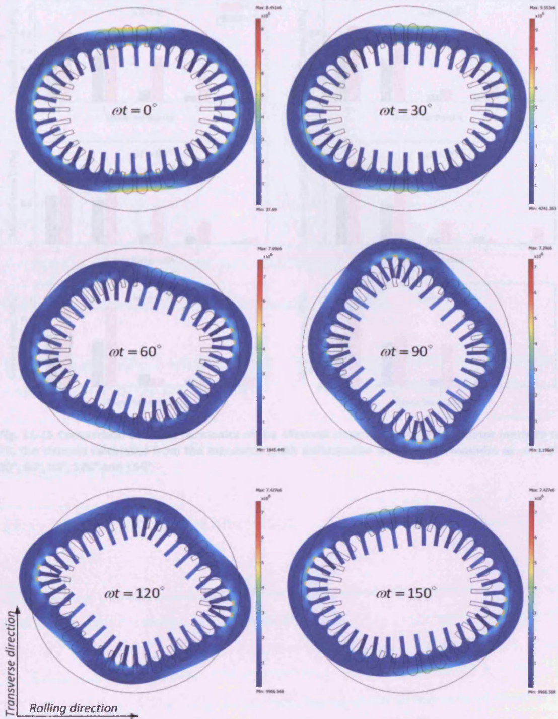
Fig. 11-14 Simulated core deformation due to the combination of Maxwell stresses and magnetostriction ( \sigma_{T_m}^e ) at the time instances \omega t = 0^\circ, 30^\circ, 60^\circ, 90^\circ, 120^\circ and 150^\circ . The colour bars indicate the von Mises (scalar) stress.
