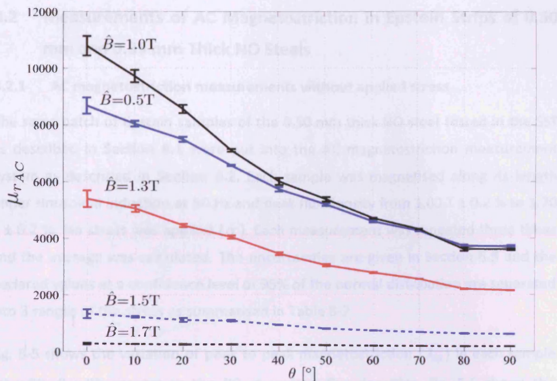
Fig. 8-3 Averaged values of the AC relative permeability in the Epstein samples of the 0.50 mm thick steel cut at angles \theta with respect to the RD at various flux densities
