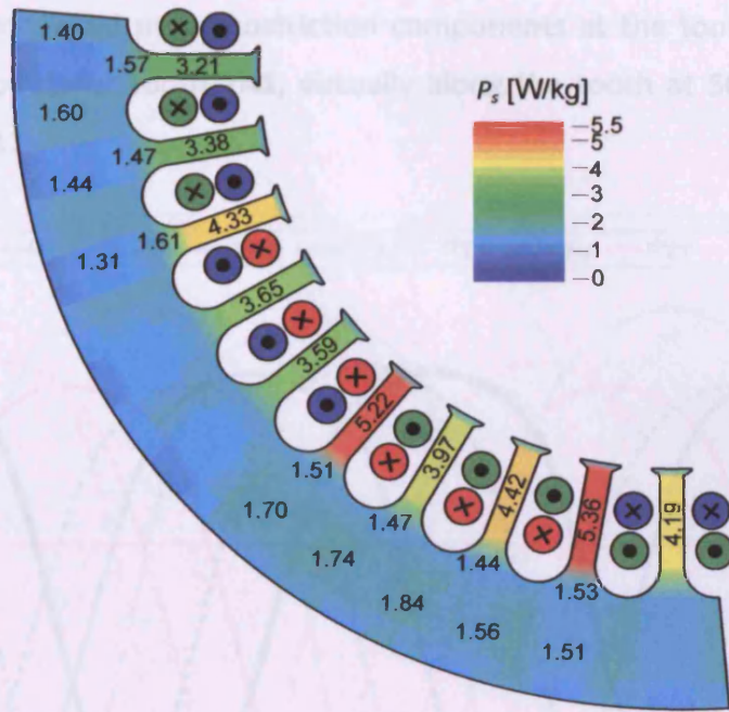
Fig. 11-8 Distribution of specific power loss in a section of the motor model core obtained from simulations in the disc sample under localised magnetisation conditions in the core
