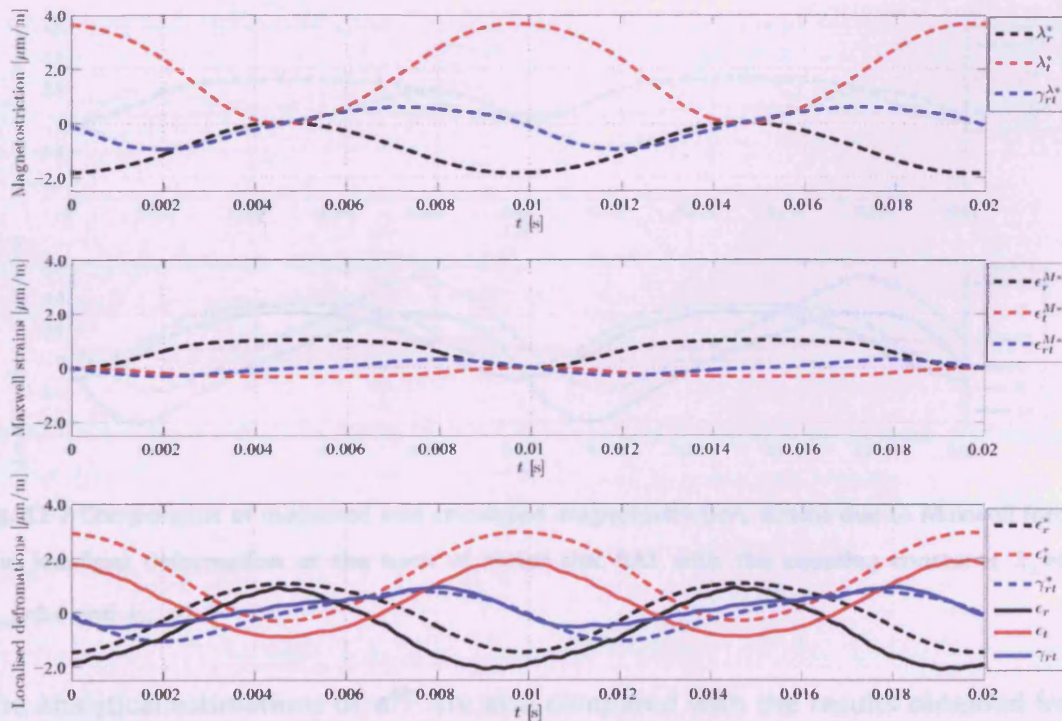
Fig. 12-6 Components of calculated magnetostriction ( P_x = P_y = P = 136 GPa, \xi_x = \xi_y = \xi = 0.5 , and D = P/(2(1 + \xi)) ), strains due to Maxwell forces, and localised deformation at the back of stator tooth YA1 with the coupling constants k_\lambda=0.8 and k_M=0.2
