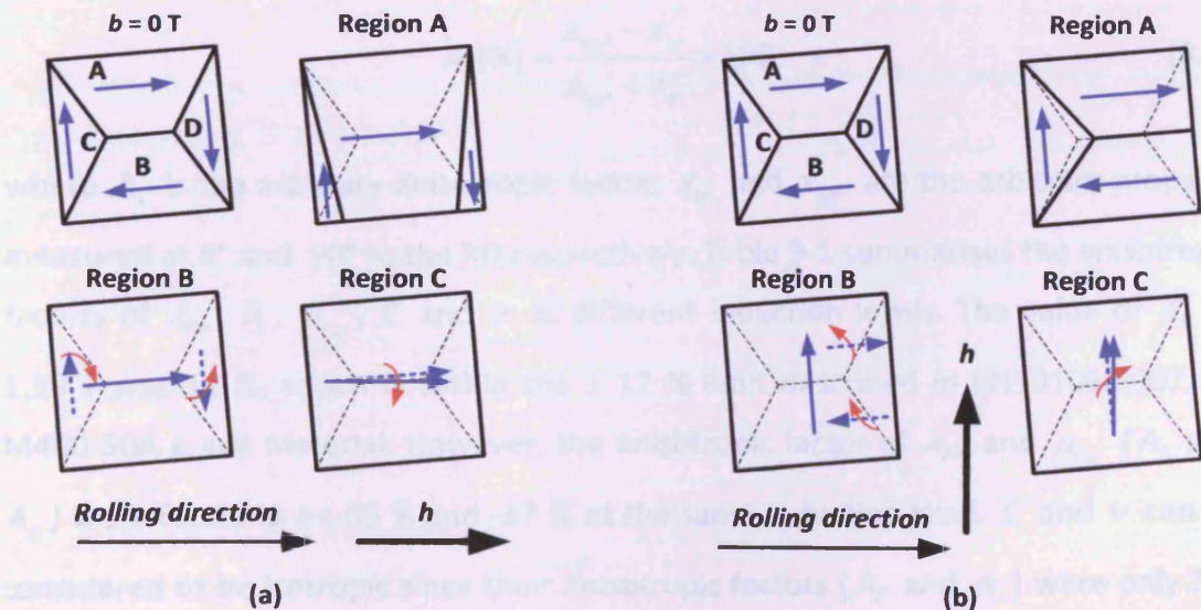
Fig. 9-3 Schematic diagram of the domain model of the 0.50 mm NO steel in different regions of magnetisation (referred to Fig. 9-1): (a) magnetised along the RD, (b) magnetised perpendicular to the RD.
