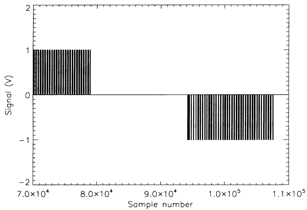
Figure 4.3: Nodding structure for the Mars file 060205.ob7. The nodding sequence is clearly different to the typical structure.
