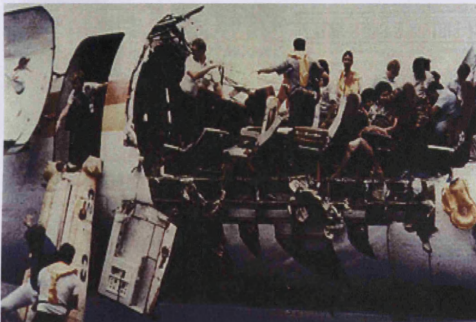
Figure 1.7 Aloha Airlines Structural Fuselage Failing
