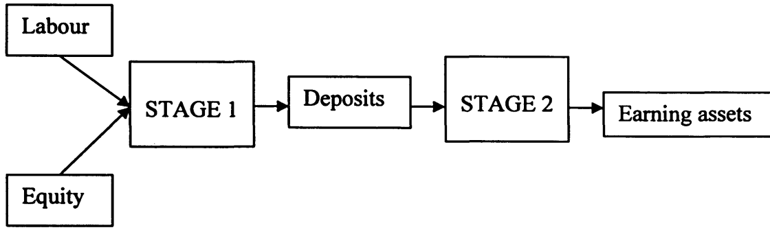
Figure 3.4 Network DEA Serial Process
