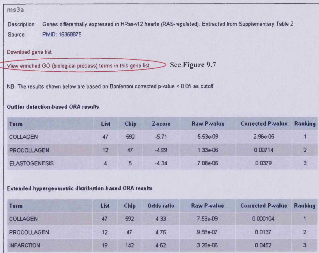
Figure 9.6: Screenshot from PAKORA showing the text-based ORA results for a literature gene list derived from the mouse MG-U430 2.0 array
