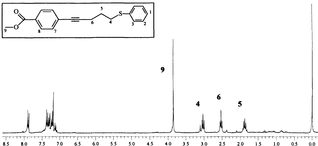
Figure 6 1 H-NMR spectrum (400 MHz, CDCl 3 ) of 29
