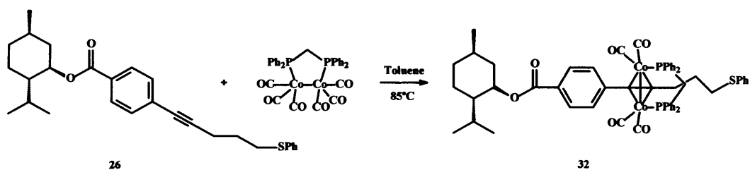
Scheme 19 Synthesis of 32
