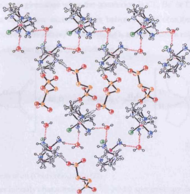
Figure 31 Crystal packing of 20 along the b-axis, with cationic units linked by hydrogen bonding water (red) and cationic units linked by tetrathionate counterions (black)
