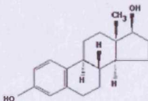
Figure 1.2 Chemical structure of 17- \beta oestradiol
