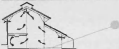
Figure 5 & 6: 'Seasonal hybrid' ventilation system at Trinity College Library, Carmarthen
