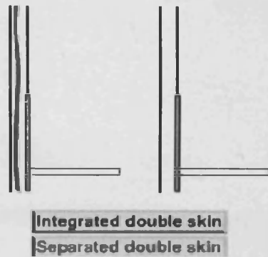
Figure 10: Integrated and separated double skin ventilation systems Click to view illustrations
