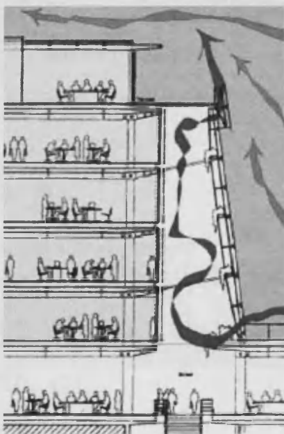
Figure 1: Analysis of wind driven ventilation in an atrium. .
