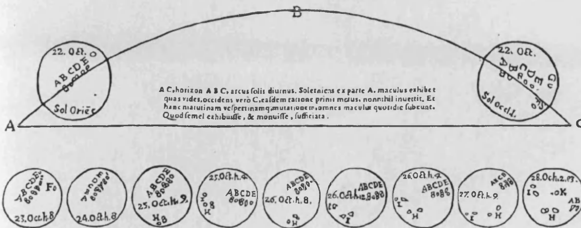
Illustrations from Galileo's Three Letters on Sunspots (1613), reporting the sunspots of October 1611. Small multiples record the movement of sunspots on the surface of the sun.
