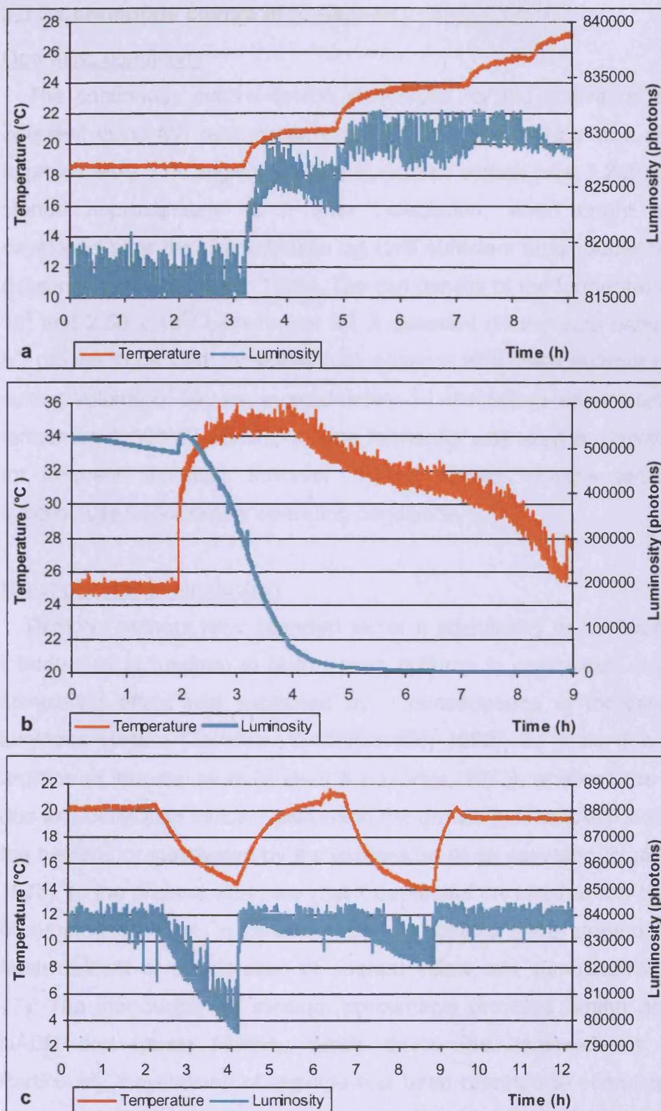
Figure 46 Influence of temperature variations in continuous cultivation of V. fischeri . Small increases in temperature between 18 and 24°C resulted in increased bioluminescence. Above 24°C bioluminescence decreased (a). Large increase in temperature above 25°C resulted in large decrease in bioluminescence (b). Decreases in bioluminescence could be restored with the restoration of favourable temperature conditions. The temperature variations were achieved by placing the fermenter inside an incubator.
