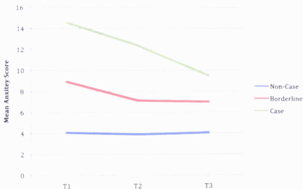
Fig 4.2. Graphical display of trends over time for anxiety (n=110).
