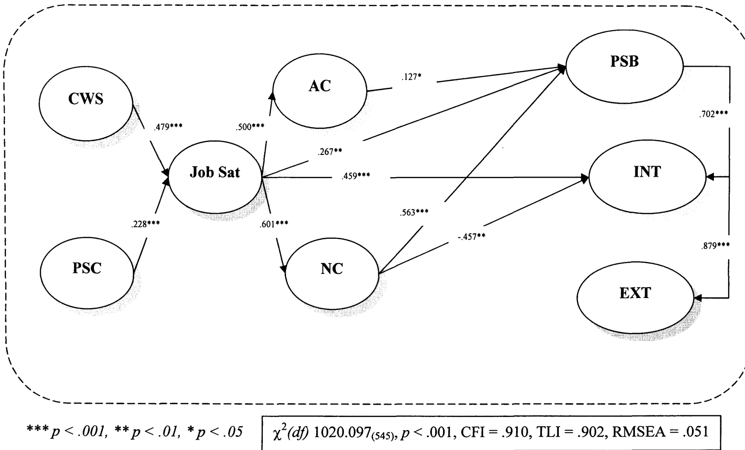
Figure 9.2: The trimmed model and the parameter estimates
