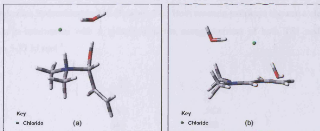
(a) Optimised geometry of aminol and (b) iminium ion product.
