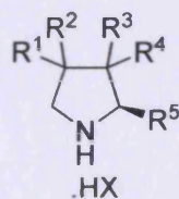
Pyrrolidine architecture
