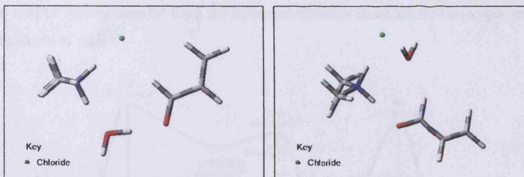
Two possible reaction geometries.
