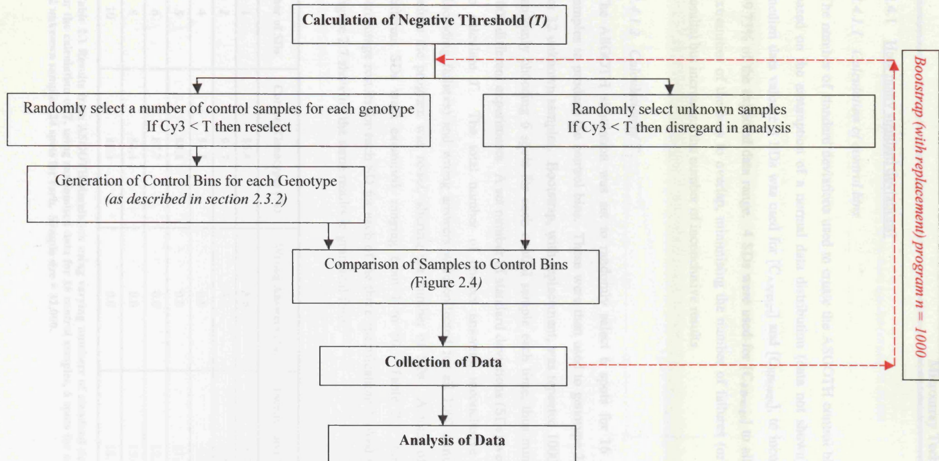
Figure 2.6 Flow diagram depicting the path of the validation bootstrapping program. Samples are randomly selected (with replacement) and the program was repeated 1000 times.
