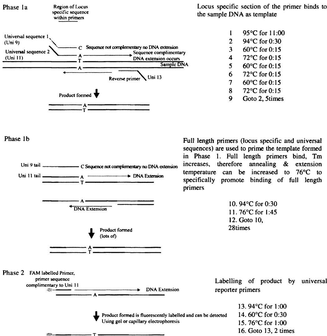
Fig. 1. Diagrammatical representation of the URP/ARMS Principle. The amplification technique has two distinct phases: phase 1a uses the locus-specific portion of the ~40-mer primers to provide sufficient template with Universal tails for amplification in phase 2. The increase in T_m observed in phase 1b allows the whole length of the long primers to bind to the template, dependent on the Universal tail present. By phase 2, all long primers have been exhausted and the annealing temperature is reduced to allow the 20-mer fluorescently labelled Universal primers to anneal and extend.
