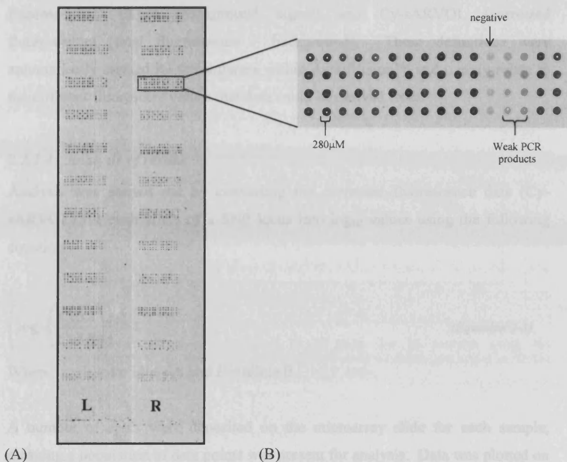
Figure 2.1 Cy3 fluorescent images of a post-spotted, hybridised glass slide derived from ImageQuant™. (A) = duplicated spots (L & R) in 12 separate blocks, each block being spotted by a different pen from the 12-pen set. (B) = one block enlarged to show the individual spots, each one indicating a single PCR product.
